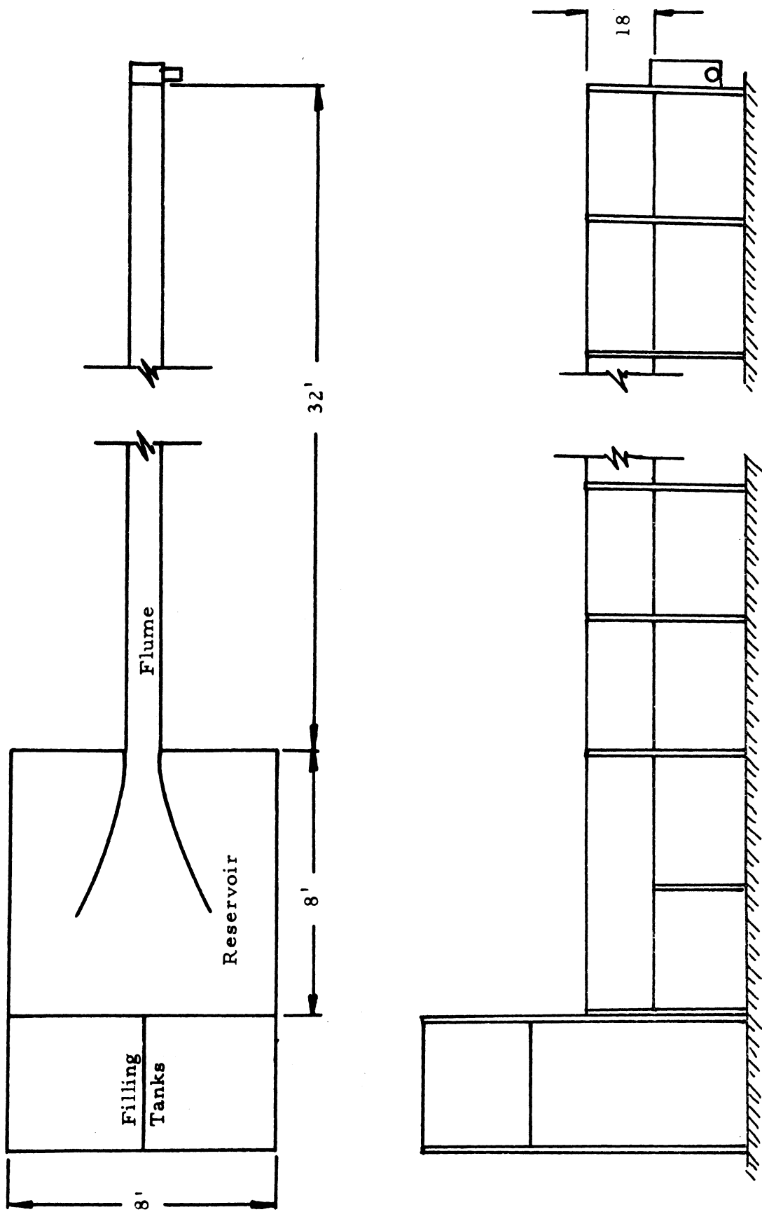
Flume-Reservoir System
