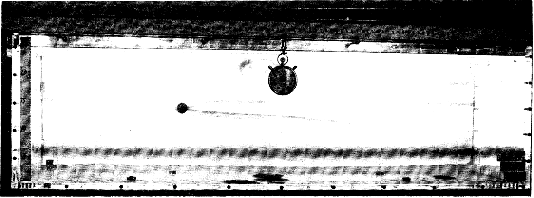
Fig. 3 a. Translating cylinder ( \mathbb{R} = 11 , \mathbb{F}_d = 0.0455 ) with a following fluid train.
