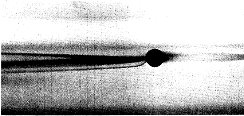
Fig. 4 a. Elongated, stable vortex pair upstream of cylinder which is moving to the right. Downstream pattern, a wedge formation, is associated with downstream blocking. \mathbb{R} = 18 and \mathbb{F}_d = 0.072 in this experiment appear to be marginal for downstream blocking.
