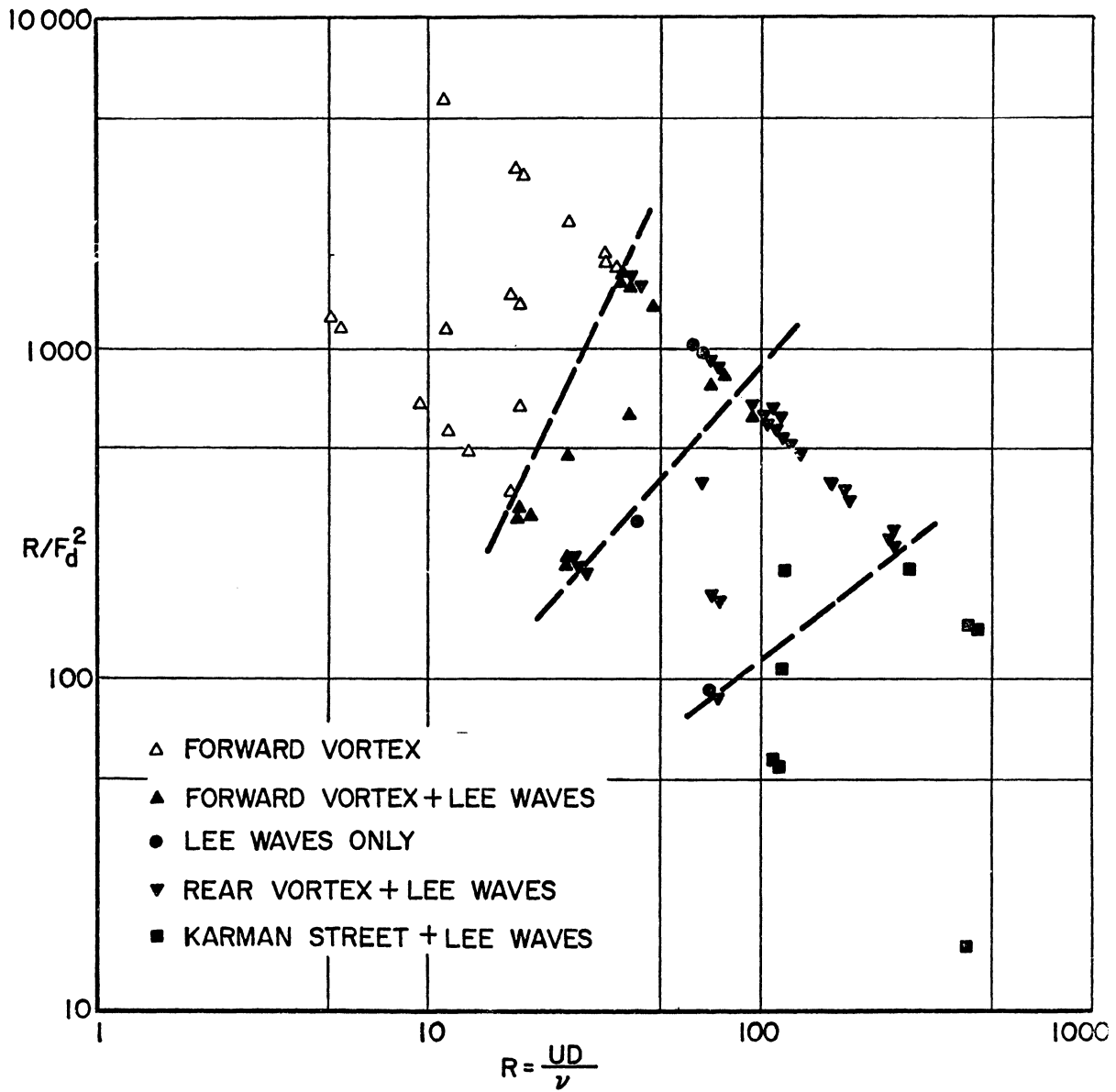
Fig. 6 Flow phenomena diagram for two dimensional circular cylinder translating in a stratified fluid. Vertical coordinate is ratio of the buoyant and viscous forces.
