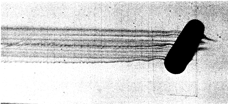
Fig. 4 c. View of dye from cylinder moving ahead of cylinder to delineate ultimately a vortex pair \mathbb{R} = 40 and \mathbb{F}_d = 0.16 .
