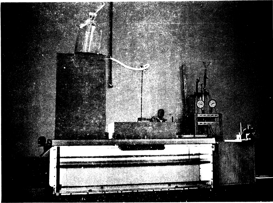
Fig. 1 a. Side view of towing tank, drive and filling appurtenances.
