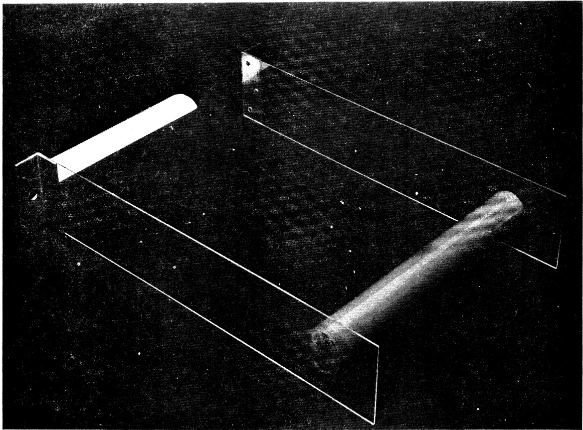
Fig. 2 a. Cylinder and support struts.
