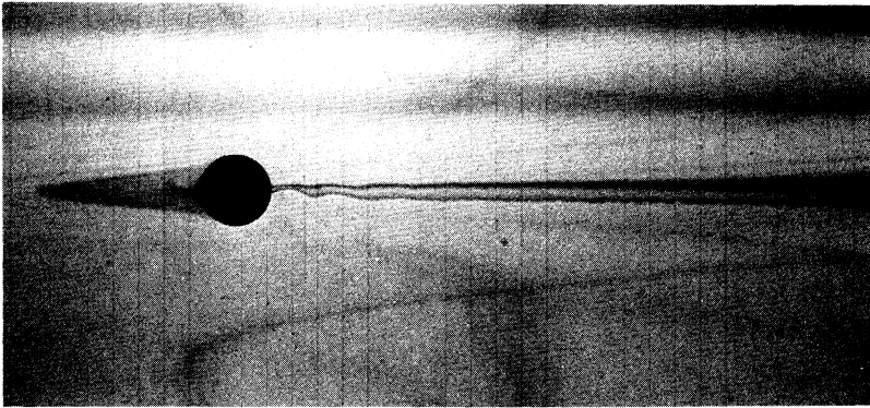
Fig. 4 b. Upstream vortices without downstream blocking. Horizontal lines at the right caused by dye coming from cylinder. Lower line due to gradual sinking of dye. No significant lee waves present. Symmetric structure of upstream vortices indicated. \mathbb{R} = 47 and \mathbb{F}_d = 0.188 .
