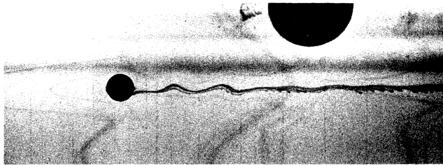
Fig. 5 b. Cylinder free of upstream and downstream vortices. Lee waves present. \mathbb{R} = 62 and \mathbb{F}_d = 0.248 .
