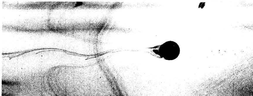
Fig. 5 c. Cylinder with attached, stable, downstream vortices with lee waves. \mathbb{R} = 160 and \mathbb{F}_d = 0.641 .
