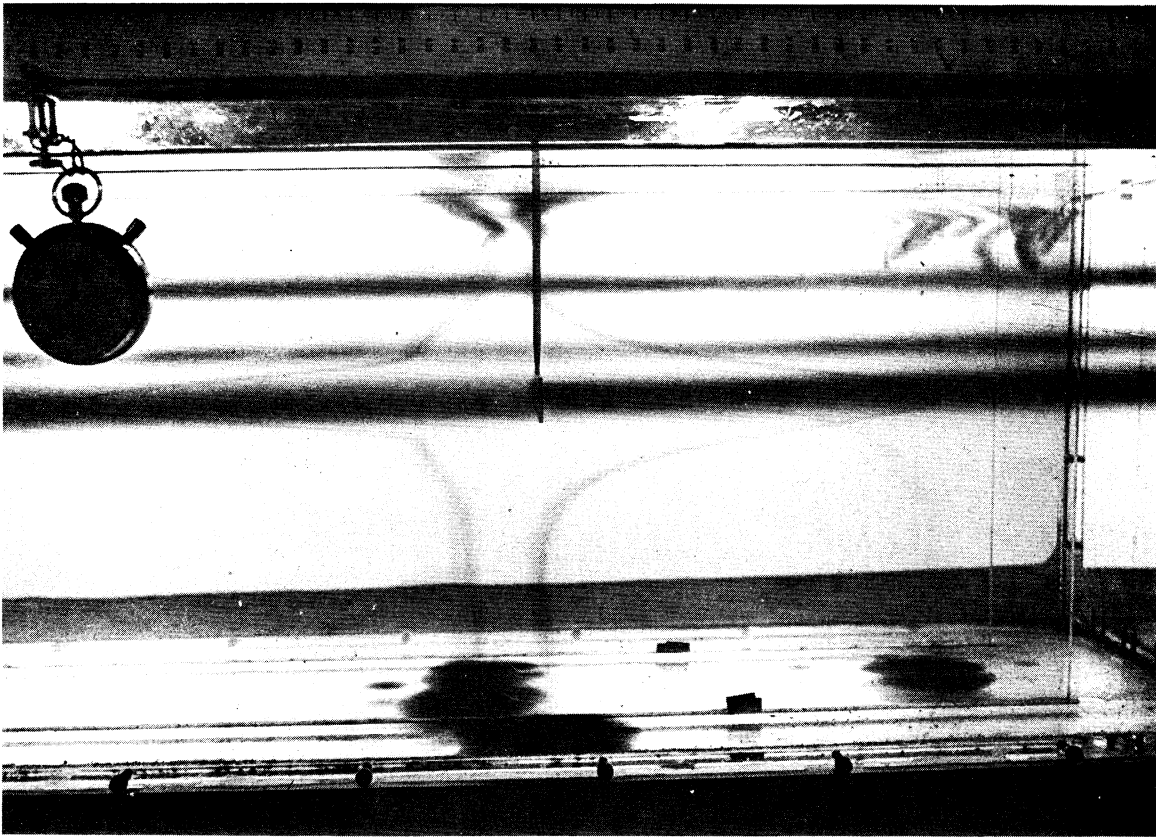
Fig. 7. Vertical plate moving toward the left. \mathbb{R} = 93 and \mathbb{F}_d = 0.037 . Dye sheets in central channel show upstream and downstream blocking.
