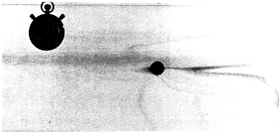
Fig. 3 c. Same cylinder 15 minutes after starting. Fluid which was originally behind cylinder (i. e. to the right of horizontal wedge) is being left behind.
