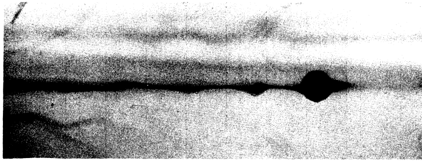
Fig. 5 a. Upstream vortices and small lee waves. \mathbb{R} = 77 and \mathbb{F}_d = 0.31 .
