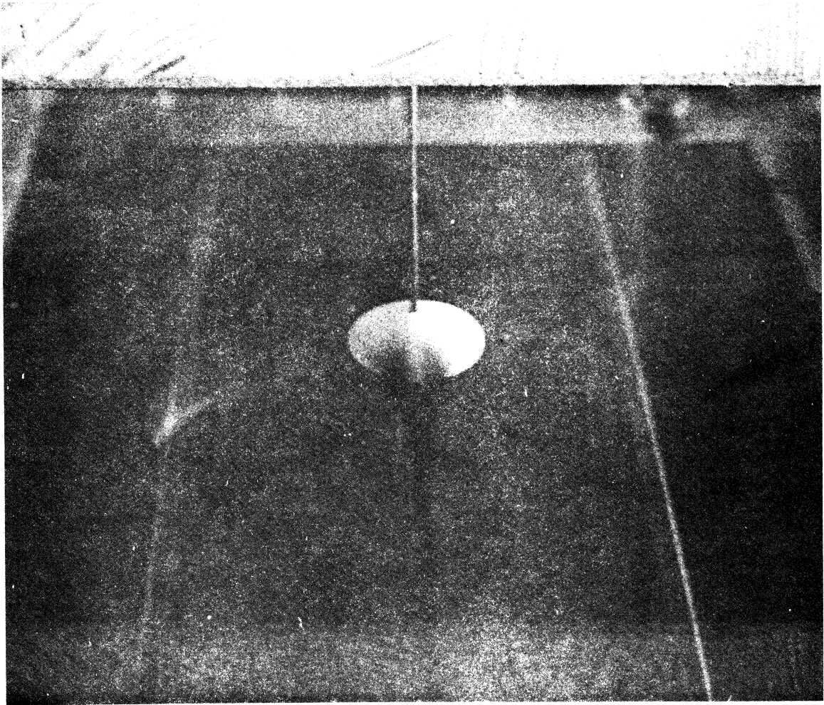
Fig. 8. Sphere being towed in a stratified liquid R = 17.6 and F_d = 0.037 . Wake appears two dimensional in view. Extent of latitudes having horizontal flow can be inferred.
