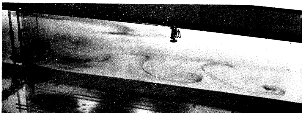
Fig. 9. Four stages in the development of a two dimensional Karman vortex street behind a sphere moving in a stratified liquid. \mathbb{R} = 377 and \mathbb{F}_d = 0.8 .
