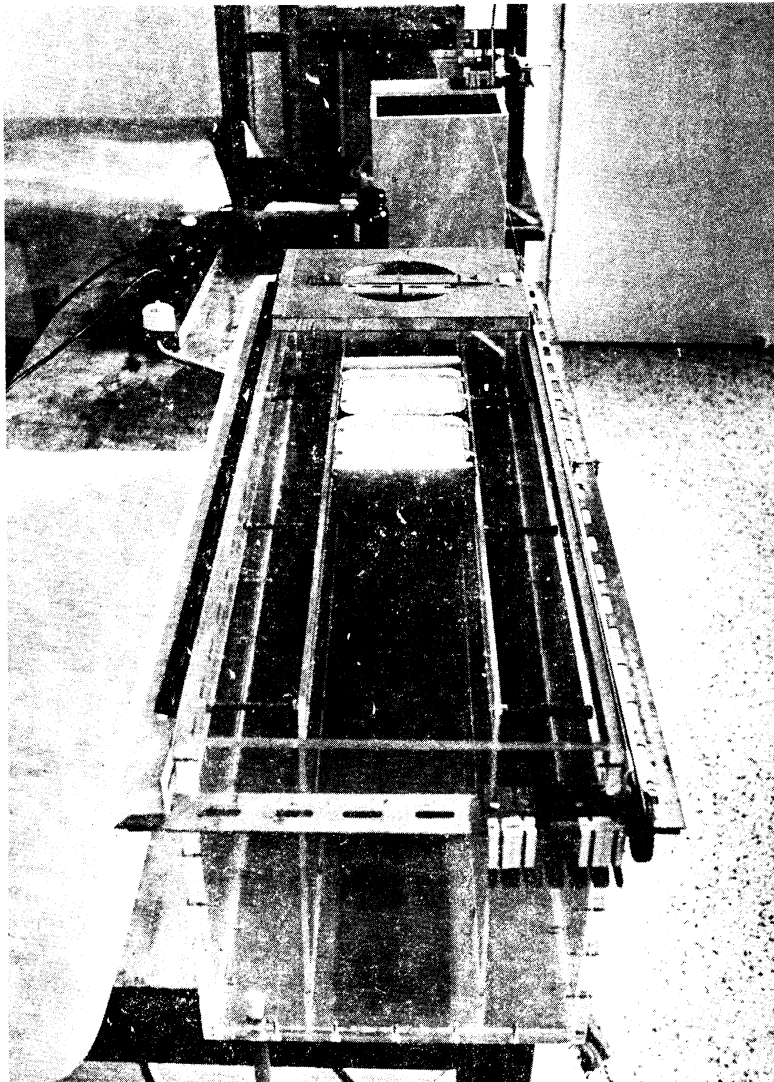
Fig. 1 b. Top view of towing tank showing flow distributor for filling.
