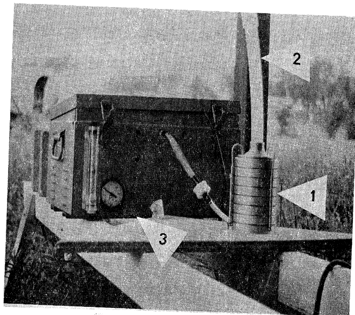
Figure 3. Shown in this photograph are the (1) Anderson sampler, its (2) intake, and the power unit a (3) Gilman pump. This setup was used for air sampling at the base station.
