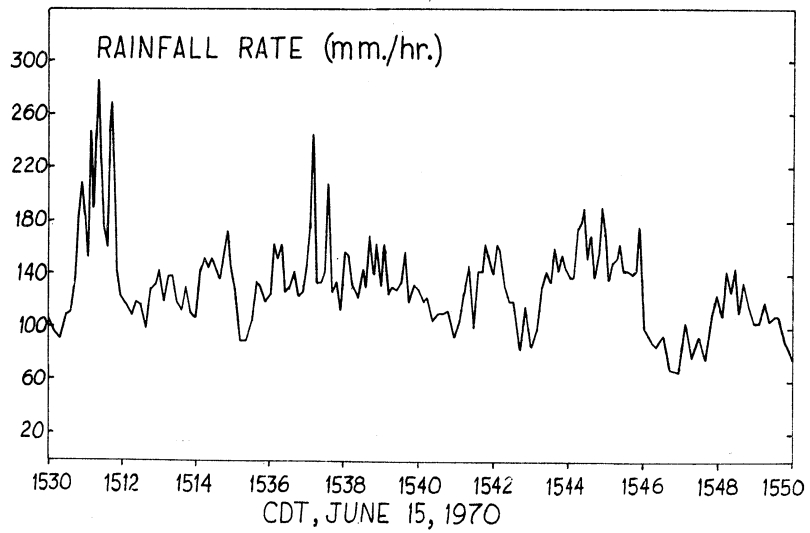
Figure 17. Rainfall intensity for rain of 15 June 1970, at Clinton, Illinois.
