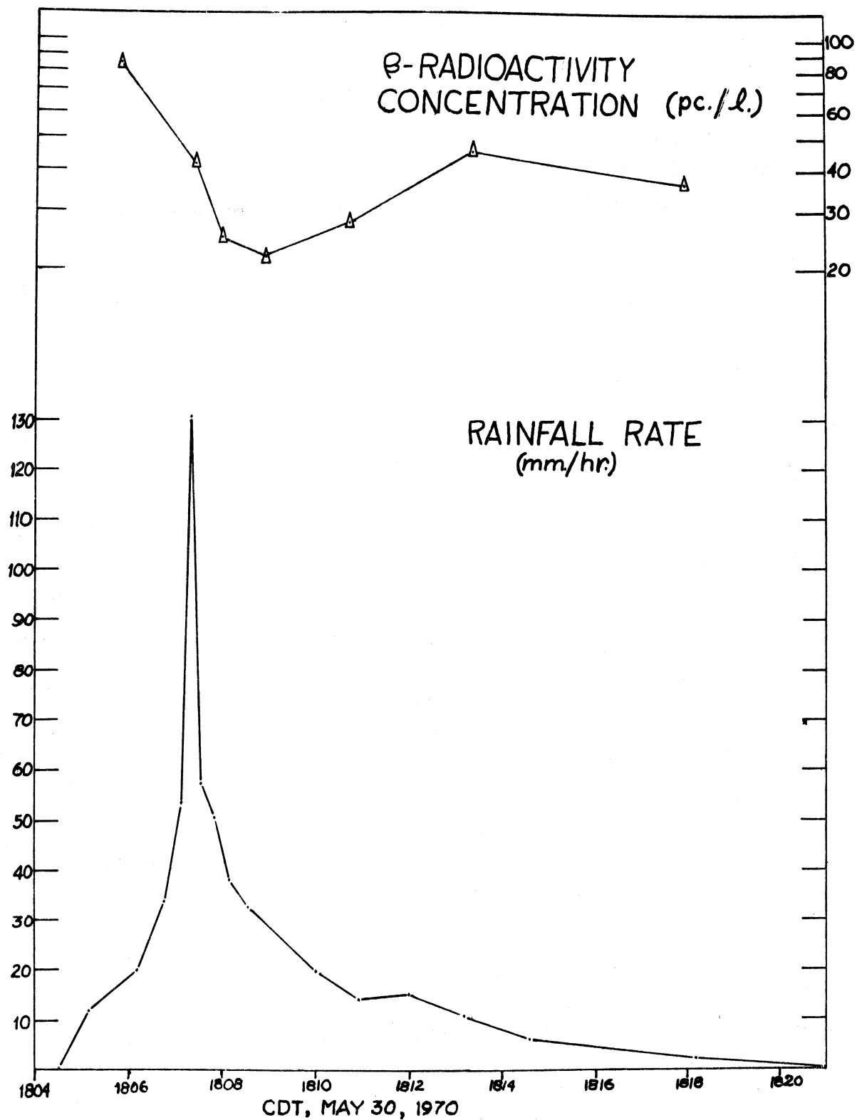
Figure 15. Rainfall intensity and \beta -radioactivity concentration for rain samples collected on 30 May 1970 at Clinton, Illinois.
