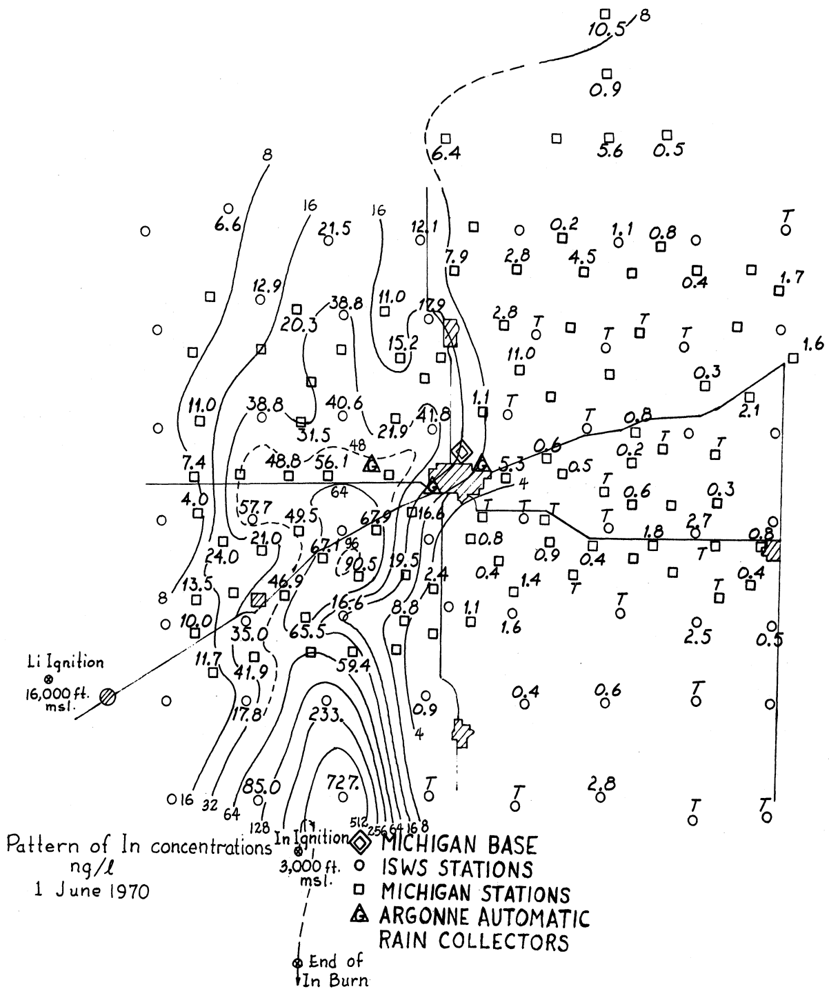
Figure 12. Map showing the distribution of Indium concentrations in the whole storm rain samples collected in the network on 1 June 1970. Also indicated is the aircraft path followed during the indium burn.
