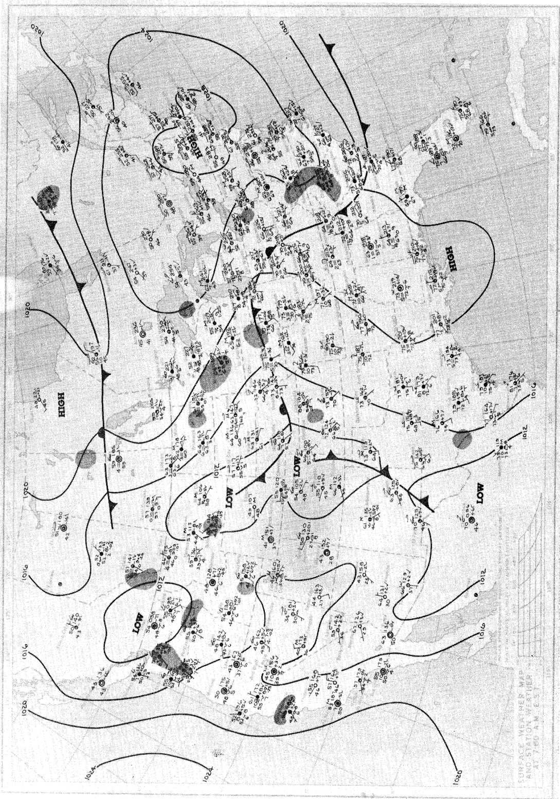
Figure 7a. Weather map at 0700 CDT. Surface map for 14 June 1970.
