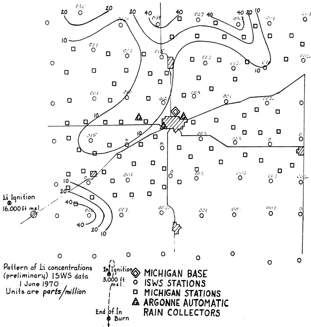
Figure 13. Map showing the distribution of lithium concentrations in the whole storm rain samples collected in the network on 1 June, 1970. Along with these preliminary ISWS results is indicated the aircraft path followed during the lithium burn.
