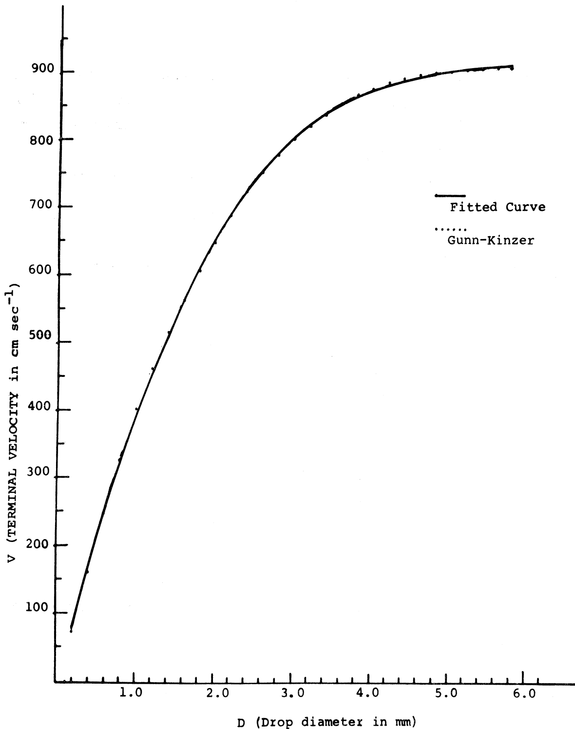
Figure 22. Results of third degree least squares fit to terminal fall speed data of Gunn and Kinzer (1949) for the diameter range 0.1 to 1.4 mm and 1.4 to 5.8 mm (see also Tables 7a & 7b).
