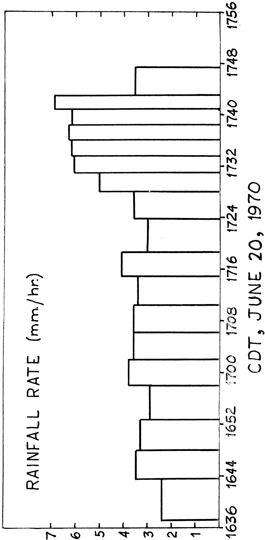
Figure 18. Rainfall intensity for rain of 20 June 1970, at Clinton, Illinois.
