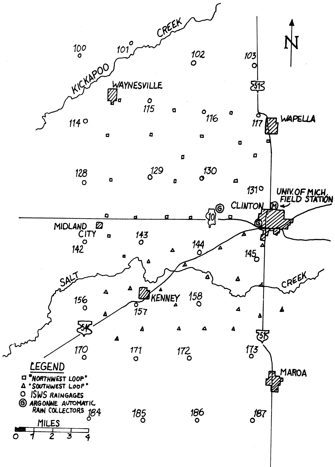
Figure 1a. Network master map of Clinton, Illinois area in the spring of 1970 showing the Northwest and Southwest "loops".
