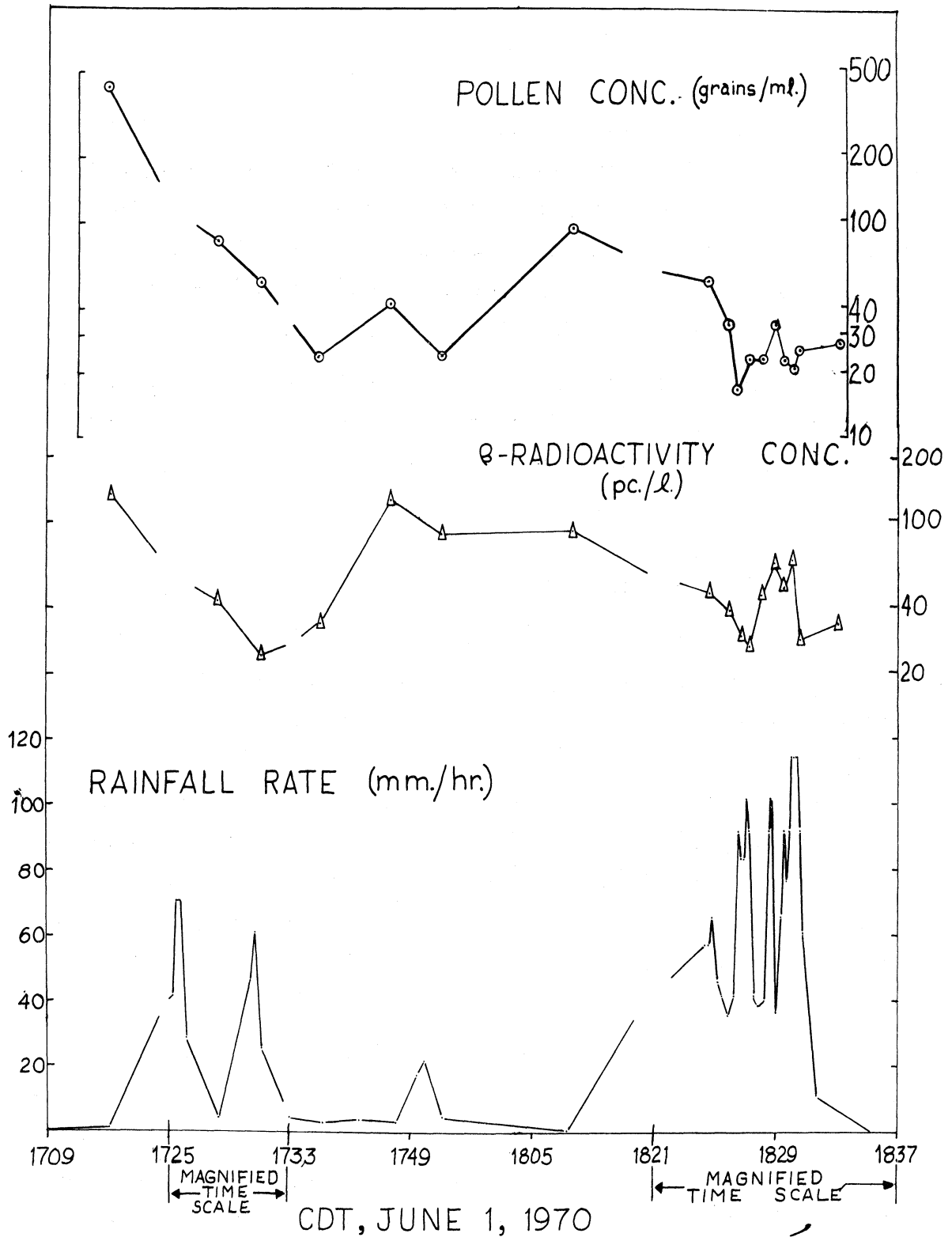
Figure 14. Rainfall intensity variations and pollen and \beta -radioactivity concentration for rain samples collected on 1 June, 1970, at Clinton, Illinois.
