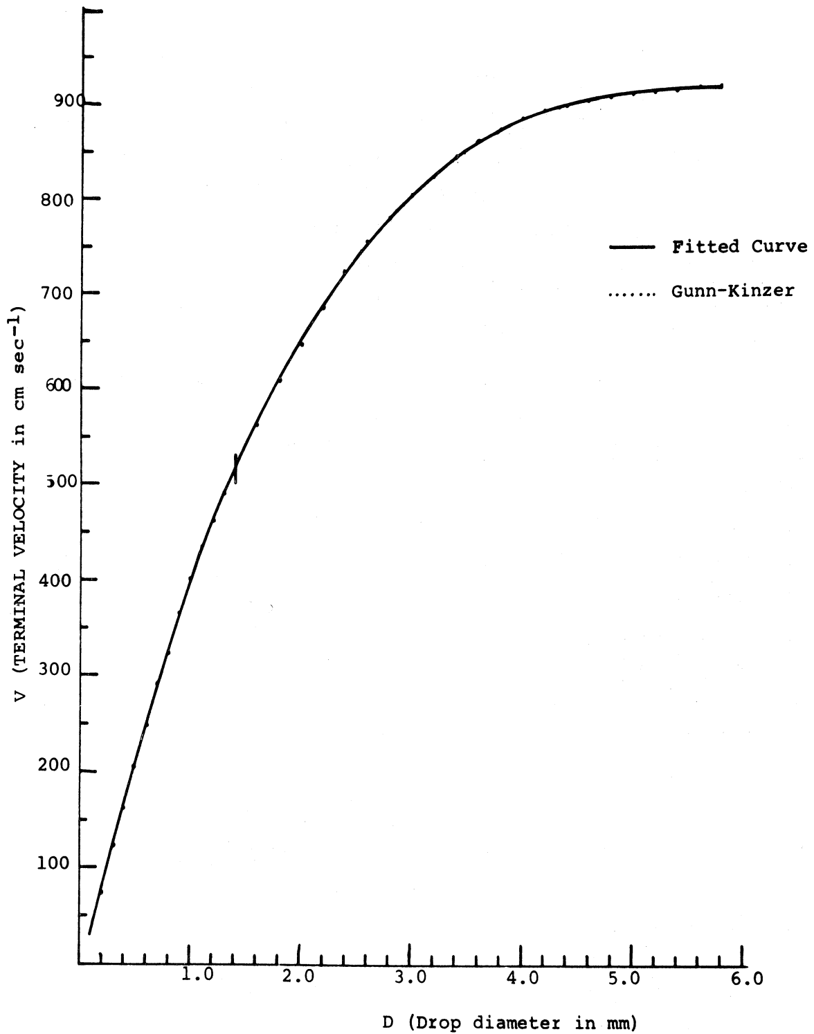
Figure 21. Results of third degree least squares fit to terminal fall speed data of Gunn and Kinzer (1949) for the diameter range 0.1 to 5.8 mm (see also Table 6).
