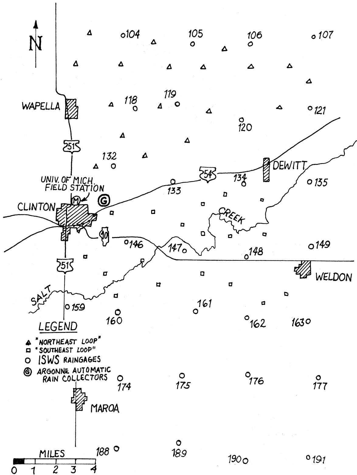
Figure 1b. Network master map of Clinton, Illinois area in the spring of 1970 showing the Northeast and Southeast "loops".
