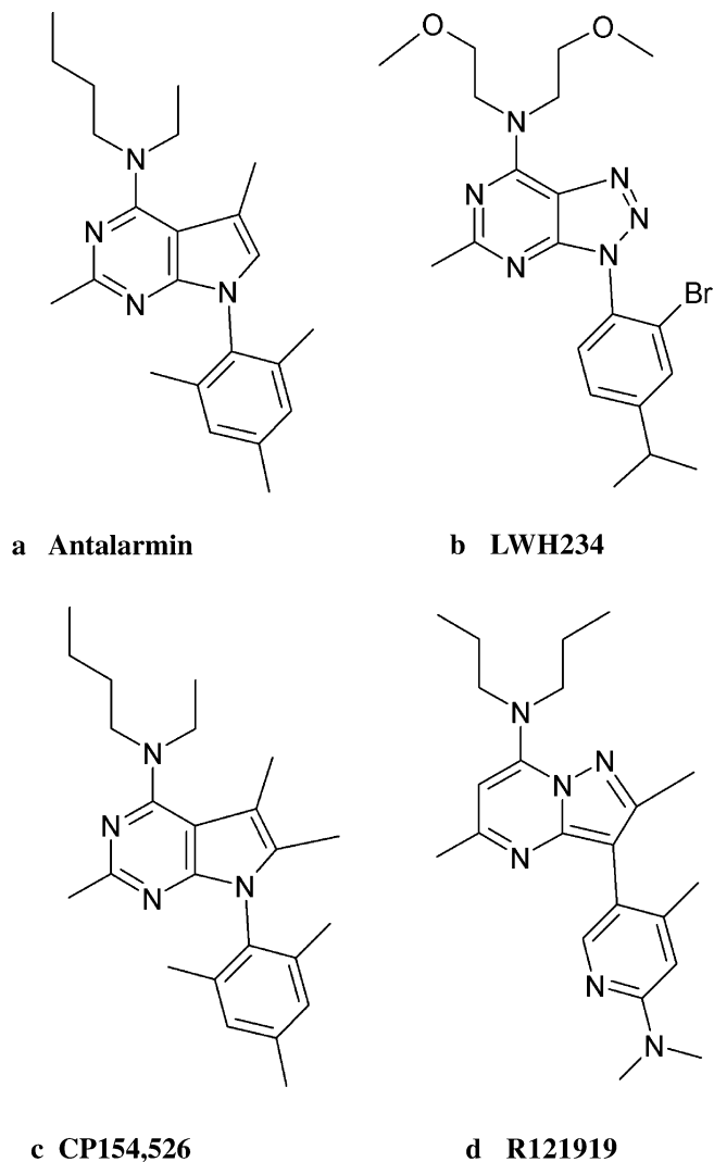
Fig. 1 Structures of antalarmin (a), LWH234 (b), CP154,526 (c), and R121919 (d)
