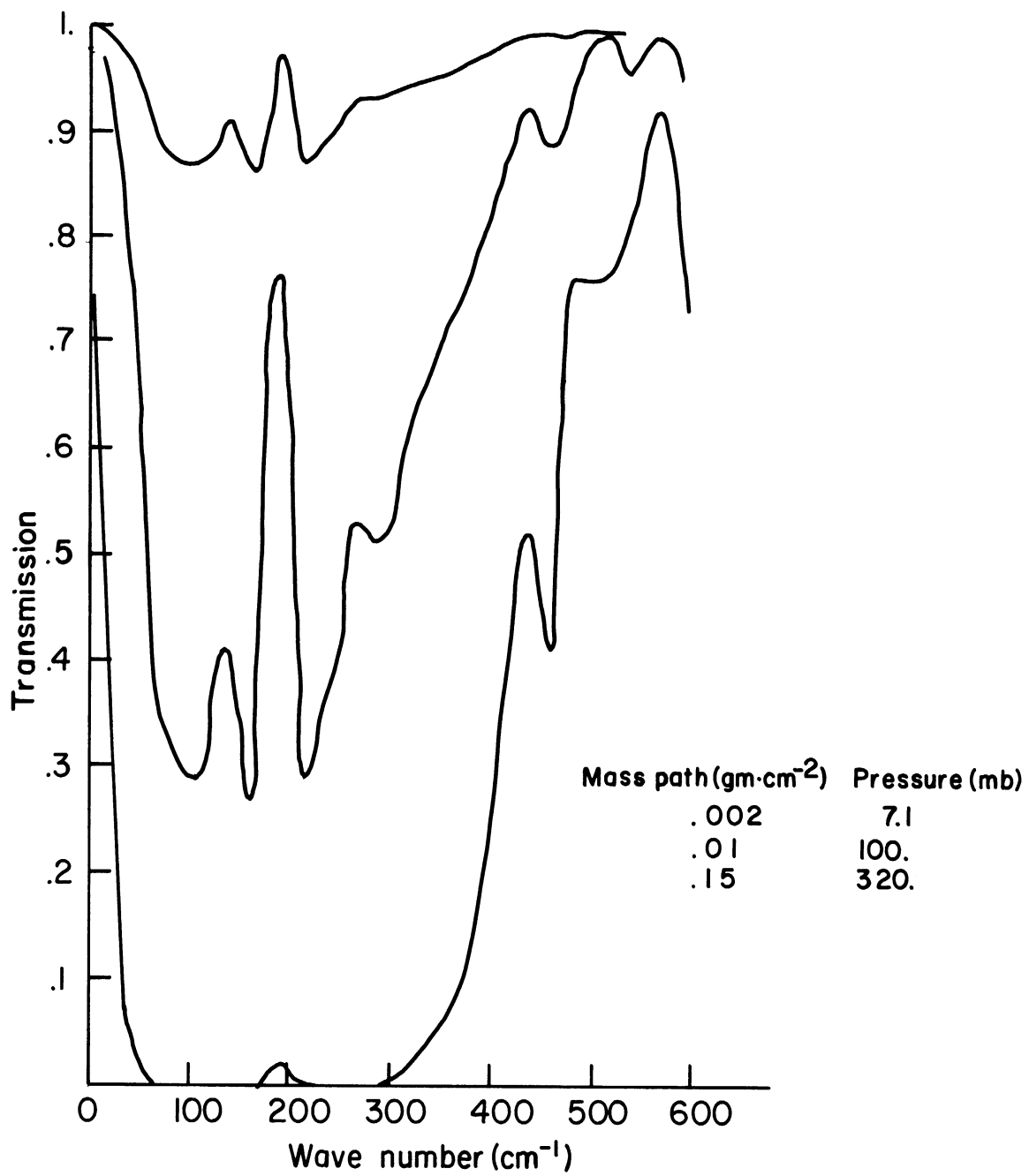
Fig. 1. Flux transmissivities for the 80 \mu\text{m} H 2 O band as calculated from the quasi-random model.
