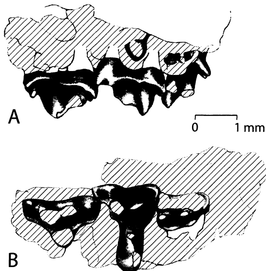
FIG. 2 — Partial upper dentition (UM 77025) of Palaeoryctes punctatus from SC-188 (Cf-2) in the Clarks Fork Basin. Drawings show a fragmentary left maxilla with crowns of a broken P 4 , complete M 1 , and a broken M 2 in lateral (A) and occlusal (B) views. Note that the M 1 and M 2 are of similar length.
