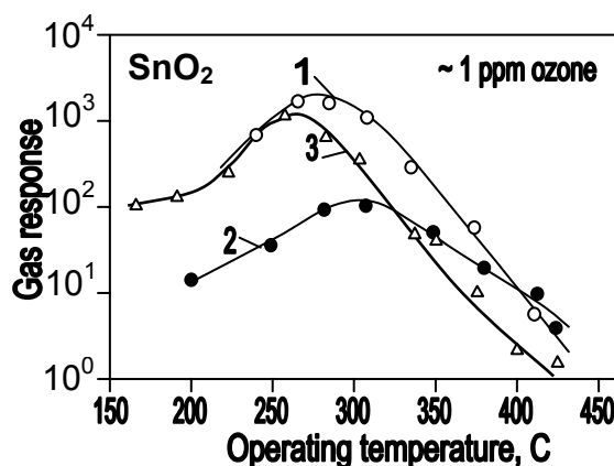
Figure 2. Temperature dependencies of \text{SnO}_2 gas response to ozone. Films deposited by SILD method using: 1- 20; 2-30; 3- 40 deposition cycles.
