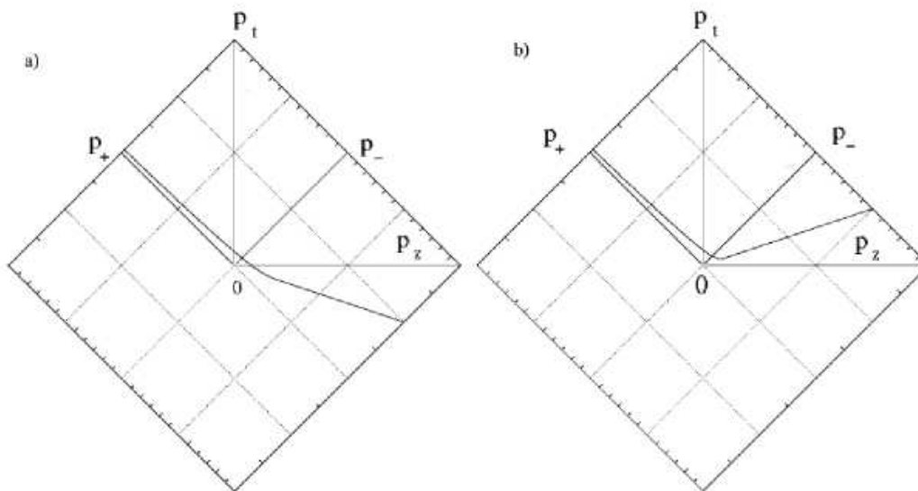
Figure 1: Plots of plausible p_- > 0 dispersion relation for a) large L\tilde{\mu} and b) small L\tilde{\mu} . Here \epsilon = 1 . The p_- < 0 branches can be obtained by inverting these diagrams through the origin.
