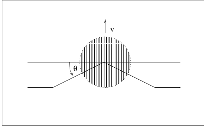
Figure 1: A black hole encountering the domain wall with a relative velocity v .
