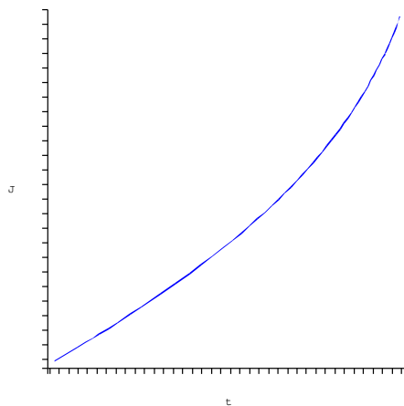
Figure 4: A parametric plot of (4.29) for x \rightarrow 1 shows similarity with the bottomonium trajectory.
