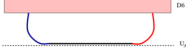
Figure 2: String ending on the probe D6.
