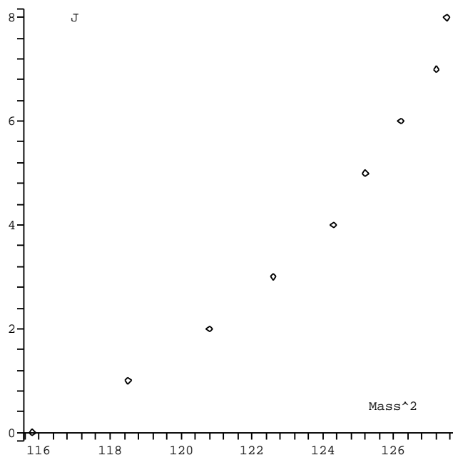
Figure 3: The bottomonium trajectory [22, 21].
