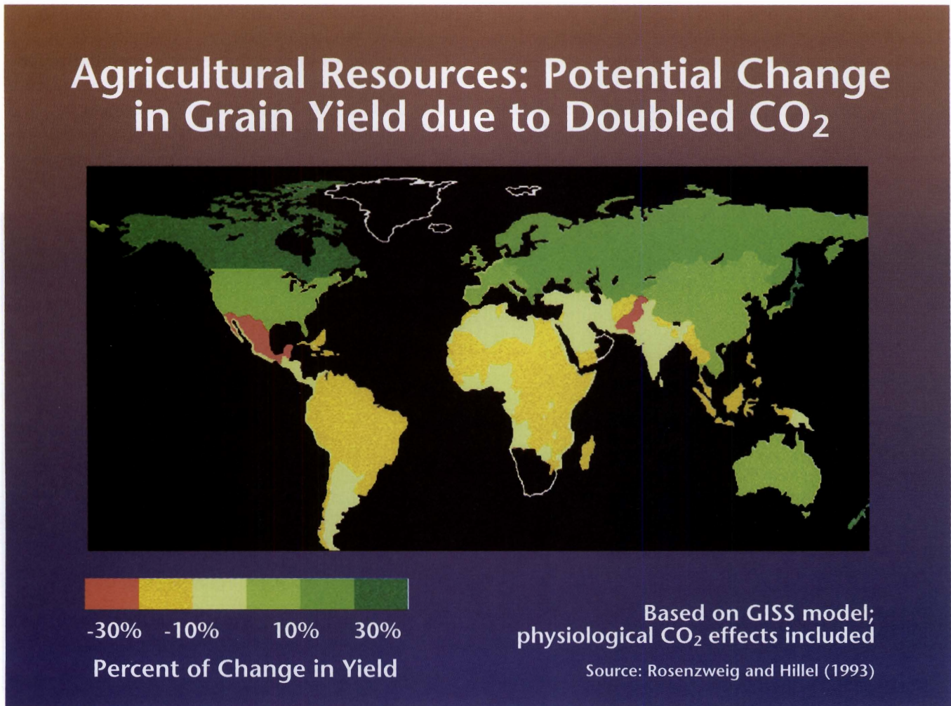
Figure 20. Agricultural production would increase in some areas, and decline in others as the climate warms and the CO 2 levels in the atmosphere increase. Farmers may need to shift crops, or re-locate agricultural lands. The need for irrigation may also increase.
