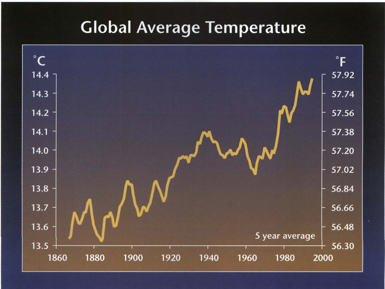
Figure 7. The global average temperature has risen by approximately 1° F over the last century.
