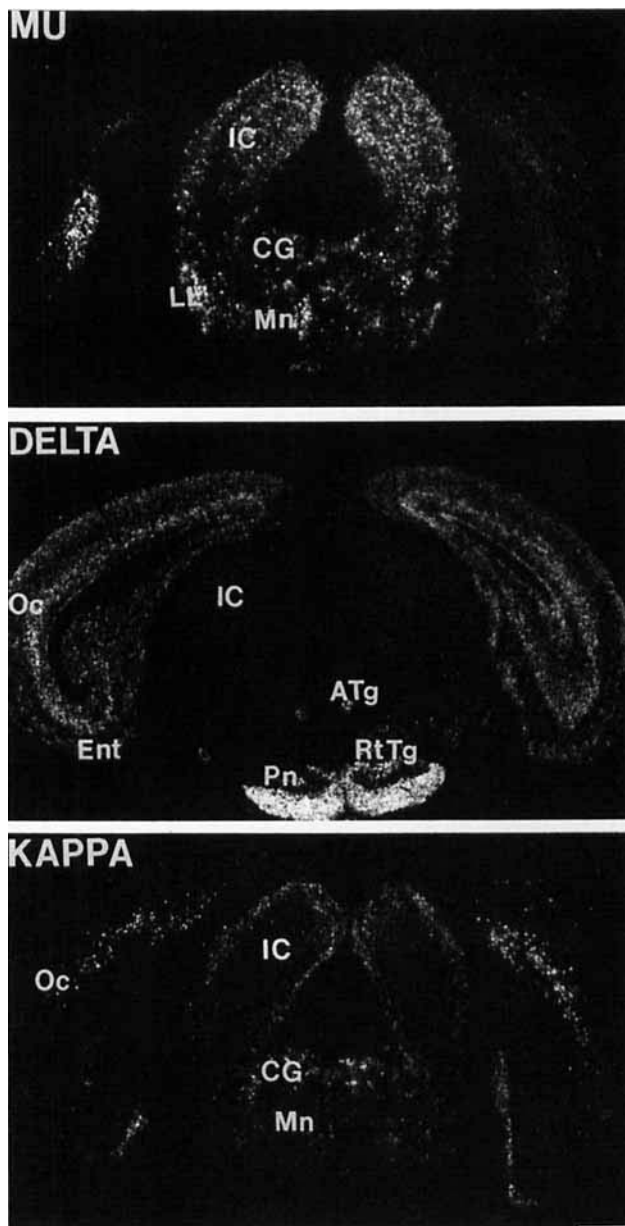
Fig. 8. Darkfield autoradiograms comparing \mu , \delta , and \kappa receptor mRNA expression at the level of the pontine nuclei. \delta Receptor mRNA expression is prominent in the pontine nuclei, reticulotegmental nucleus of the pons, and anterior tegmental nucleus, all regions not demonstrating \mu or \kappa receptor mRNA expression. As was shown in preceding figures, cells expressing \delta receptor mRNA are also prominent in the occipital and entorhinal cortices. Cells expressing \mu receptor mRNA are localized in the central and external cortices of the inferior colliculus, pontine central gray, lateral lemniscus, and median raphe. In contrast, cells expressing \kappa receptor mRNA are restricted to the dorsal and external cortices of the inferior colliculus. Other regions expressing \kappa receptor mRNA include layers 5 and 6 of the occipital cortex, pontine central gray, and median raphe. A higher resolution image of the cells in the median raphe expressing \mu receptors is provided in Figure 16. Scale bar = 1,000 \mu m.
