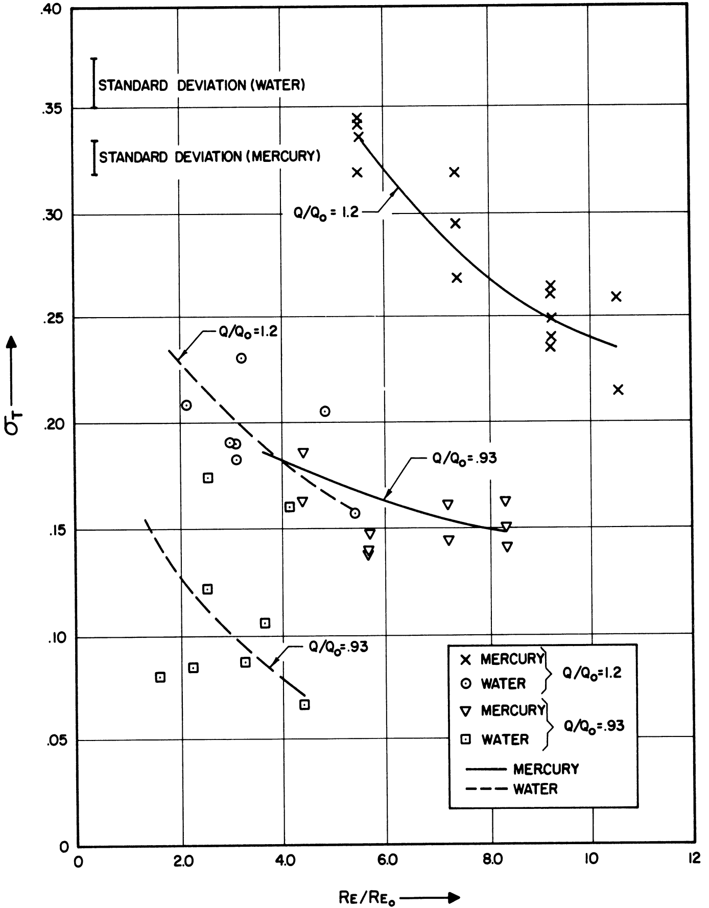
Figure 4. Thoma Cavitation Parameter vs. Normalized Reynolds' Number.
