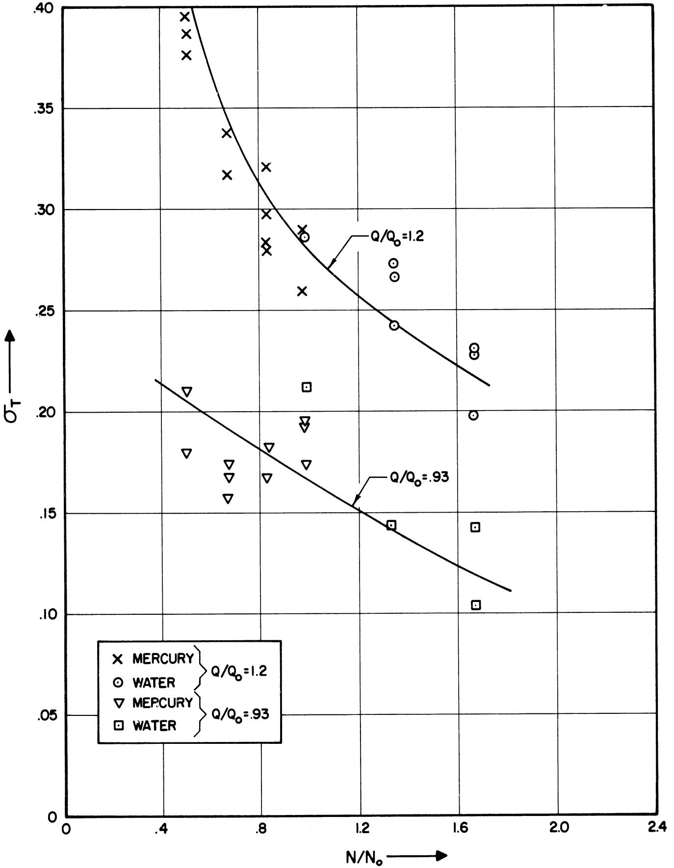
Figure 9. Thoma Cavitation Parameter vs. Normalized Pump Speed Based on First Break Due to Cavitation.
