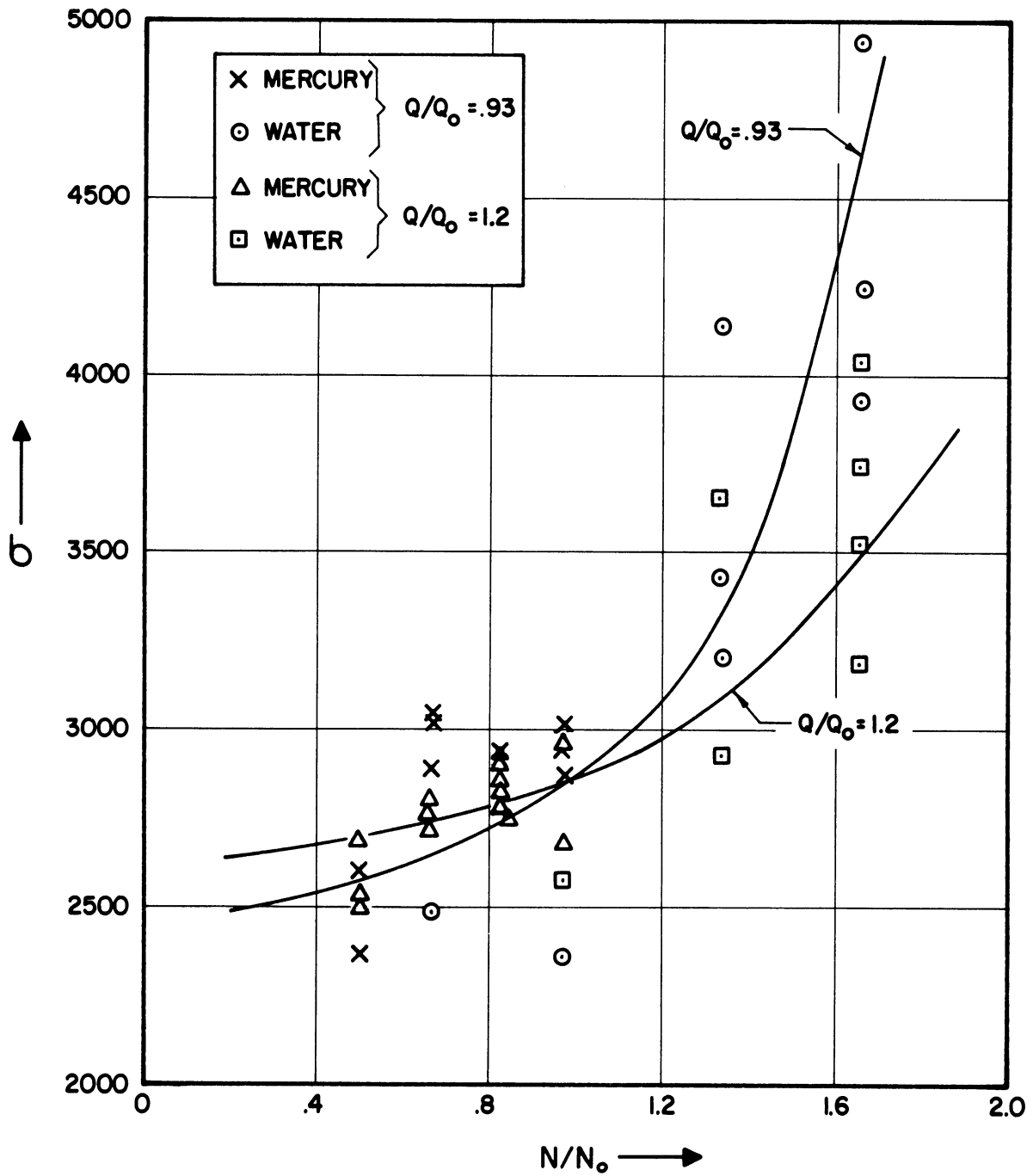
Figure 5. Suction Specific Speed vs. Normalized Pump Speed for Water and Mercury at Two Different Normalized Flow Conditions Using Berkeley Model 1 1/2 WSR Centrifugal Pump.
