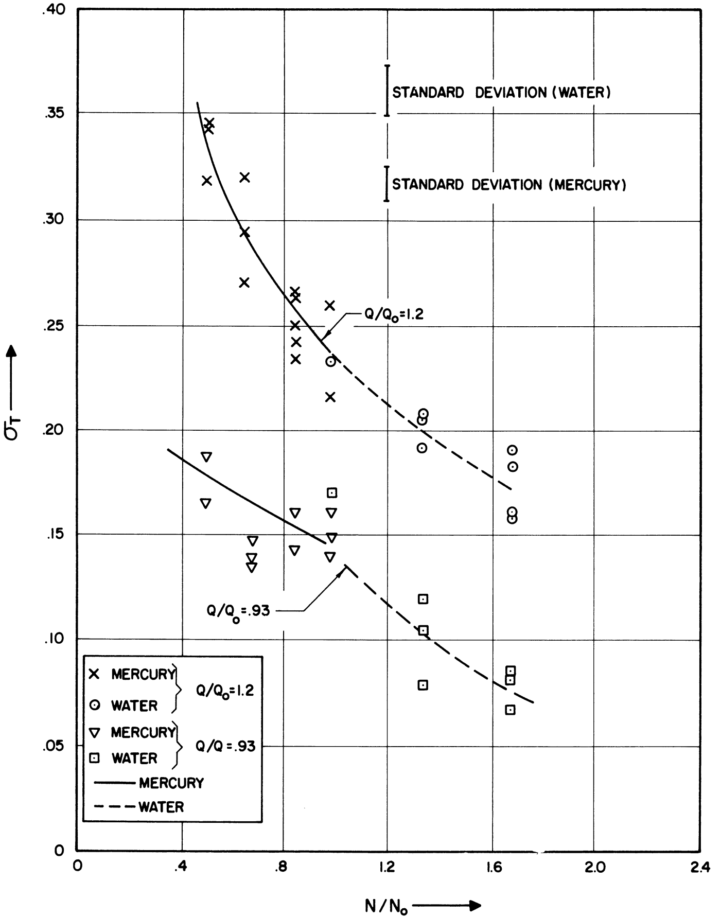
Figure 3. Thoma Cavitation Parameter vs. Normalized Pump Speed.
