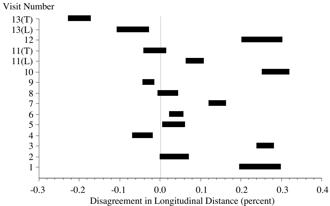
Figure 1. Consistency in longitudinal distance measurement.
