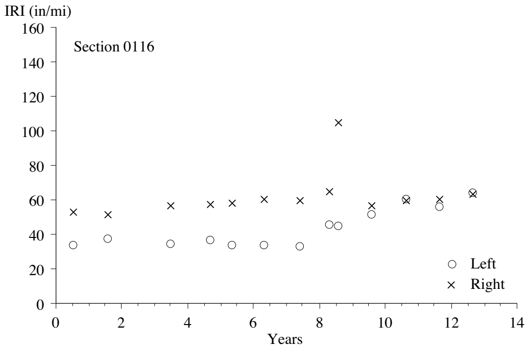
Figure 5. IRI progression, section 0116.
