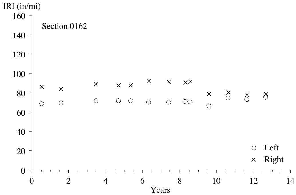
Figure 16. IRI progression, section 0162.
