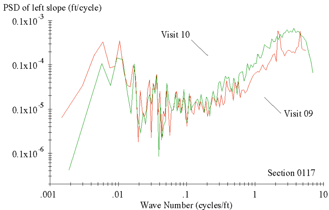
Figure 19. PSD of section 0117 profile, left side.
