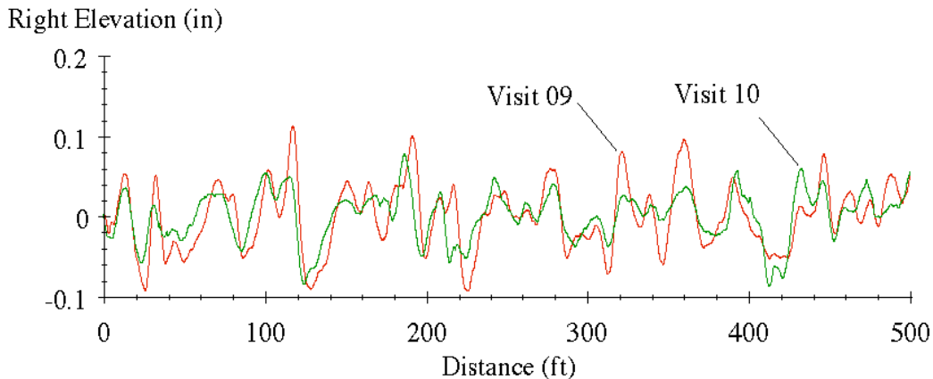
Figure 22. Medium wavelength profiles of section 0122.
