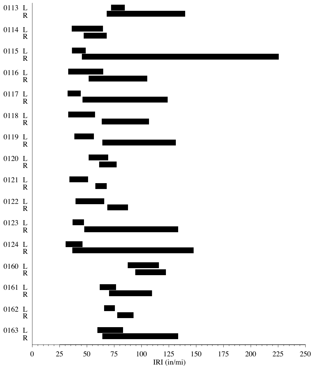
Figure 25. Summary of IRI ranges.
