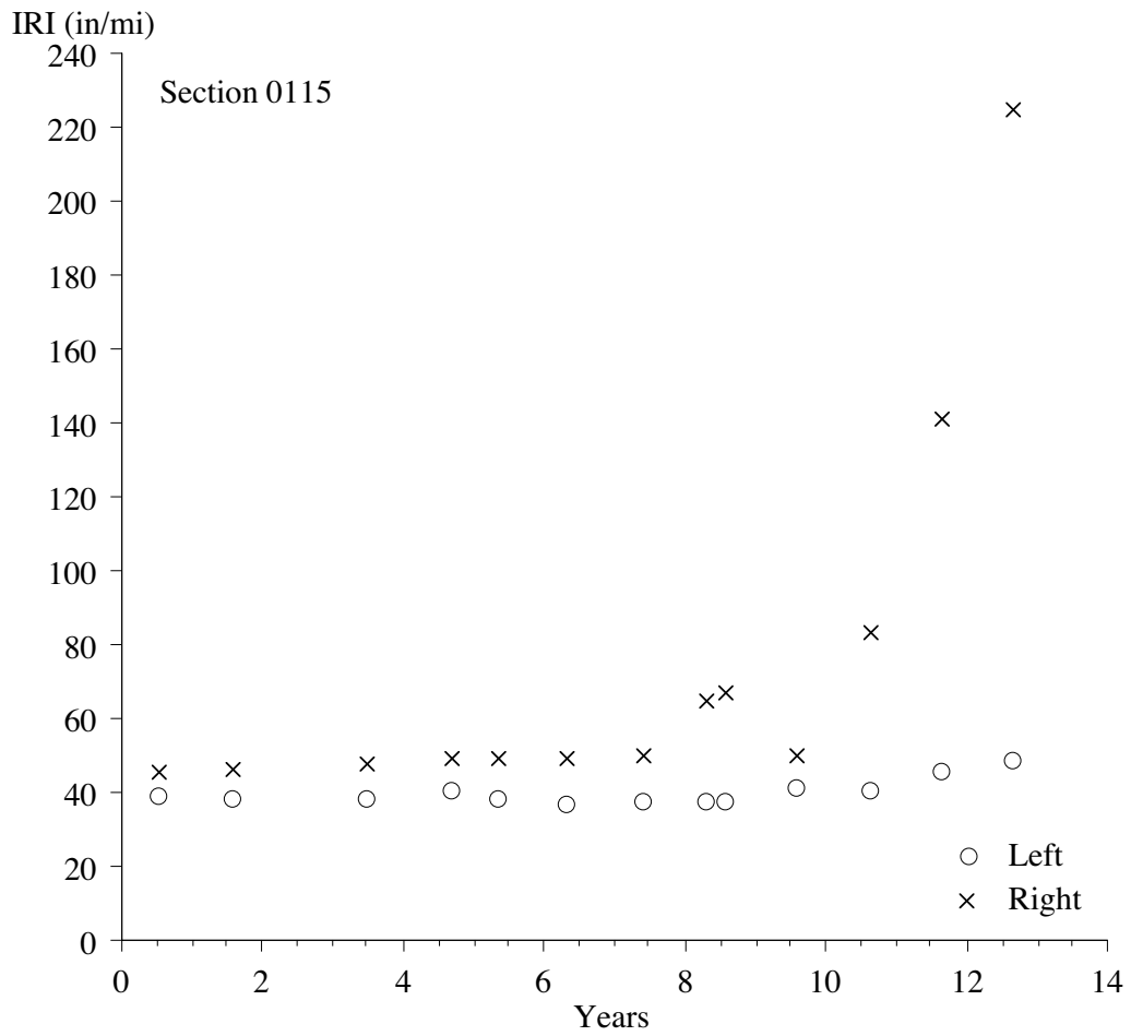
Figure 3. IRI progression, section 0115.
