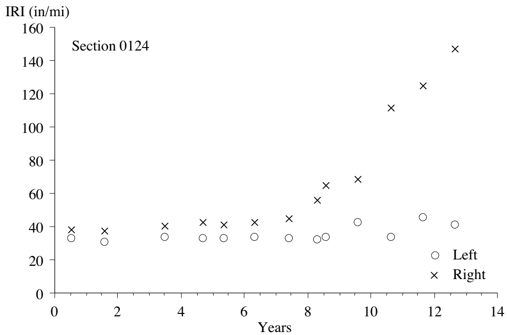
Figure 13. IRI progression, section 0124.
