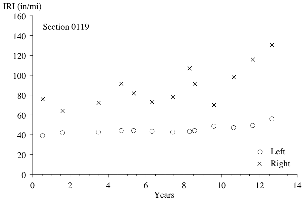
Figure 8. IRI progression, section 0119.
