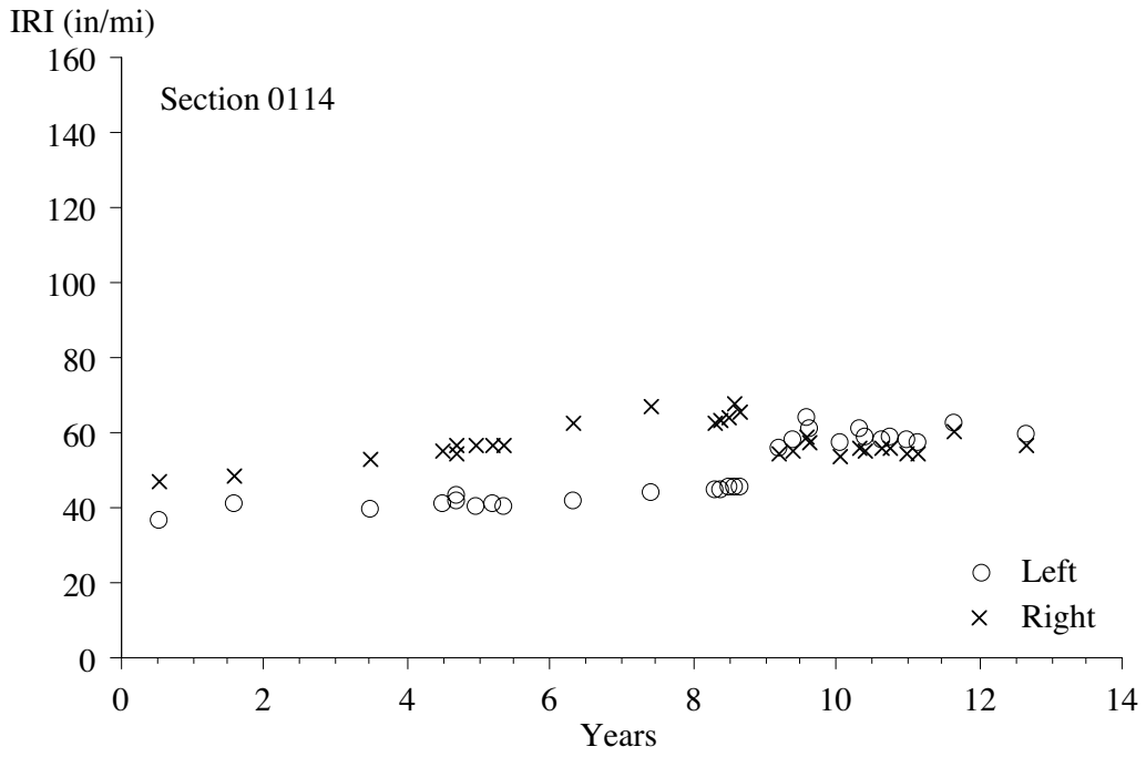
Figure 4. IRI progression, section 0114.
