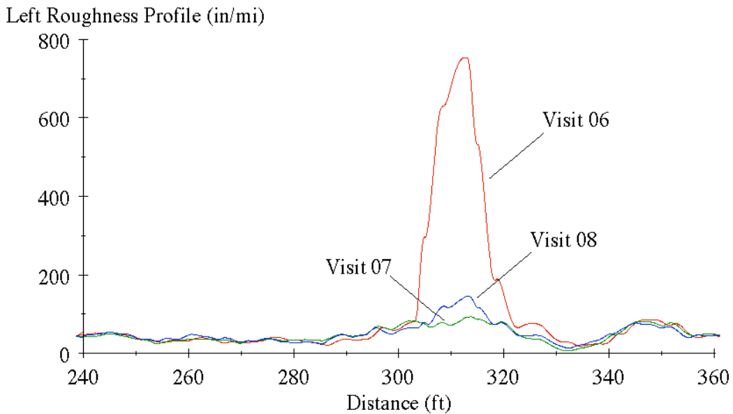
Figure 24. Roughness profile of section 0122, 10-ft baselength.
