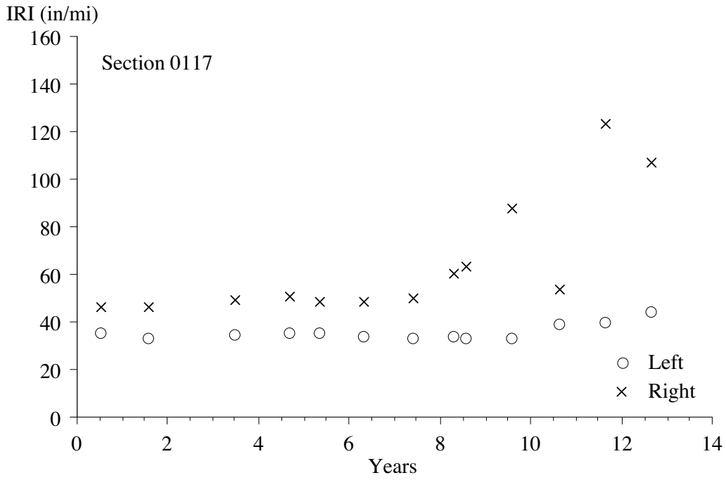
Figure 6. IRI progression, section 0117.
