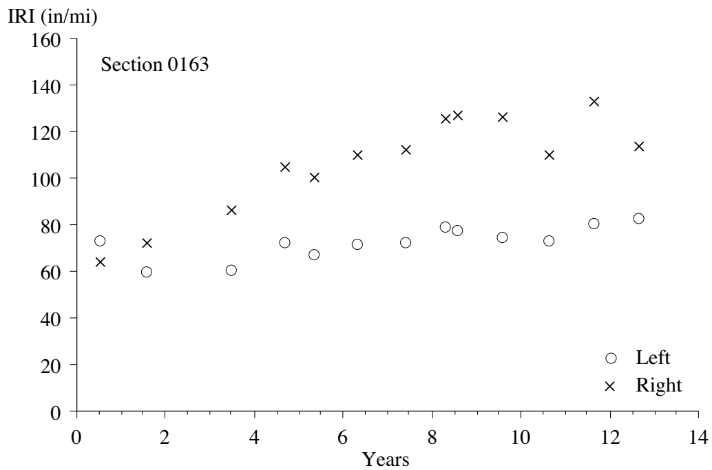
Figure 17. IRI progression, section 0163.
