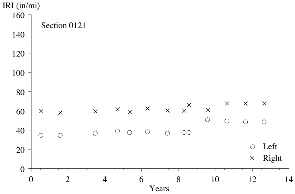
Figure 10. IRI progression, section 0121.
