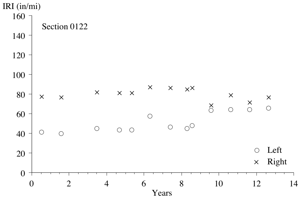
Figure 11. IRI progression, section 0122.
