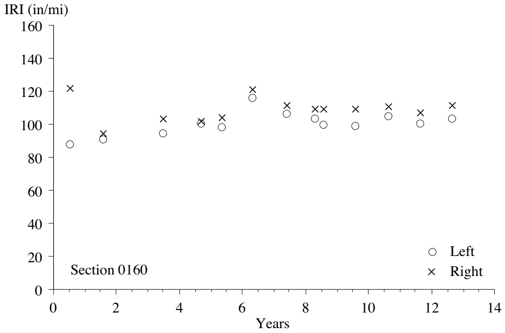
Figure 14. IRI progression, section 0160.
