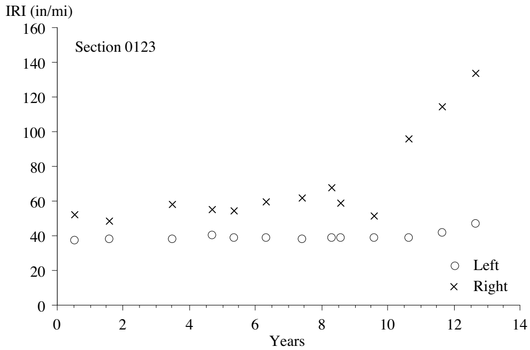
Figure 12. IRI progression, section 0123.
