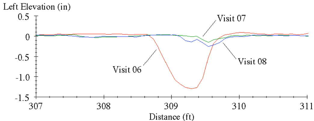
Figure 21. Filtered profile of section 0122.
