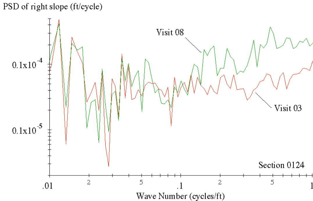
Figure 18. PSD of section 0124 profile, right side.
