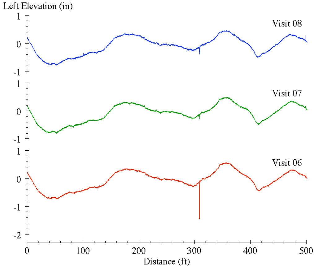
Figure 20. Raw profiles of section 0122.
