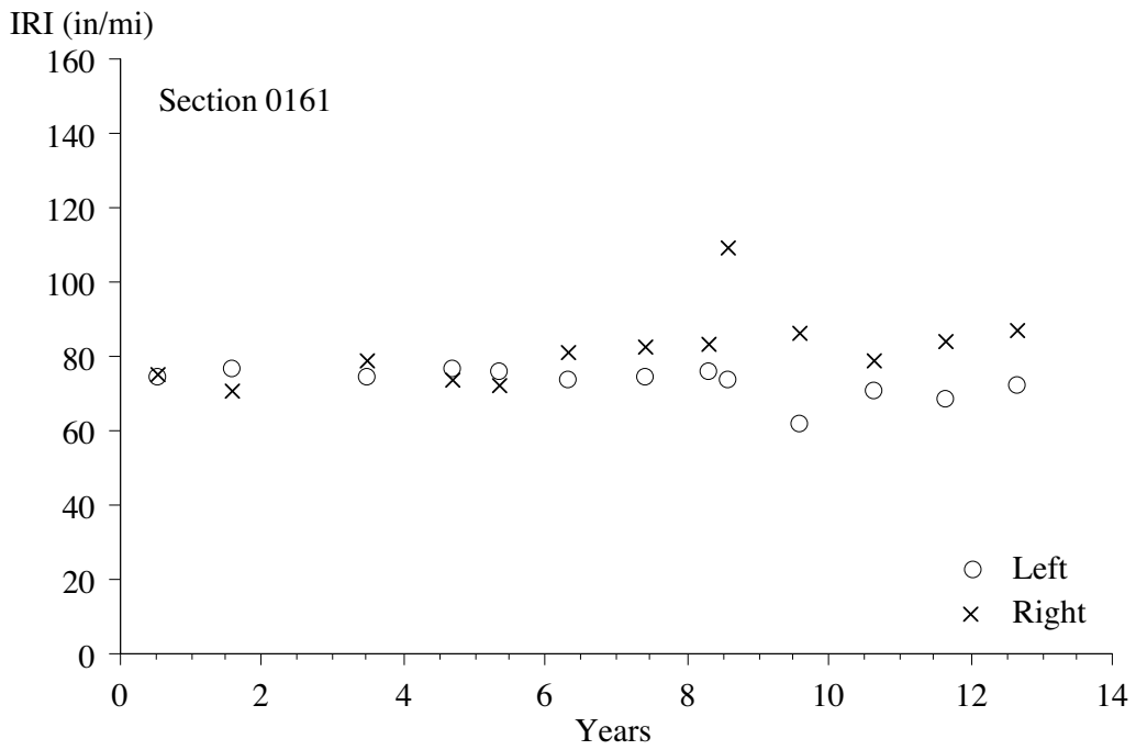
Figure 15. IRI progression, section 0161.
