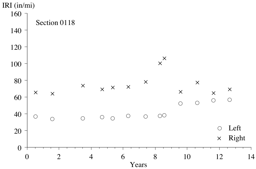
Figure 7. IRI progression, section 0118.
