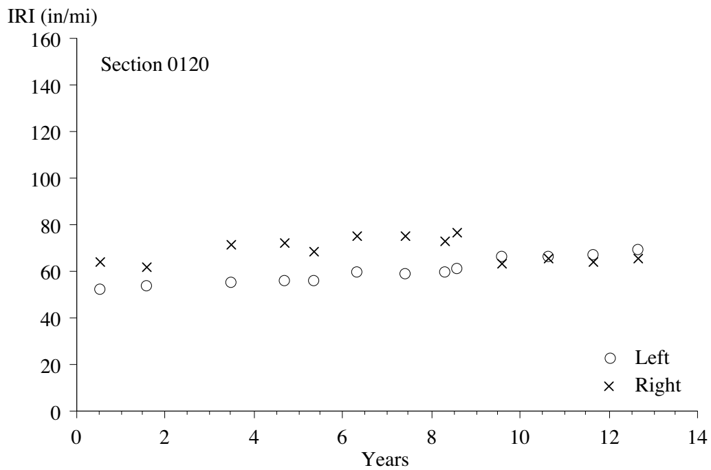
Figure 9. IRI progression, section 0120.
