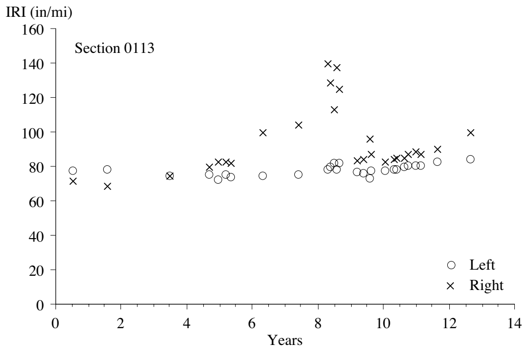
Figure 2. IRI progression, section 0113.
