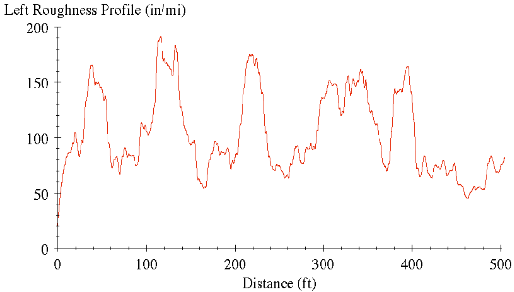
Figure 23. Roughness profile of section 0160, 25-ft baselength.
