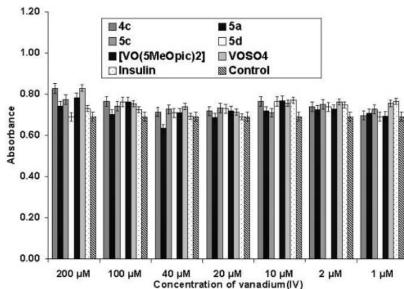
Figure 5. Glucose uptake stimulated by the vanadium picolinates 4c , 5a , 5c and 5d after 60 min. The absorbance, shown relative to a control group, reflects the efficacy of the compounds. The diagram also shows the data for [VO(5MeOdipic) 2 ], VOSO 4 , and a group of cells where insulin was added instead of vanadium.
