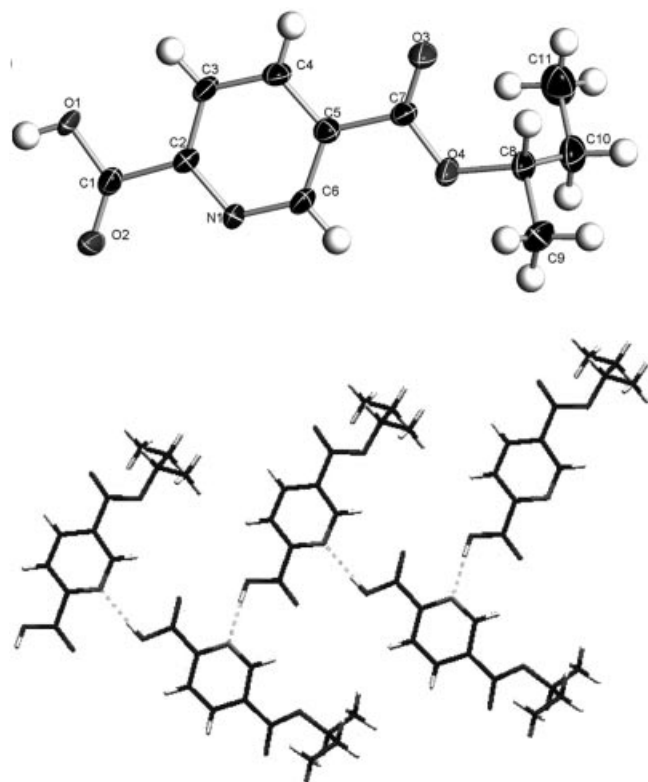
Figure 1. Top: XSHHELL plot of 2b (50% probability level). Bottom: Hydrogen bonding network for 2b (Mercury, vers. 1.1).
