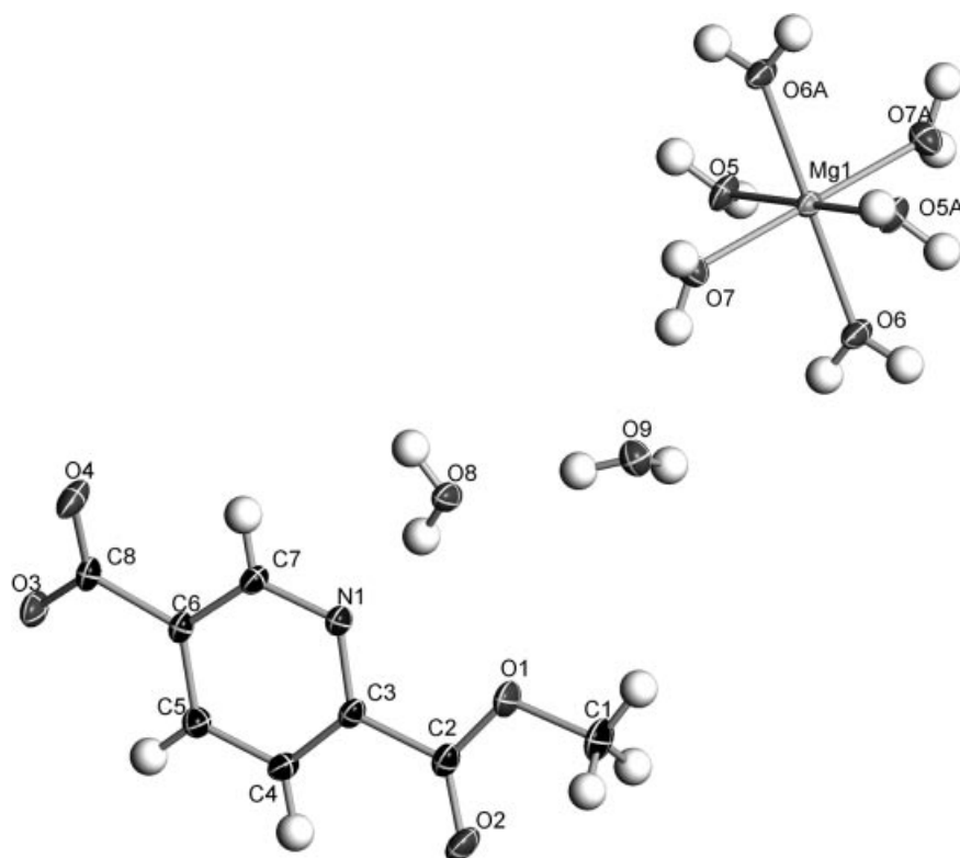
Figure 3. XSELL plot of [\text{Mg}(\text{H}_2\text{O})_6](1\text{H}_{-1})_2 \cdot 4\text{H}_2\text{O} (50% probability level). Only one of the anions 1\text{H}_{-1} and two of the waters of crystallization are shown.
