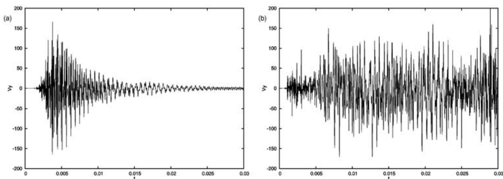
Fig. 3 Temporal evolution of the spanwise velocity component for R = 350 and Ha = 20 for a subcritical (a) and supercritical (b) perturbation as obtained in the numerical simulations of [5].
