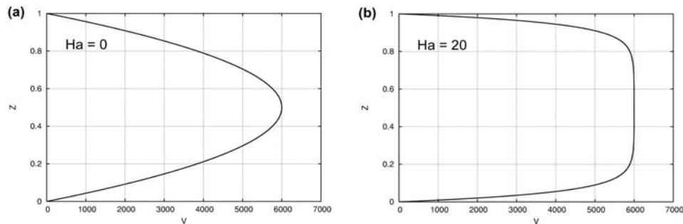
Fig. 1 Parabolic velocity profile (a) and Hartmann profile (b) for laminar flow in a channel.
