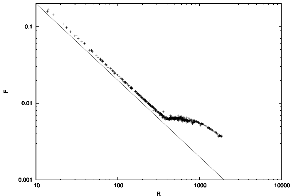
Fig. 2 Friction factor versus R as obtained in the experiments of Moresco & Alboussière [4]. The straight line corresponds to the friction factor for laminar Hartmann layers.
