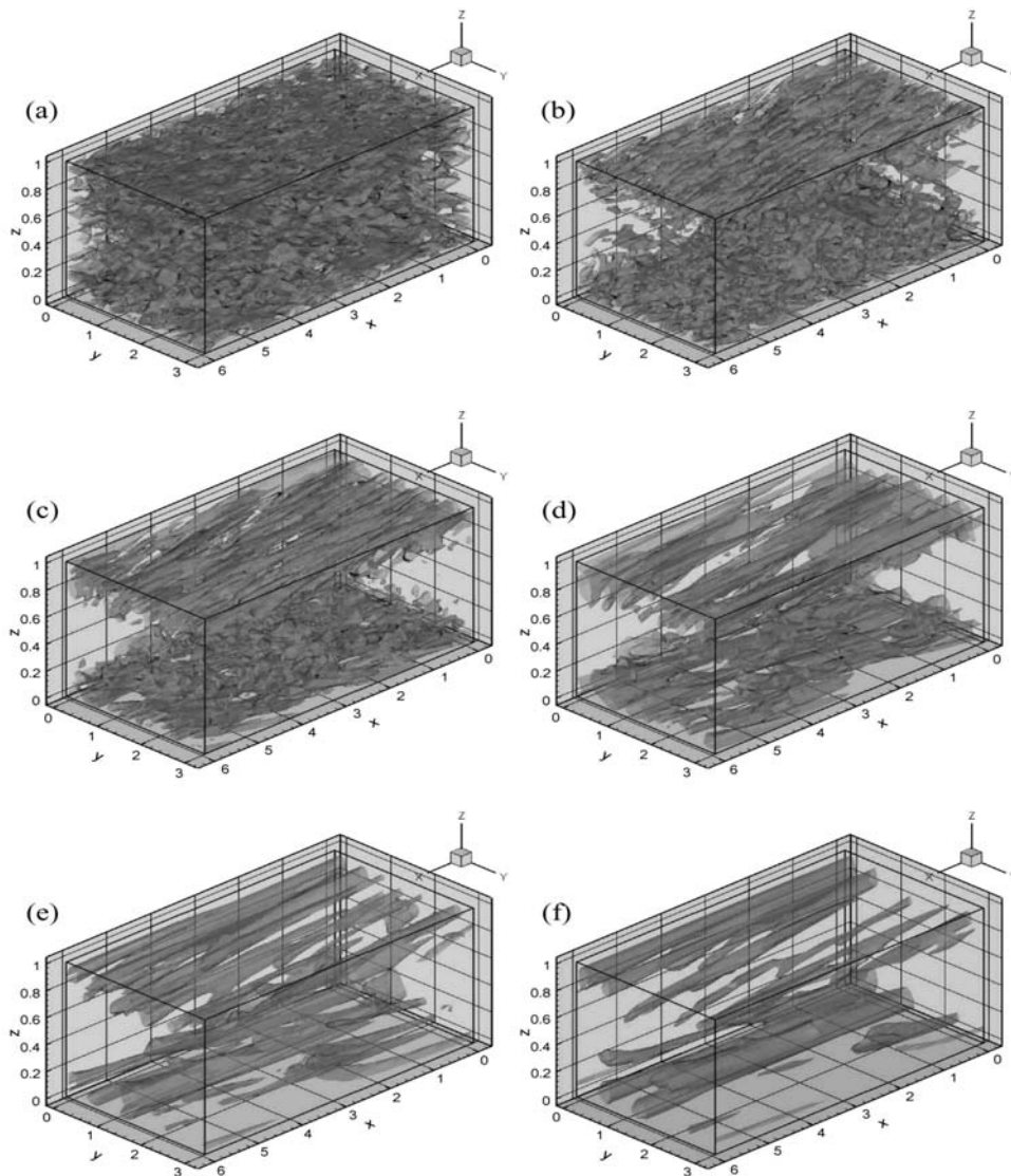
Fig. 4 Temporal evolution of the Hartmann flow with initially imposed random three-dimensional noise. Shown are the isosurfaces of the streamwise velocity fluctuations for R = 400 and Ha = 15 as obtained in the numerical simulations of [5].
