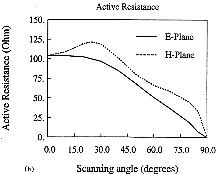
Fig. 5 Scanning reflection coefficient and active resistance as a function of scan angle for an infinite cavity-backed patch array. For this computation T_x = T_y = 0.5\lambda , the cavity size is 0.45\lambda \times 0.45\lambda \times 0.02\lambda and the patch size is 0.3\lambda \times 0.3\lambda . The cavity is filled with a dielectric having \epsilon_r = 2.8 .
