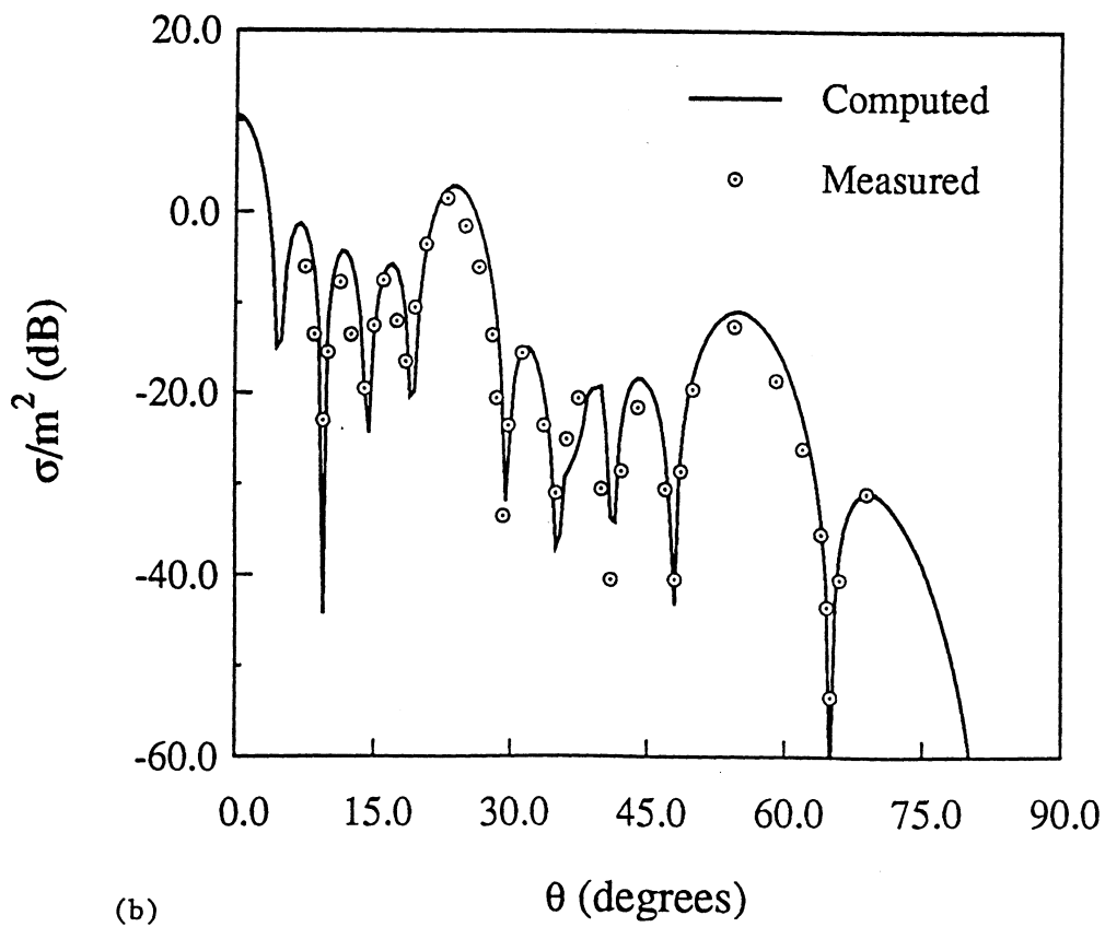
Fig. 3 Principal backscatter RCS pattern of the 5 \times 5 cavity array. For this computation T_x = T_y = 4 cm, the cavity size is 3 \text{ cm} \times 3 \text{ cm} \times 0.45 \text{ cm} and f=9.1\text{GHz} . (a) E_\theta pattern. (b) E_\phi pattern.
