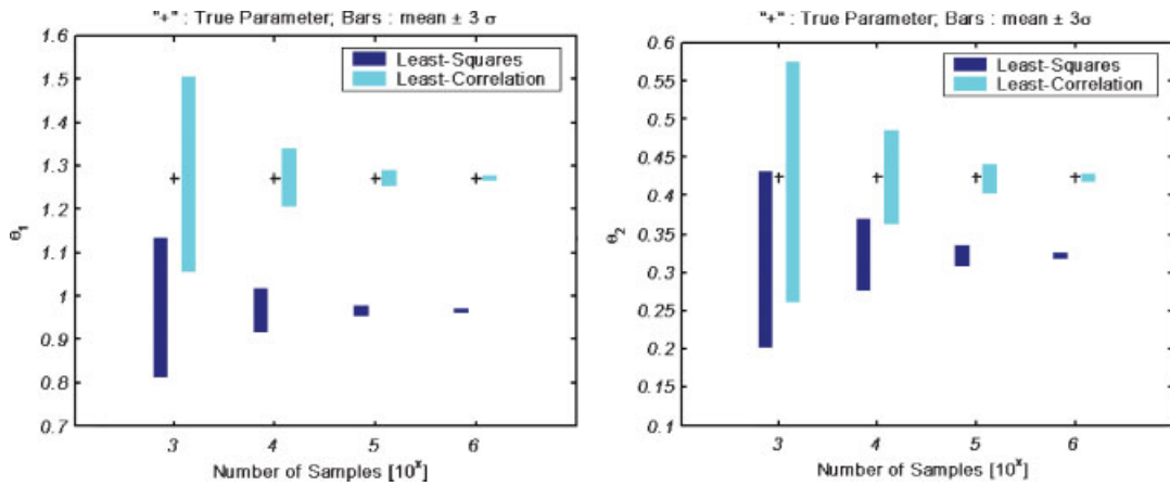
Figure 3. Effect of the number of samples: FIR input noise, SNR_i \approx SNR_o \approx 5 dB.
