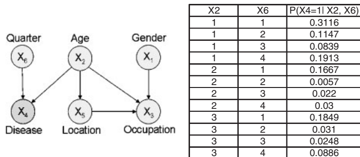
Figure 5. The structure and partial parameters of the Bayesian network in case study 1
