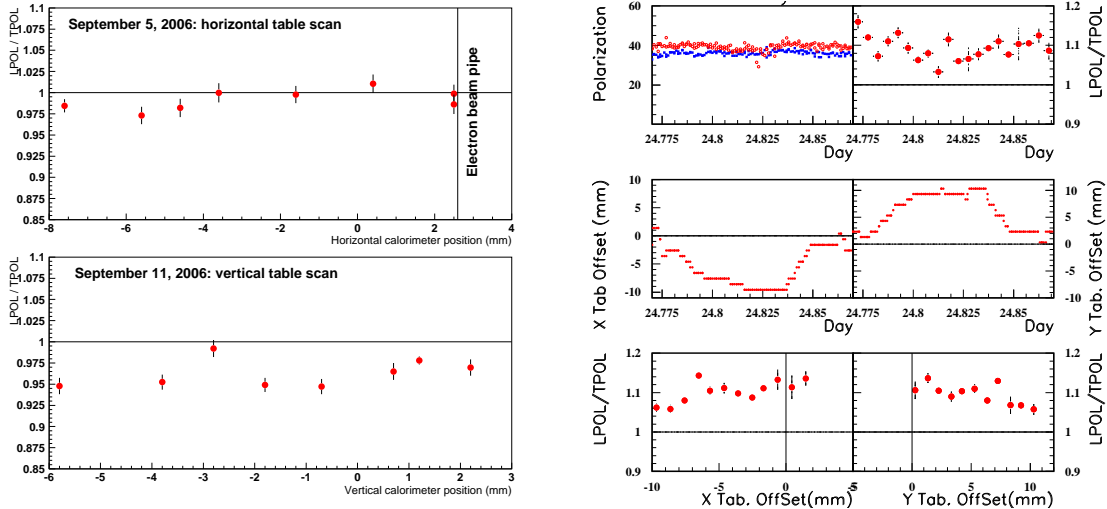
Figure 3.16: Results of a spatial calorimeter scan. In the top left panels the calorimeter was moved horizontally, in the bottom left panel vertically. The horizontal movement was limited by the electron beam pipe at the indicated position. In the right panel a similar measurement was performed during a period with a strong disagreement between the LPOL and TPOL measurements.
