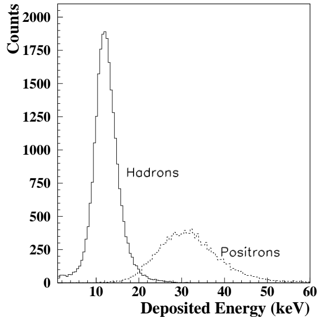
Figure 3.5: The average energy deposited in the transition radiation detector (TRD) by hadrons and leptons, averaged over all momenta. Taken from reference [7].
