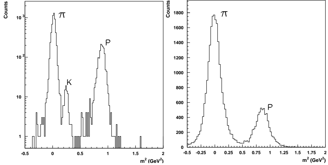
Figure 3.4: Time-of-flight hadron identification with the scintillator hodoscopes H1. Pions, kaons, and protons can be separated in the distribution of the squared mass m^2 for the momentum range 0.6–1.1 GeV (left). For the momentum range 1.5–2.0 GeV pions and protons can be distinguished. Taken from reference [14].
