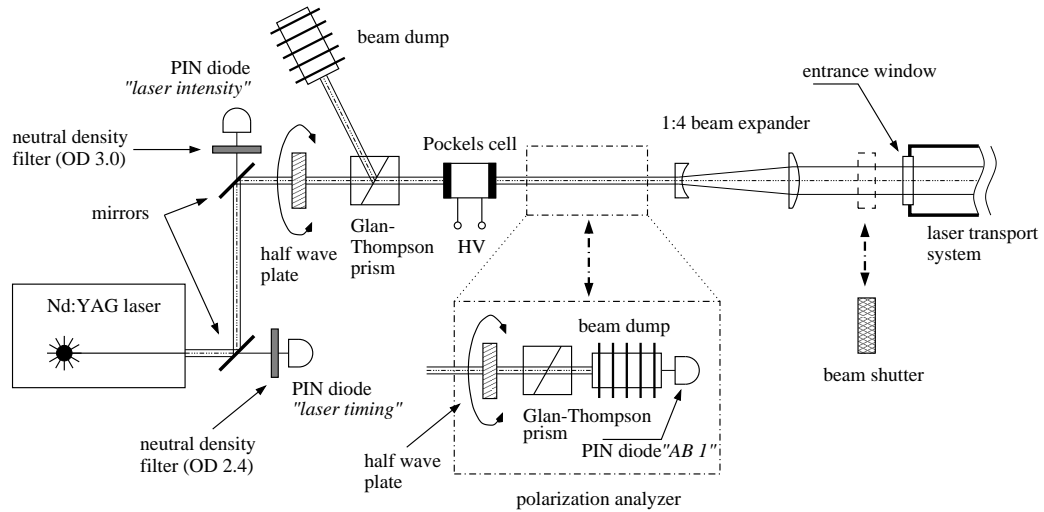
Figure 3.12: Schematic view of the LPOL laser optics in the laser hut. Taken from reference [37].
