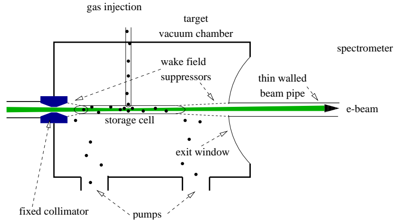
Figure 3.2: Schematic view of the HERMES target system. Taken from reference [7].
