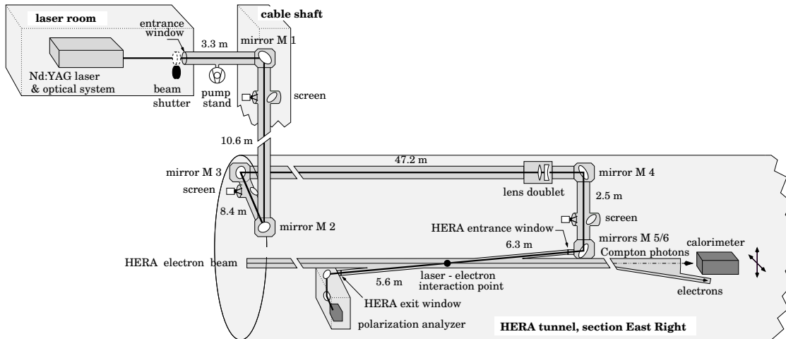
Figure 3.13: Schematic view of the LPOL laser transport system. Taken from reference [37].
