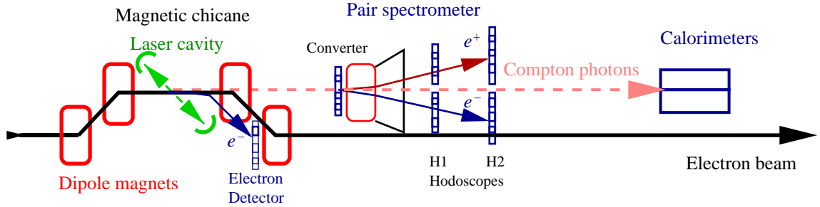
Figure 3.21: Schematic design for a hybrid Compton polarimeter at the EIC. Taken from reference [86].
