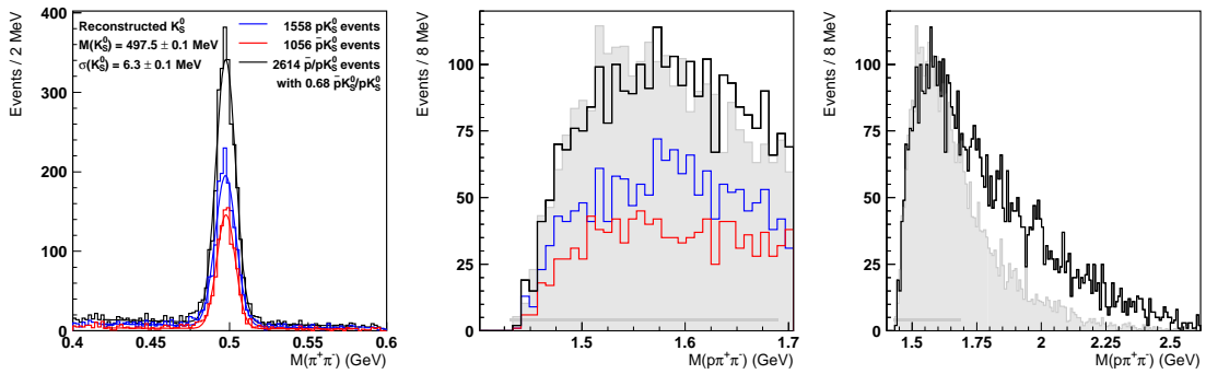
Figure 4.62: Search for the production of the exotic baryon \Theta on a high density nitrogen target during the years 1996 and 1997. For a description of the figures, refer to the text.
