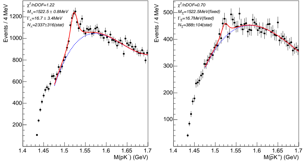
Figure 4.35: The distribution of the invariant mass M(pK) for the \Lambda(1520) \rightarrow pK^- (left panel) and \bar{\Lambda}(1520) \rightarrow \bar{p}K^+ (right panel) decay channels for the selected events in the collected data. The results of an unbinned fit with a Breit-Wigner resonance shape convolved with the Gaussian detector resolution of 4 MeV to describe the resonance peak (solid red line) and a third order polynomial for the background (dashed blue line) are superimposed. For the fit of the \bar{\Lambda}(1520) invariant mass distribution, the parameters M_{\bar{\Lambda}(1520)} and \Gamma_{\bar{\Lambda}(1520)} were fixed to the values obtained in the \Lambda(1520) fit.
