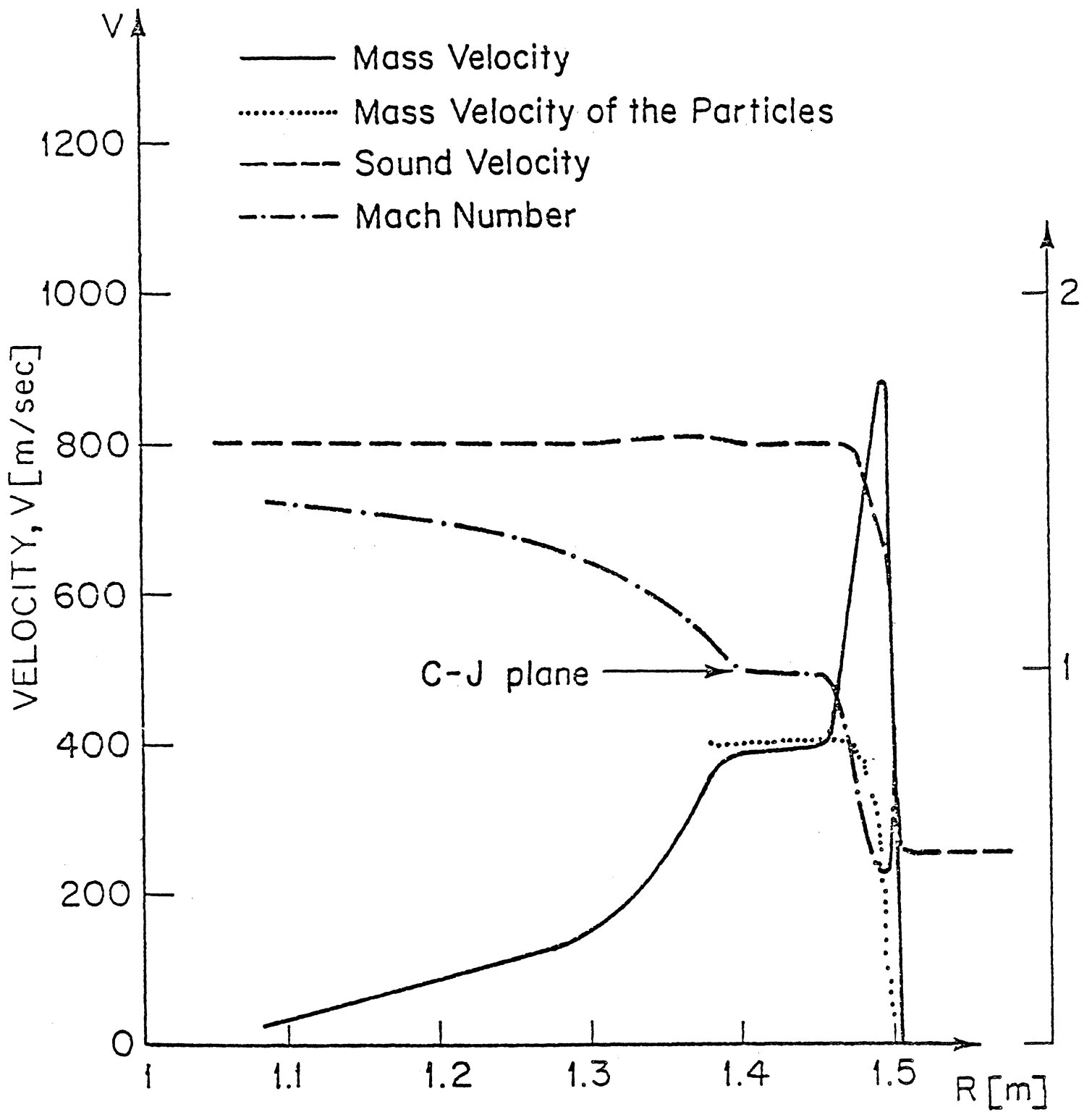
Figure 38. The structure of the detonation wave at a shock radius of 1.5 m for 80 \mu\text{m} RDX particles in air.
