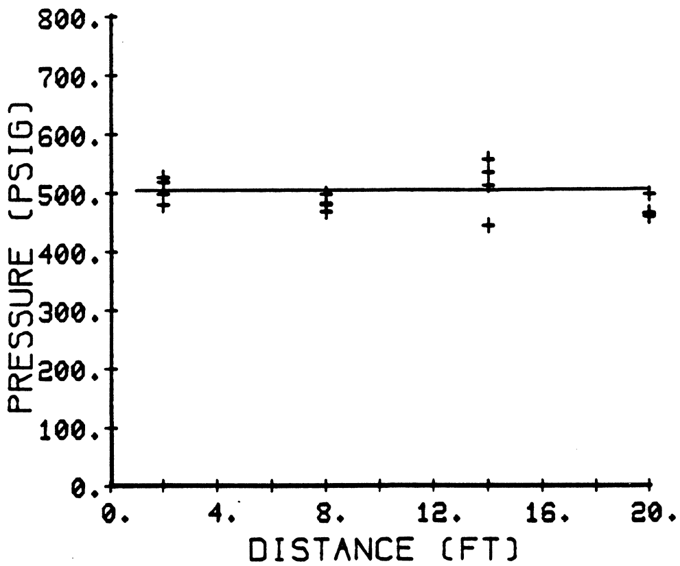
Figure 12. Wave Mach Number and Pressure RDX-A, 1300 \text{ gm/m}^3 , 88% Air, 12% \text{O}_2 , Driver Pressure 119.3 psia.
