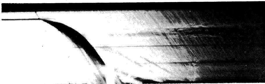
Figure 27. Ignition of 3000 \mu\text{m} Decane Droplet .
