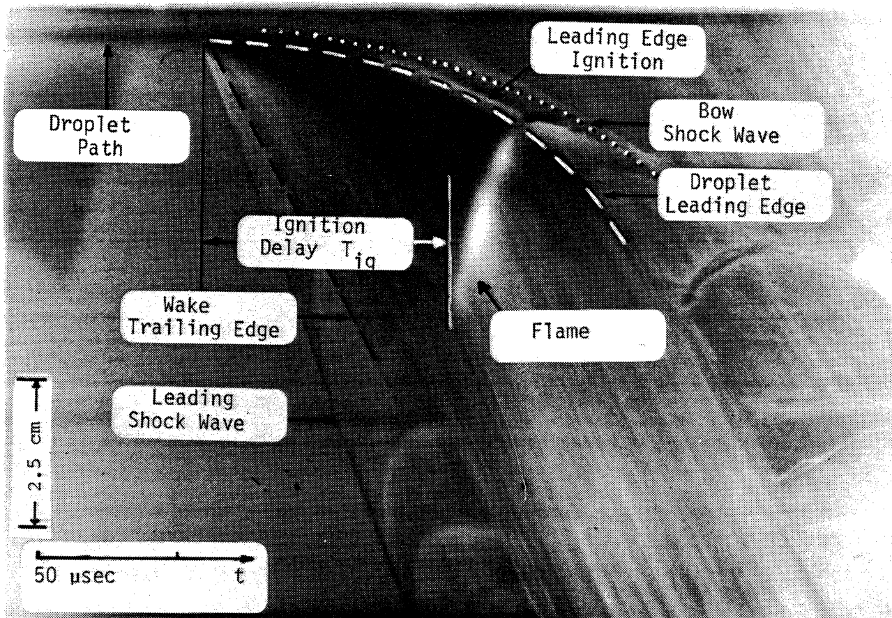
Figure 24b. Run #502, RDX-E/Decane/Cabosil Droplet, 3000 \mu\text{m} , M = 3.5 .
