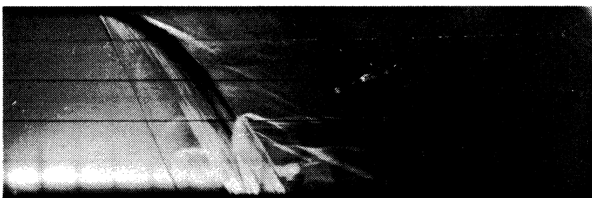
Figure 26. Ignition of 2000 \mu\text{m} Decane/RDX (60/40) Droplet.
