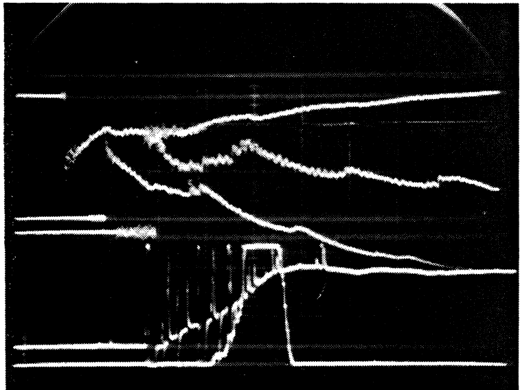
Figure 18. Light Emission and Pressure Records 0.5 msec/div. for All Traces RDX-E 1300 gm/m 3 , 88% Air, 12% O 2 , Driver Pressure 119.3 psia.
