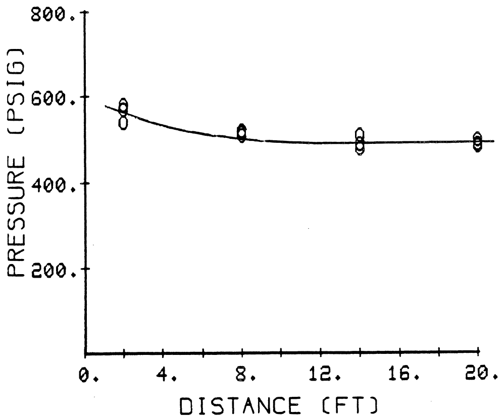
Figure 20b. Wave Mach Number and Pressure, 83% RDX-A + 17% Ammonium Perchlorate, 100% Air, 1500 \text{ gm/m}^3 , \phi = .88 , Driver Pressure 119.3 psia.
