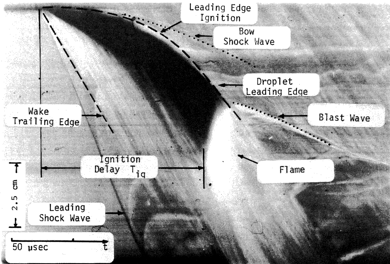
Figure 24a. Run #501, Decane/Cabosil Droplet, 3000 \mu\text{m} , M = 3.5 .
