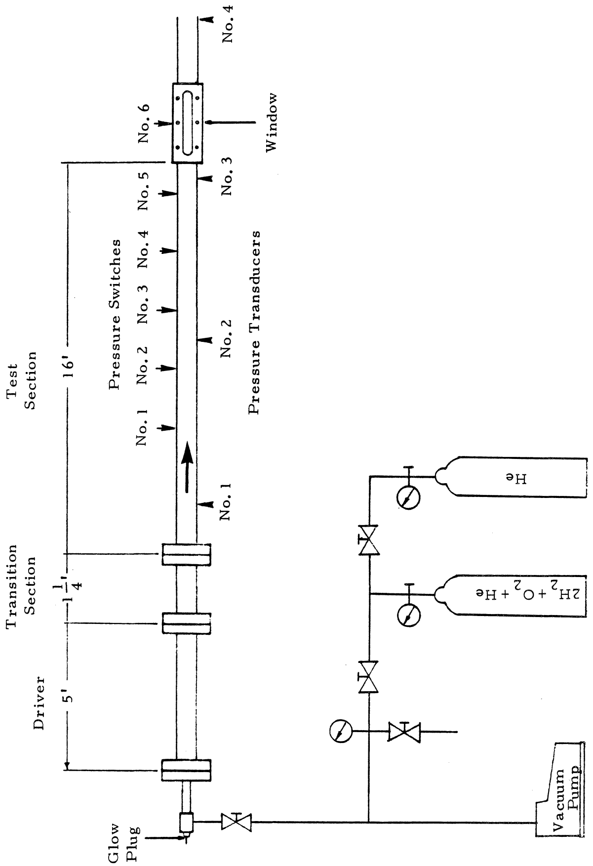
Figure 1. Schematic Diagram of Shock Tube.
