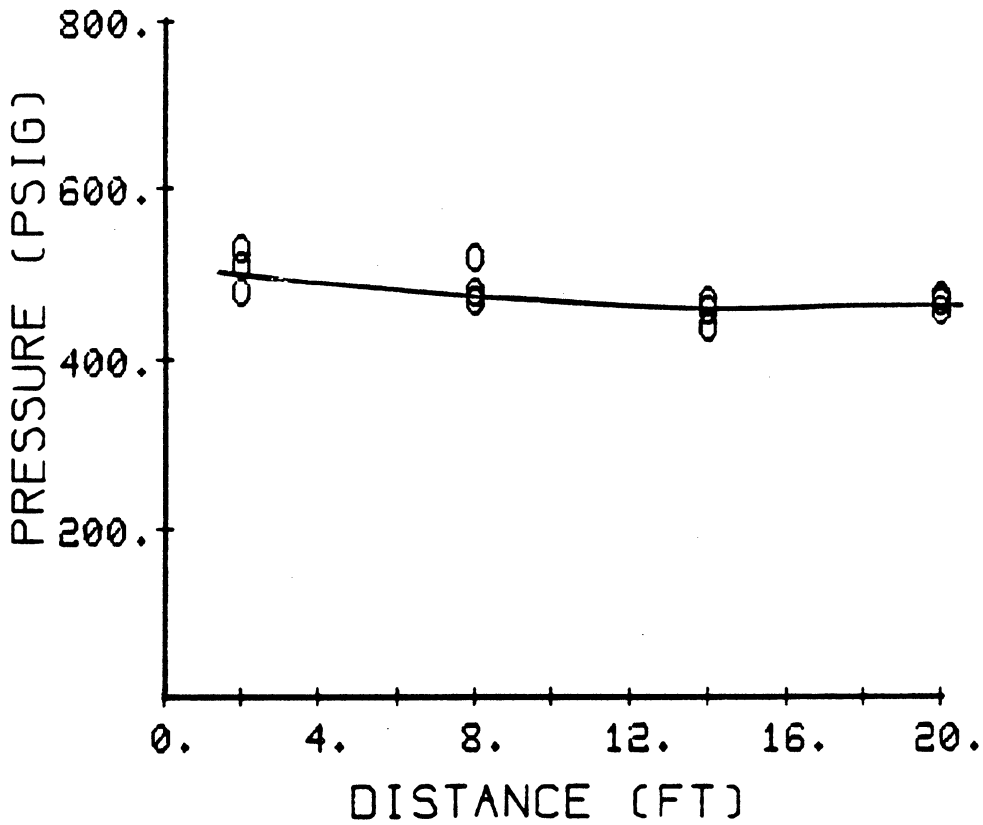
Figure 20a. Wave Mach Number and Pressure, 83%, RDX-A + 17% Ammonium Perchlorate, 100% Air, 1340 \text{ gm/m}^3 , \phi = .84 , Driver Pressure 119.3 psia.
