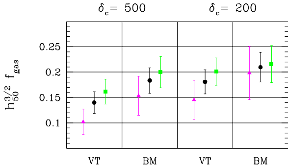
Figure 4. Bi-weight mean gas fractions at density contrasts of 500 and 200 for the VT and BM methods. Data for the full sample of 22 clusters are shown as filled circles, the low T subsample of 8 clusters as triangles, and the high T subsample of 14 clusters as filled squares. Error bars are 90% confidence limits ( 1.65\sigma ) determined from bootstrap resampling and assuming a fixed fractional error of 30% on individual cluster gas fraction estimates.
