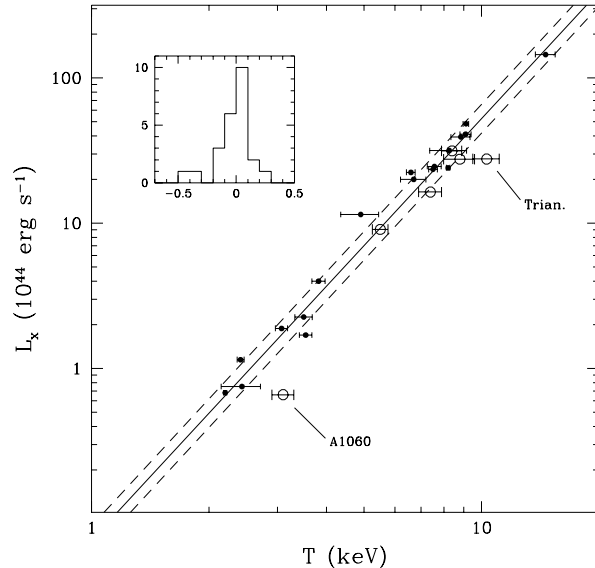
Figure 1. The luminosity–temperature relation for the 24 clusters used in this analysis. Filled circles are the homogeneous GINGA subset while open circles denote clusters with ASCA temperatures and EXOSAT, MPC, or ASCA luminosities. Error bars plotted on T are 90% confidence limits. The solid line is the best-fit relation; the dashed lines are offset by an amount equal to the rms deviation in \log(L_X) about the mean relation. The upper insert shows a histogram of the luminosity residuals (in dex), which makes apparent the two principal outliers, A1060 and Triangulum.
