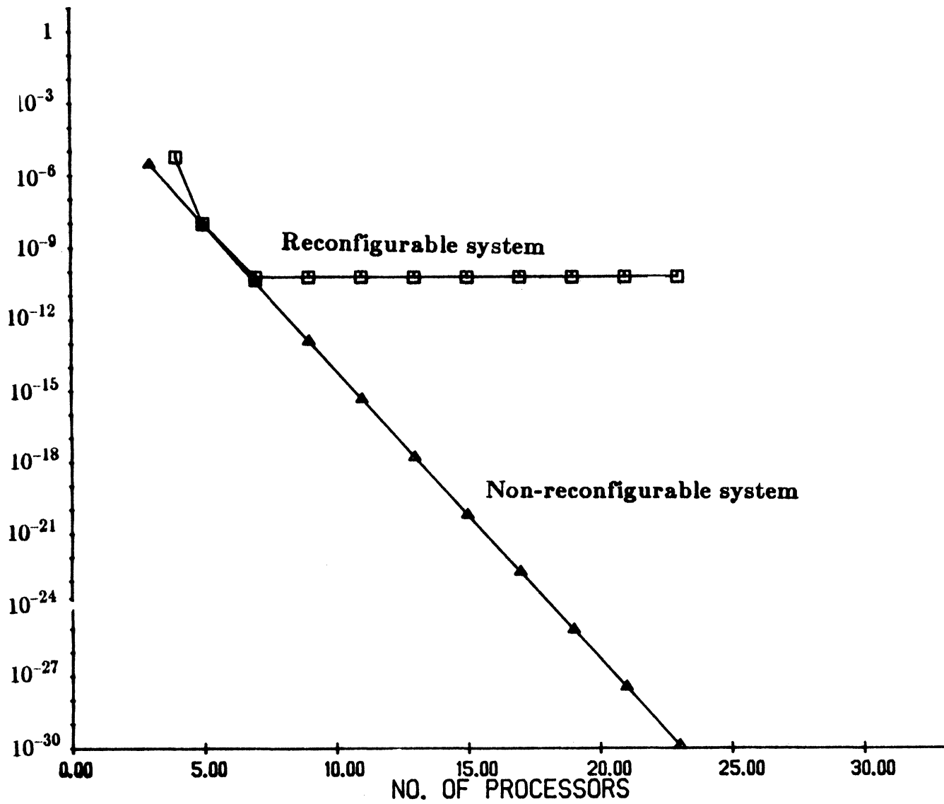
Figure 6. Comparison of reconfigurable and non-reconfigurable systems with maximum reconfigurable cluster size = 4, hard deadline = 100 milli-seconds, task execution time = 70 milli-seconds, and mission lifetime = 10^4 seconds.
