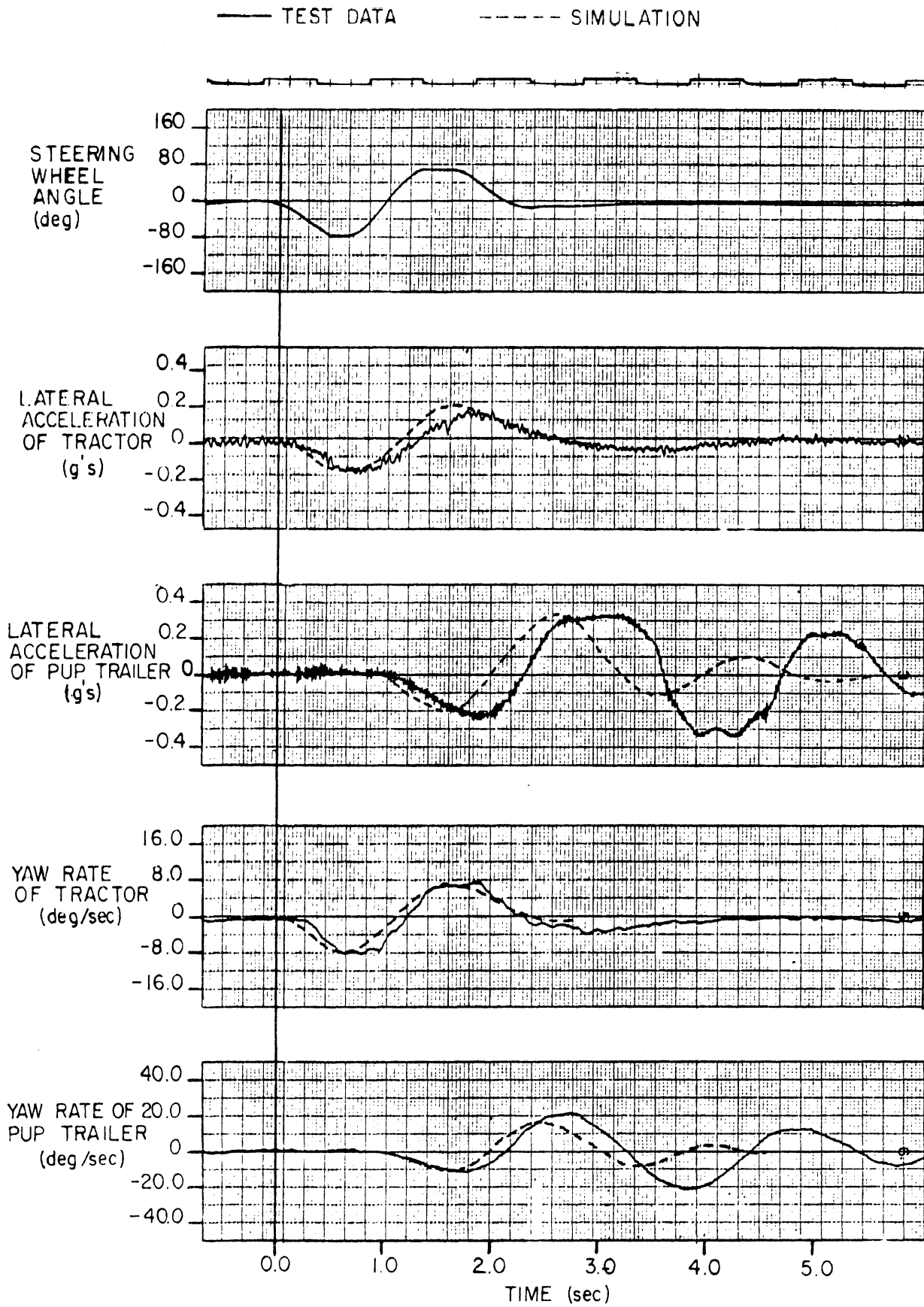
FIGURE A-19. FULLY LOADED 55' DOUBLE TANKER - FORWARD SPEED 38.5 mph
