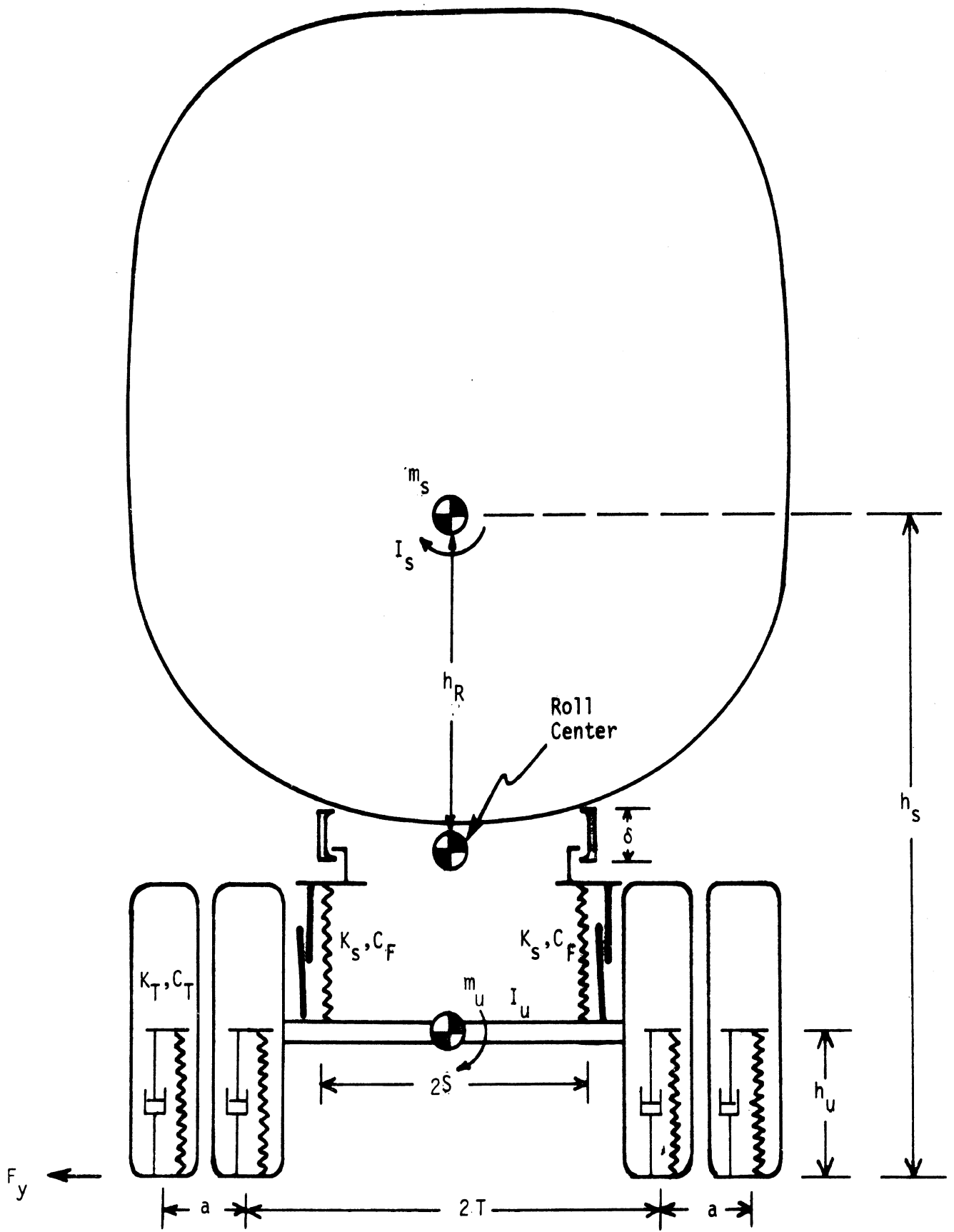
Figure B.2. The dynamic rollover model.
