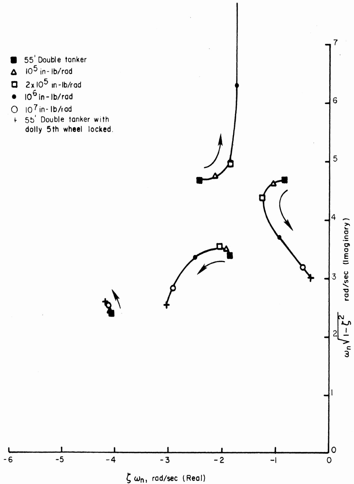
FIGURE A-15. EFFECT OF ADDING A SPRING AT THE DOLLY KINGPIN
