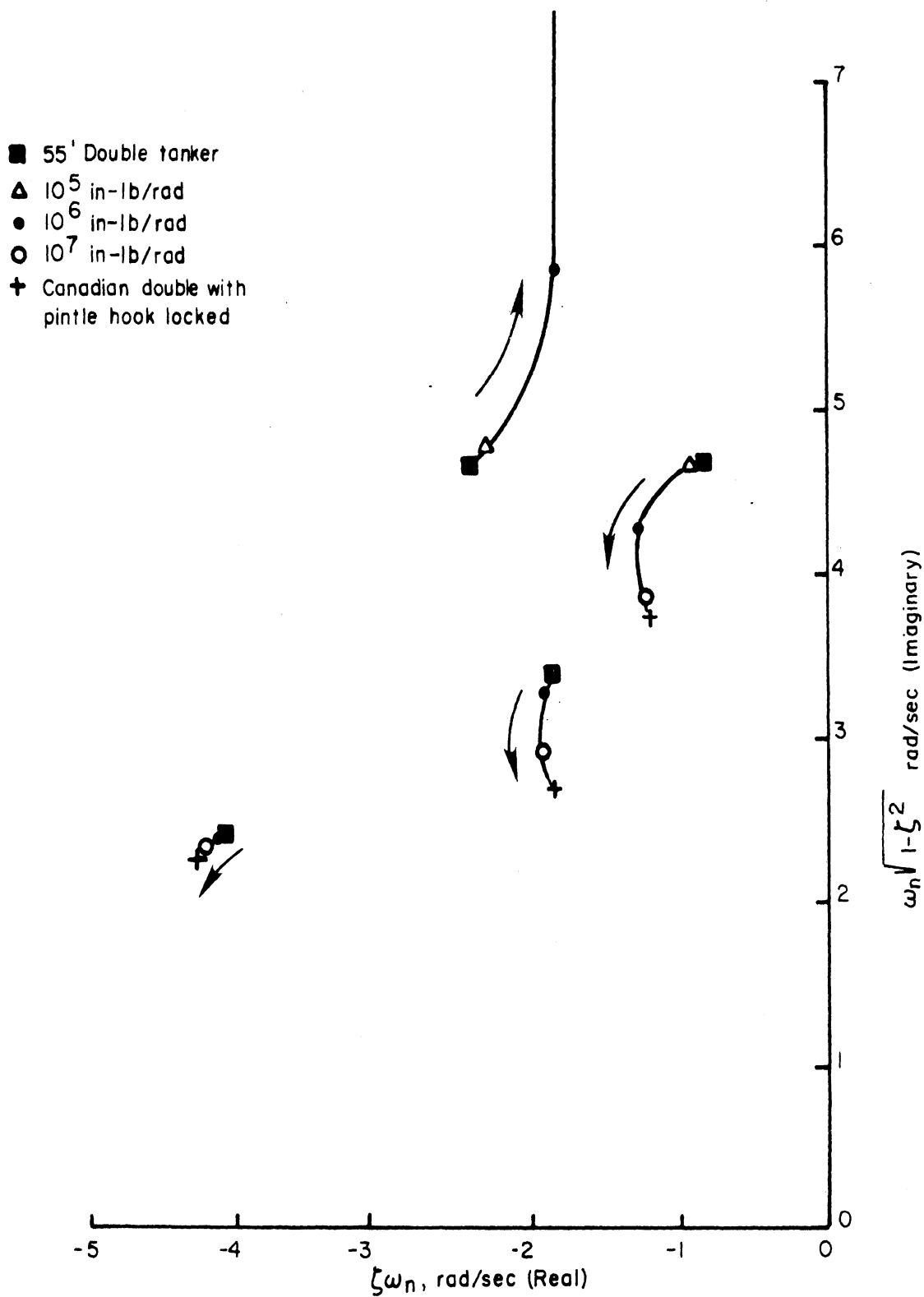
FIGURE A-14. EFFECT OF ADDING A SPRING AT THE PINTLE HOOK
