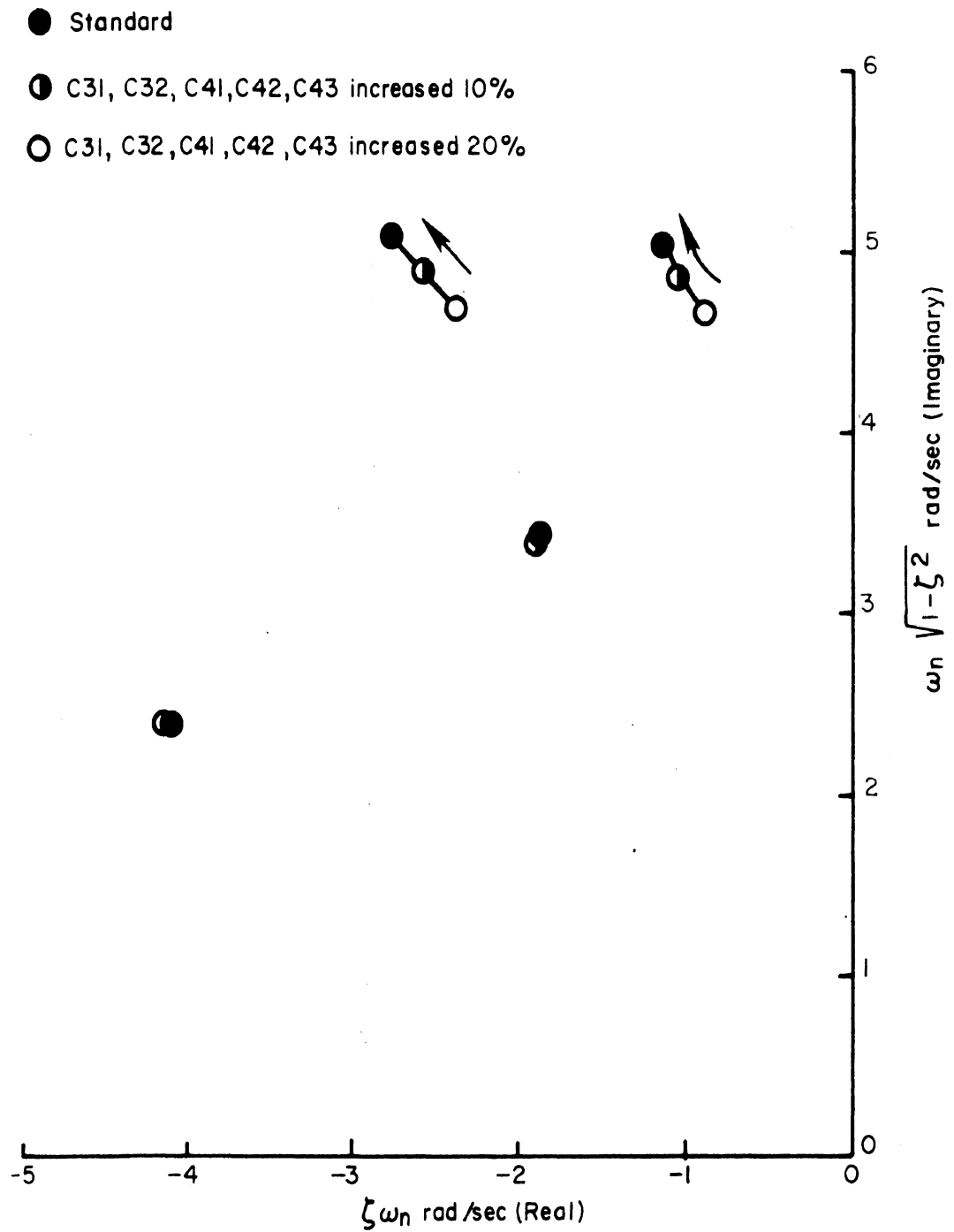
FIGURE A-II. EFFECT OF INCREASE IN CORNERING STIFFNESS OF PUP AND DOLLY TIRES
