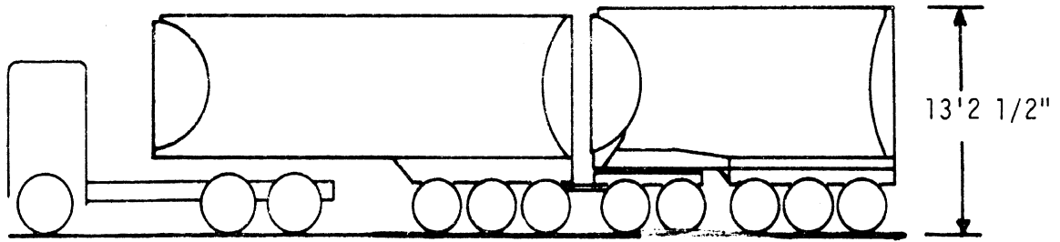
Baseline 11-Axle Michigan Double Tanker
