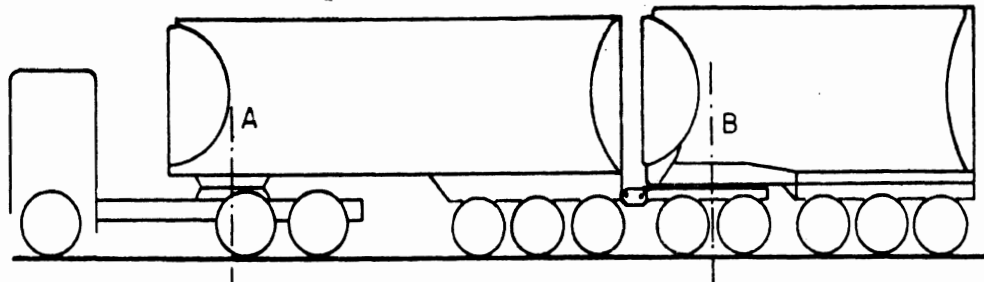
MODIFIED 11 AXLE DOUBLE BOTTOM TANKER WITH RIGID PINTLE HOOK (3 COMPONENT VEHICLE)
