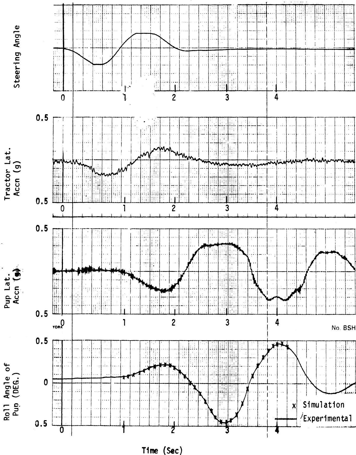
Figure B.8. Comparison of experimental and simulation roll angles for the double-bottom pup trailer.
