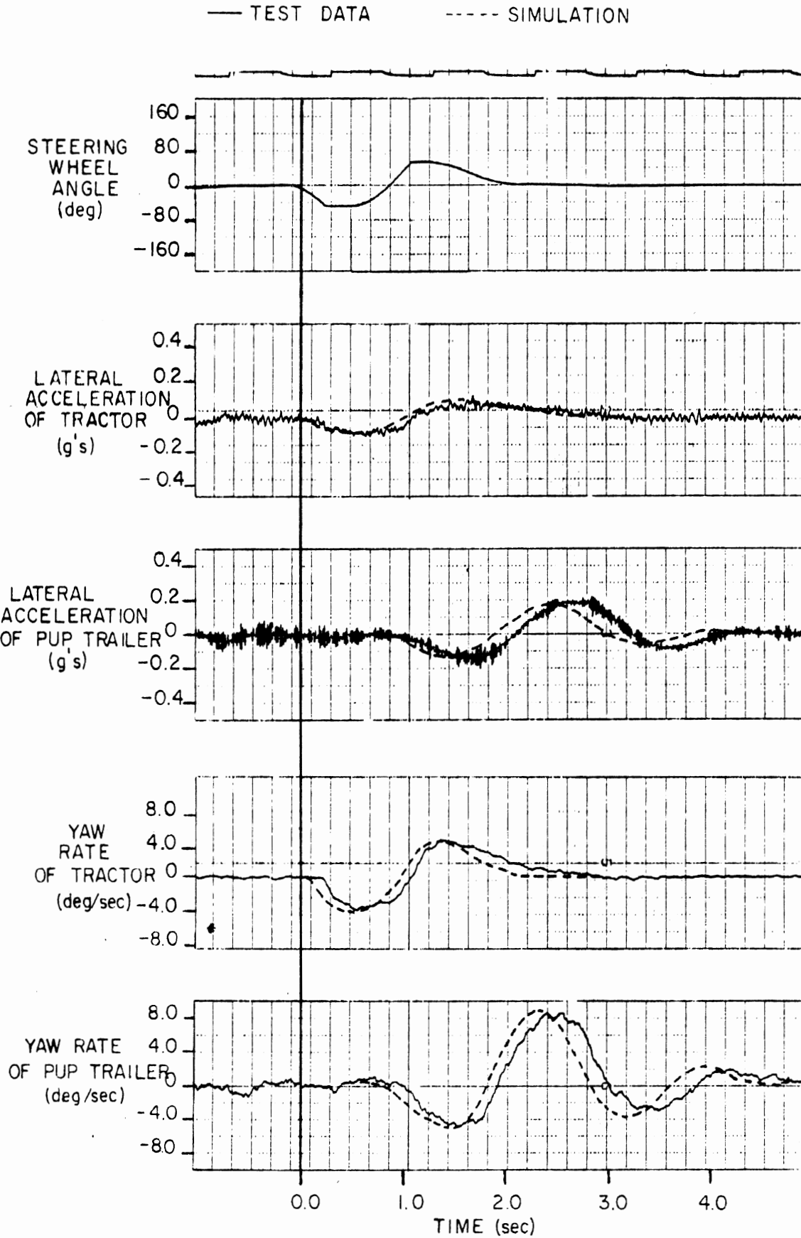
FIGURE A-18. FULLY LOADED 55' DOUBLE TANKER - FORWARD SPEED 39 mph
