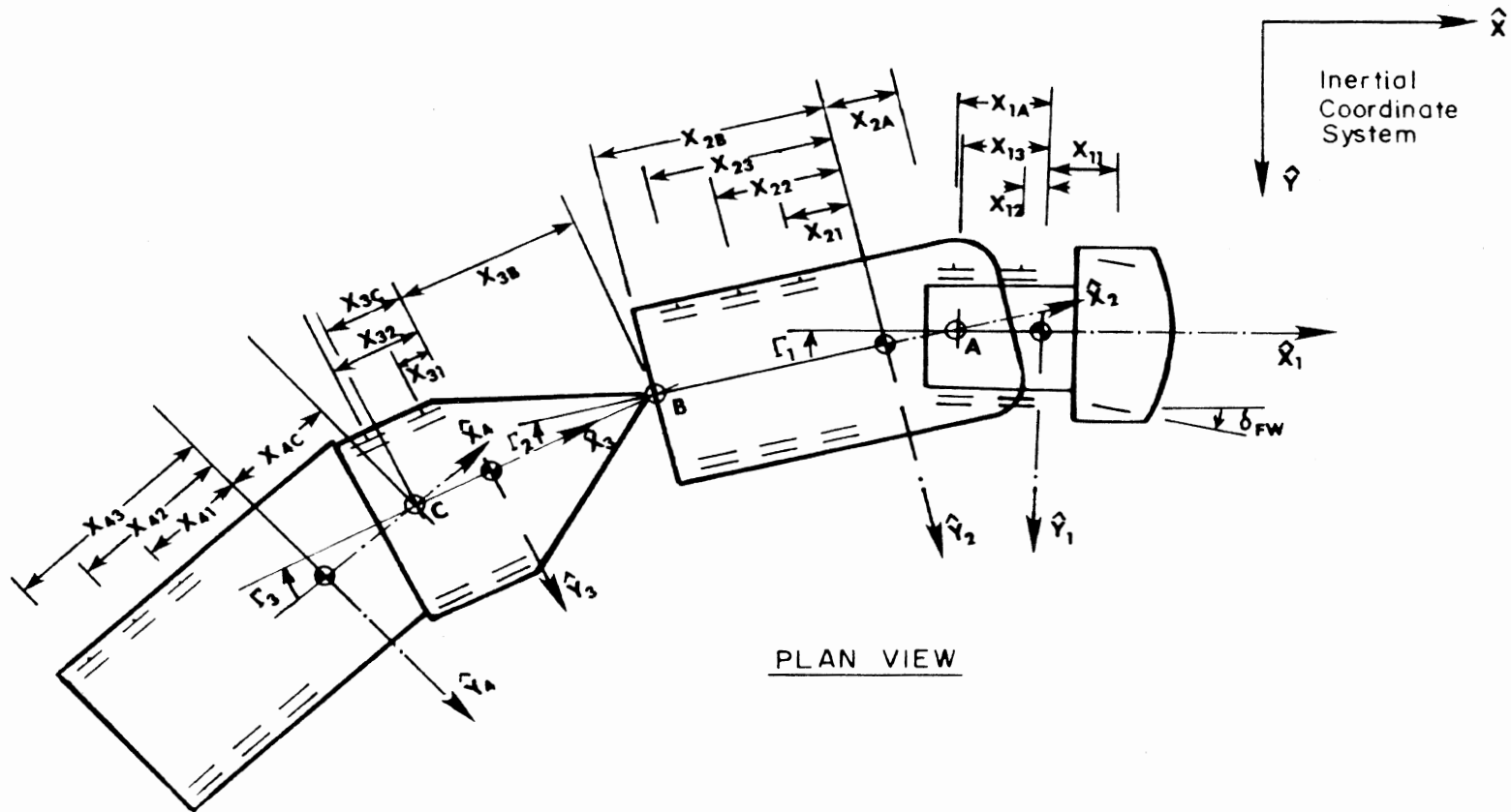
FIGURE A-3. DEFINITION OF COORDINATE SYSTEM AND IMPORTANT DIMENSIONS OF A DOUBLE TANKER
