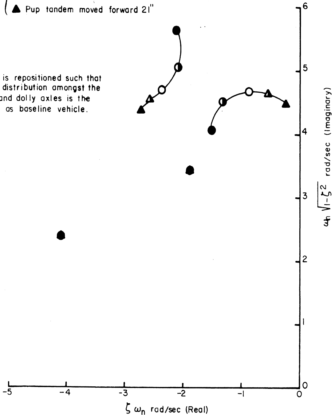
FIGURE A-9. EFFECT OF CHANGE IN PUP TANDEM AXLE LOCATION
