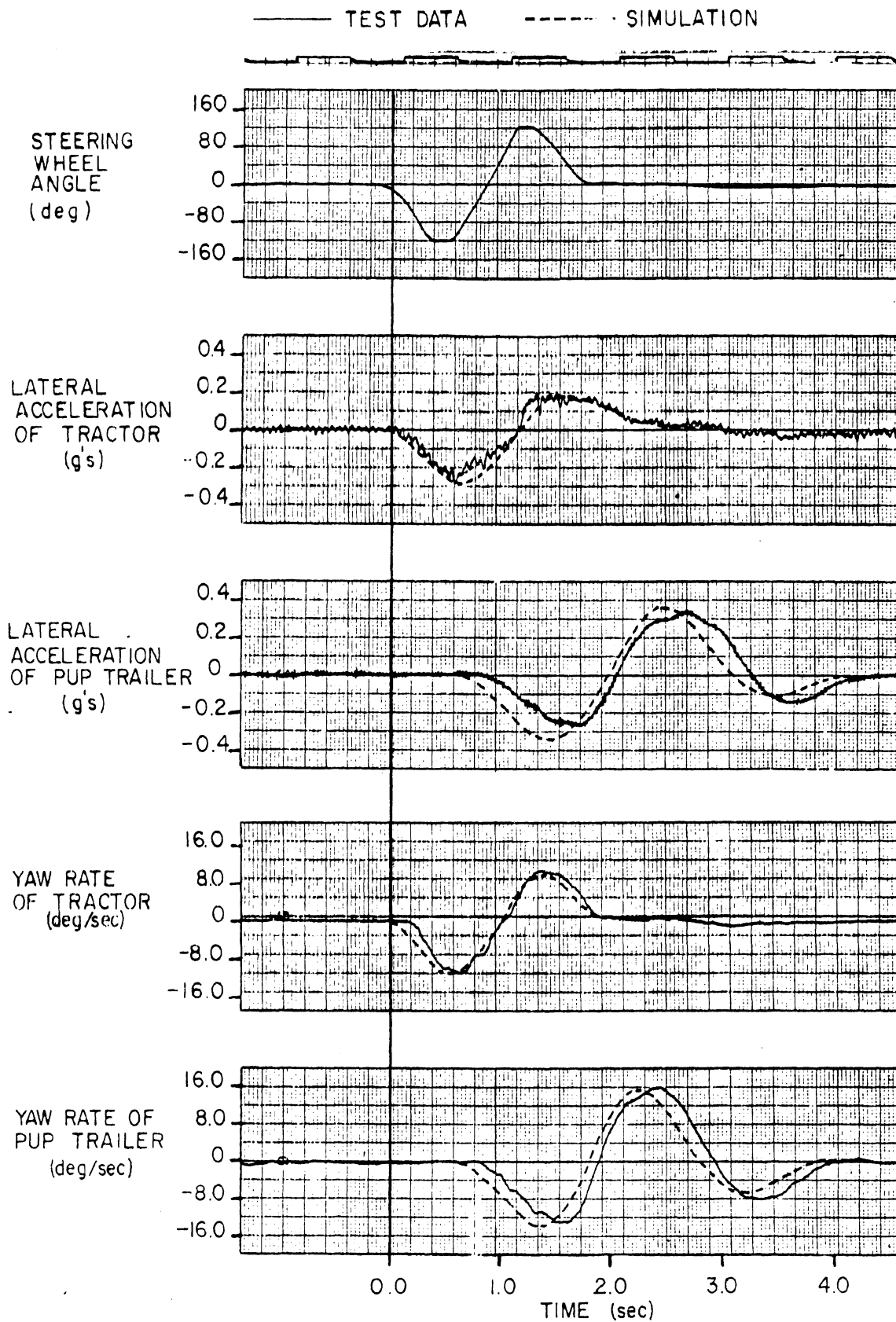
FIGURE A-20. FULLY LOADED MODIFIED 55' DOUBLE TANKER - FORWARD SPEED 40mph
