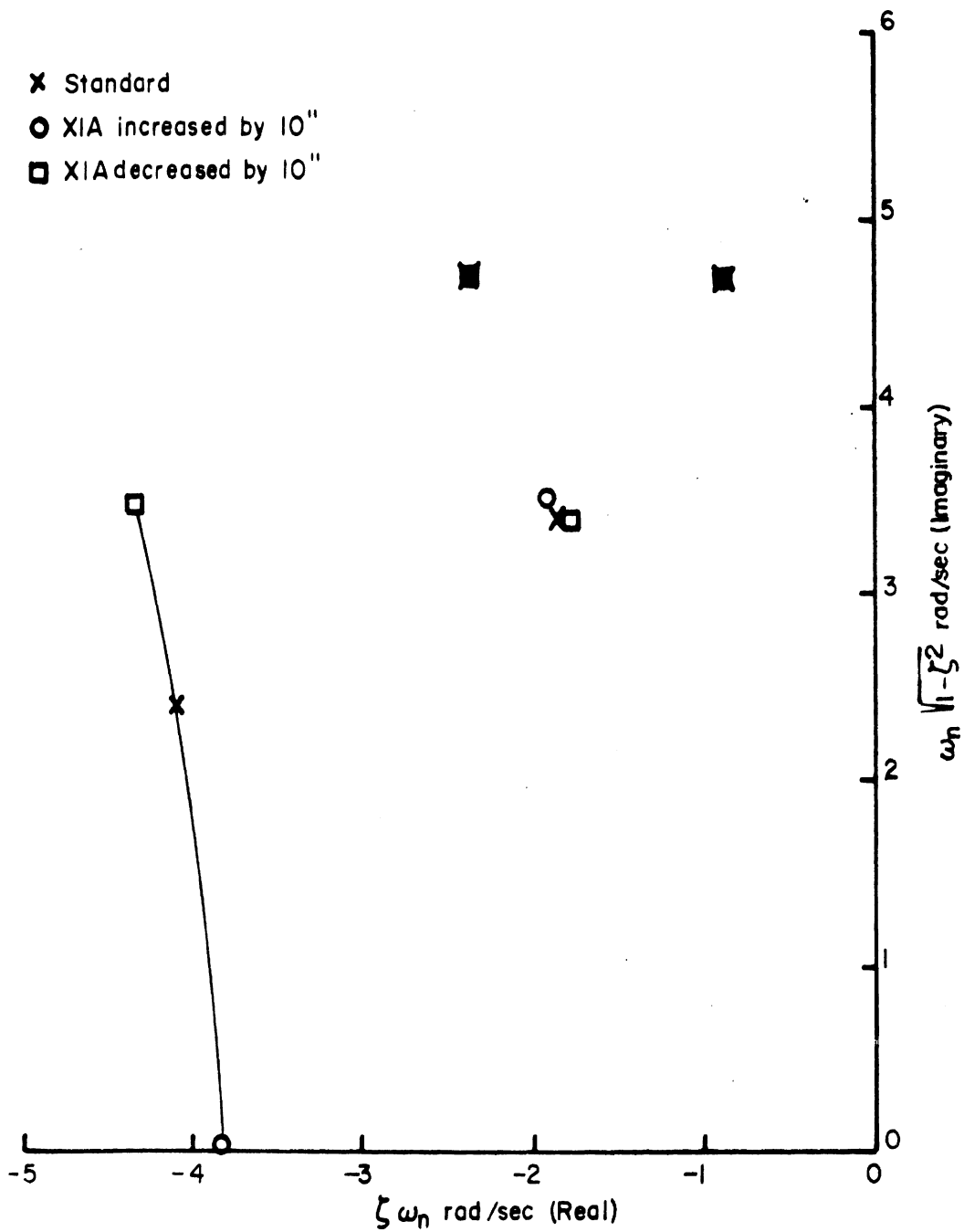
FIGURE A-10. EFFECT OF CHANGE IN TRACTOR 5th WHEEL LOCATION
