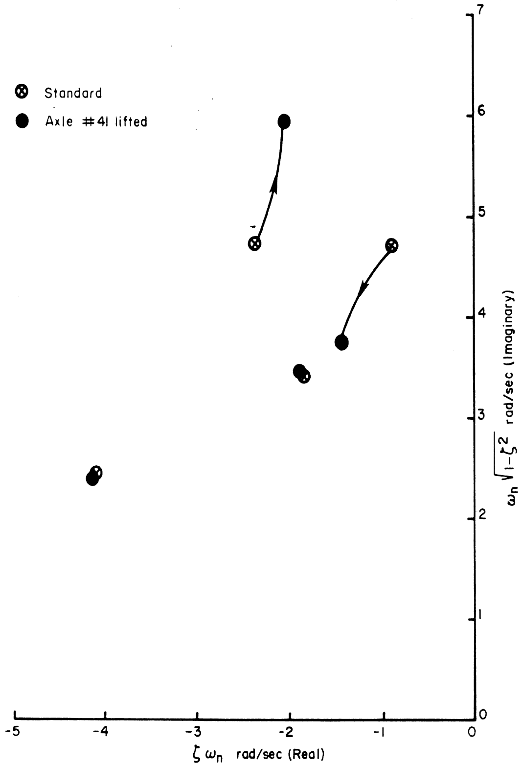
FIGURE A-12. EFFECT OF LIFTING AN AXLE
