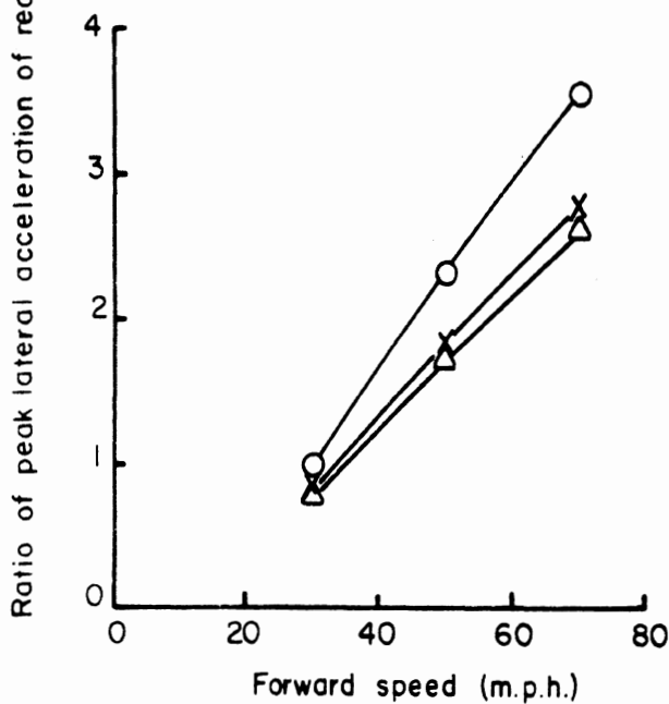
FIGURE A-17. PEAK LATERAL ACCELERATION RATIOS OF FOUR ARTICULATED VEHICLE CONFIGURATIONS DURING 2 SECOND LANE CHANGE MANEUVER
