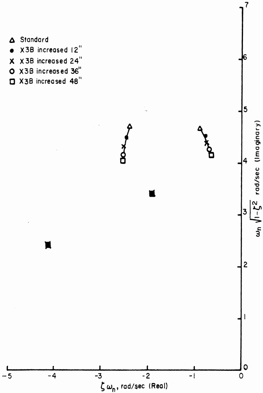
FIGURE A-13. EFFECT OF INCREASE IN TONGUE LENGTH
