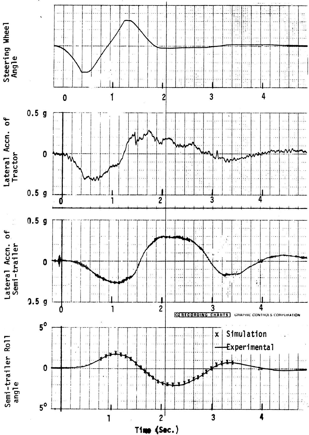
Figure B.7. Comparison of experimental and simulation roll angles for the short single tanker.
