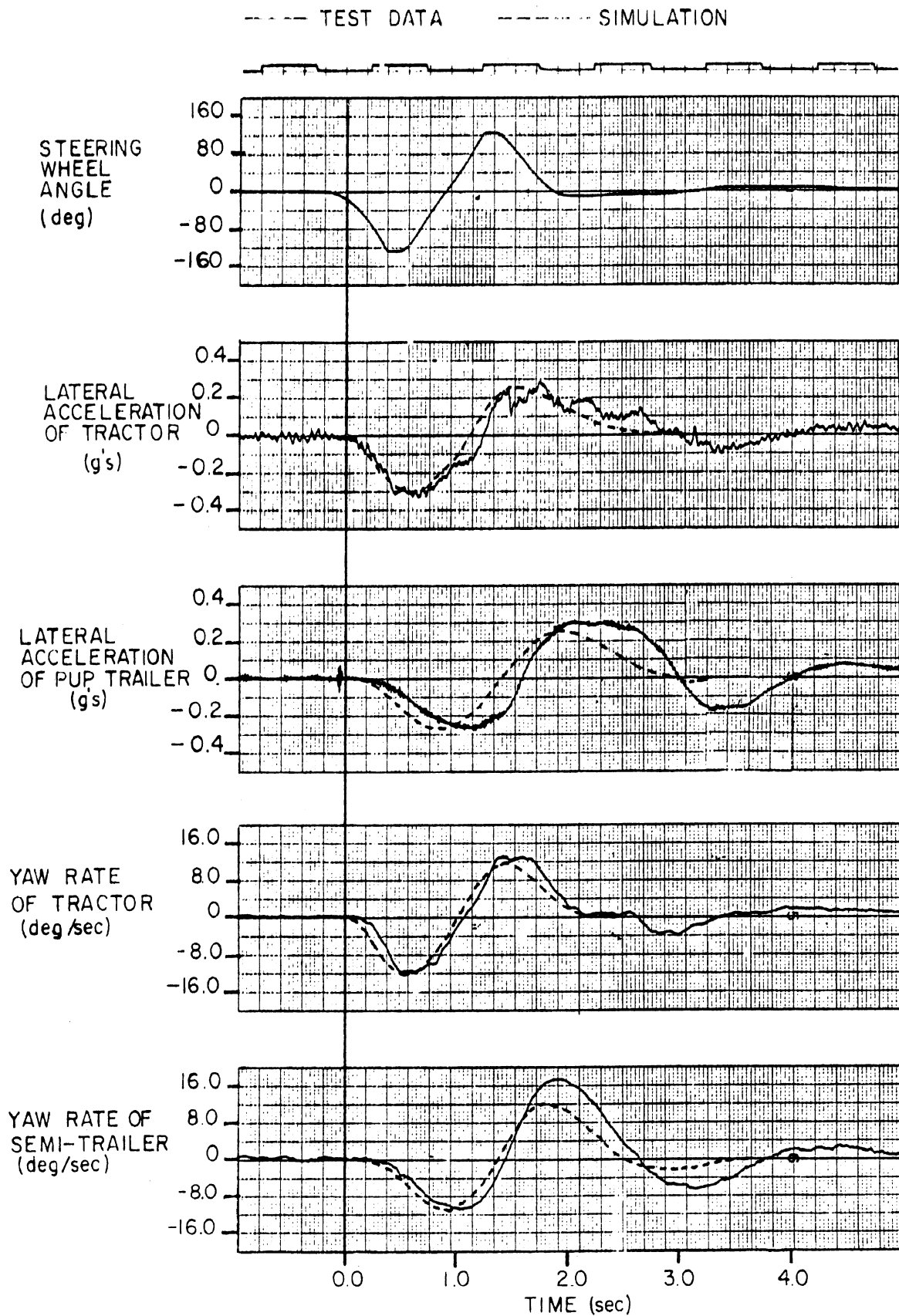
FIGURE A-22 FULLY LOADED TRACTOR SEMI-TRAILER, FORWARD SPEED 44mph
