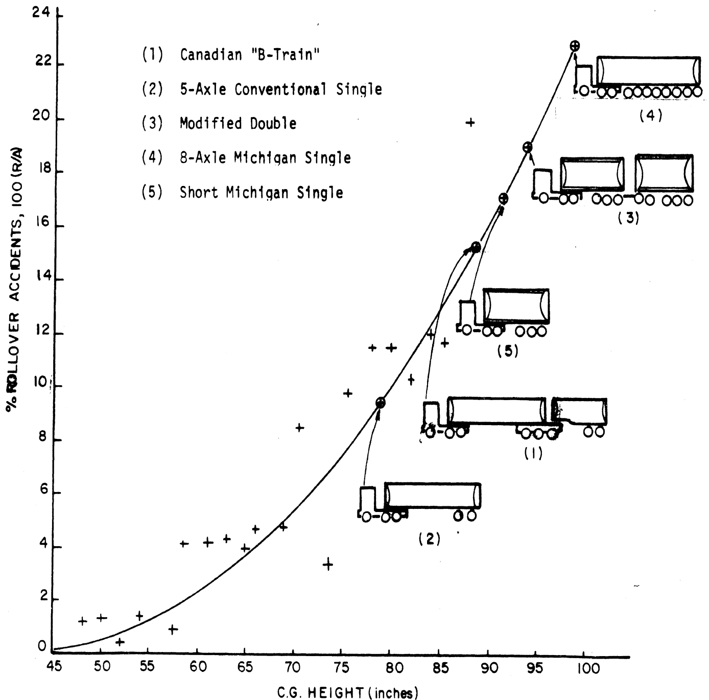
Figure F.1 Percentage Rollover Accidents, as related to center of gravity height:
