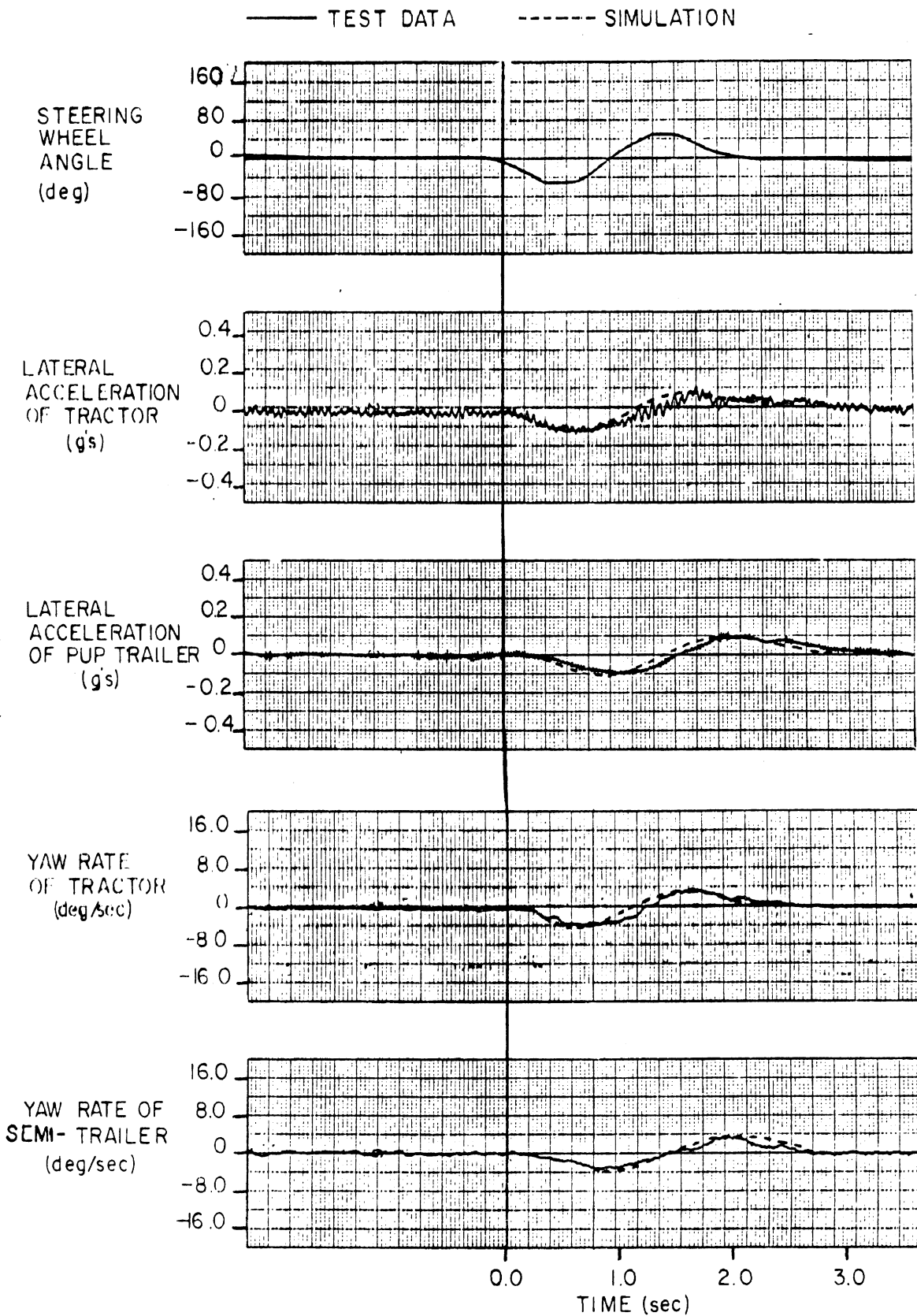
FIGURE A-21. FULLY LOADED TRACTOR SEMI-TRAILER - FORWARD SPEED 45 mph
