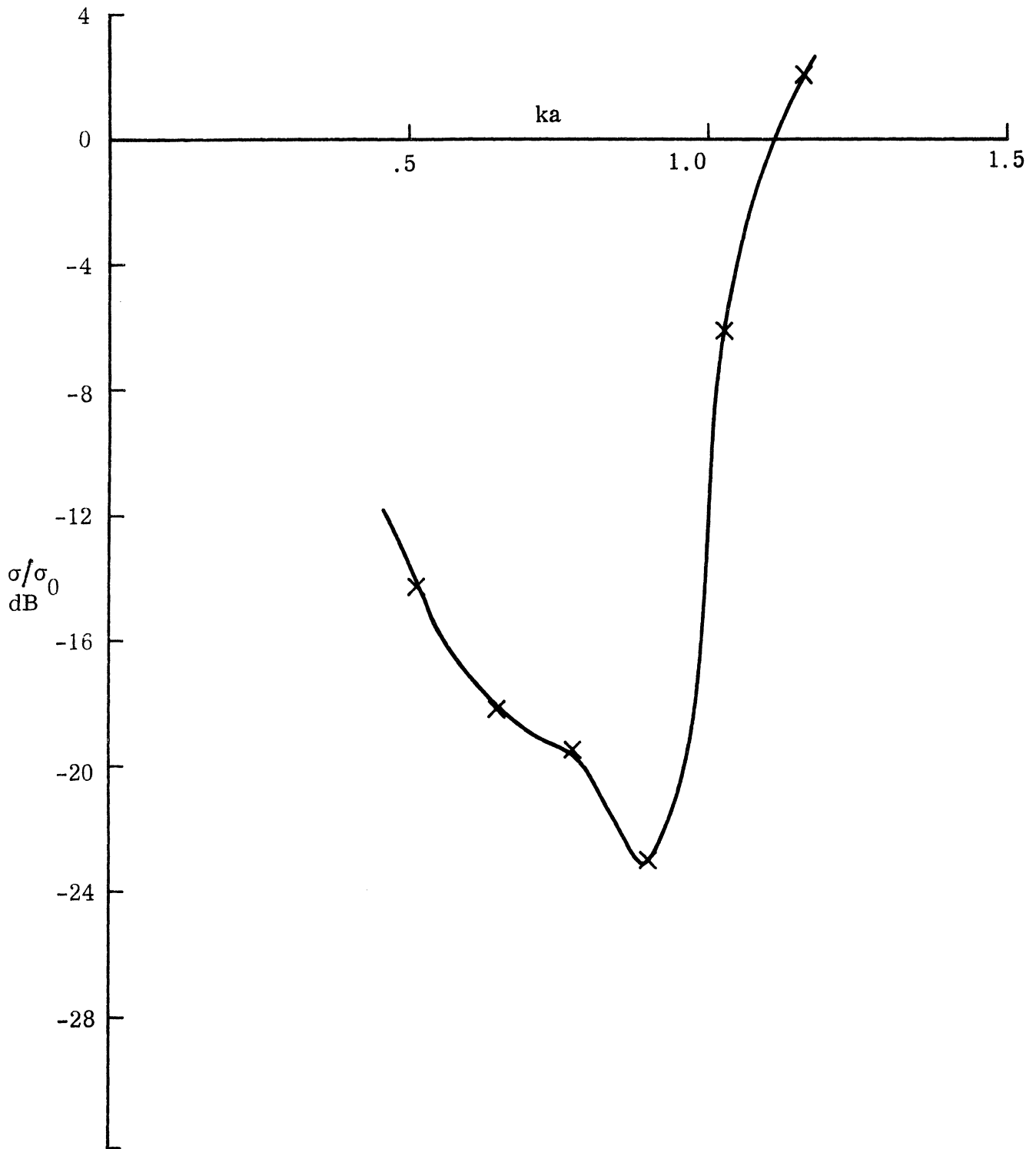
FIG. 5-5: Calculated Cross-Section Reduction for Measured Impedance Values.
