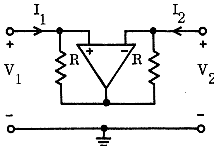
FIG. 4-9: Operational Amplifier NIC.
