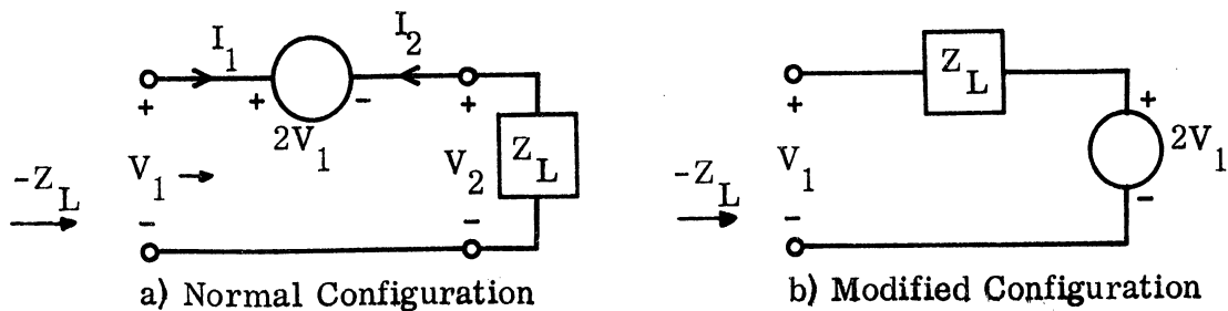
FIG. 4-7: Voltage Amplifier NIC.
