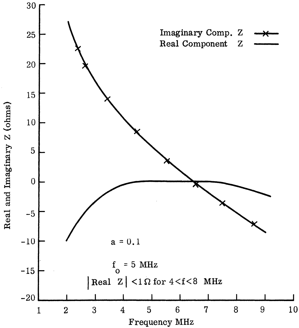
FIG. 5-4: NIC and Load Bridge Measured Impedance.
