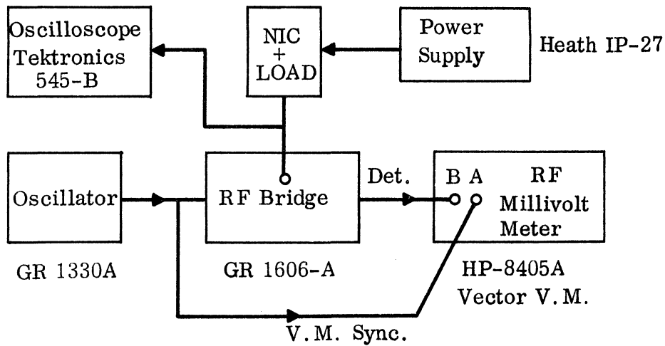
FIG. 5-1: RF Bridge Z Measurement. (voltmeter null detector)
