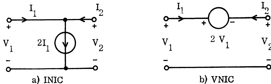
FIG. 4-2: Basic NIC Realizations.
