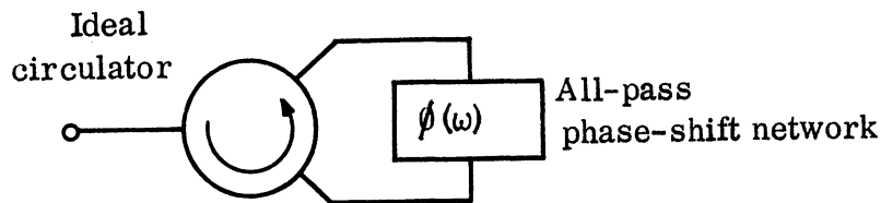
FIG. 4-1: Reflection Coefficient Realization.
