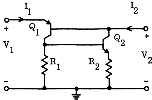
FIG. 4-10: Yanagisawa NIC.
