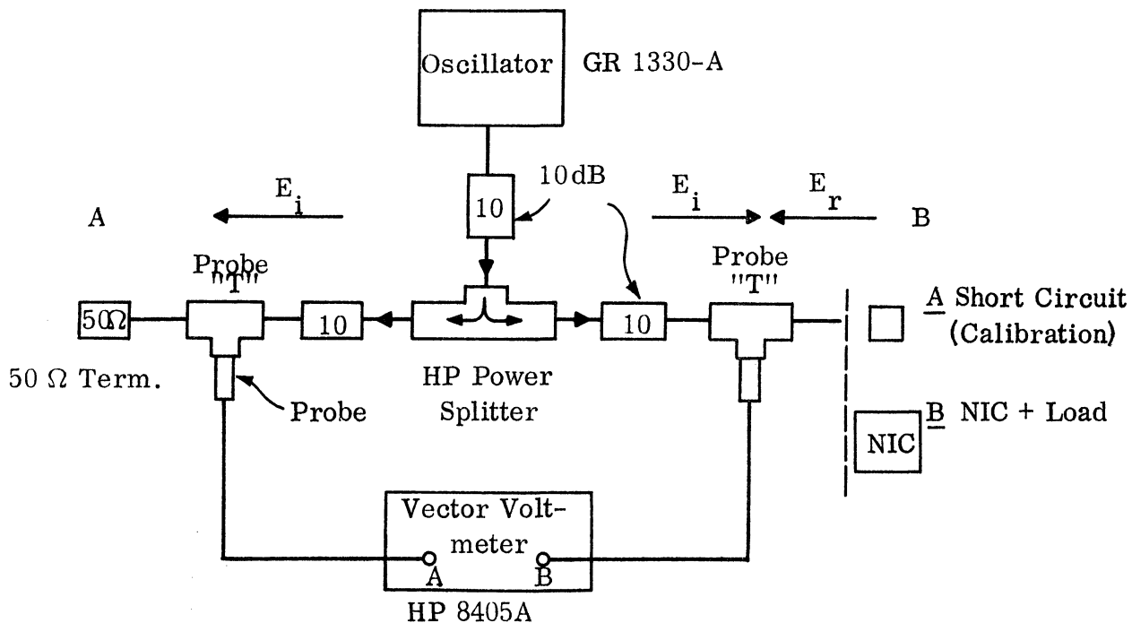
FIG. 5-1: RF Bridge Z Measurement. (voltmeter null detector)
