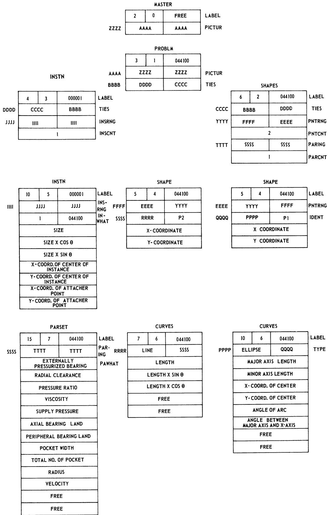
FIGURE 4-1 GENERAL DATA STRUCTURE OF THE LING SYSTEM.
