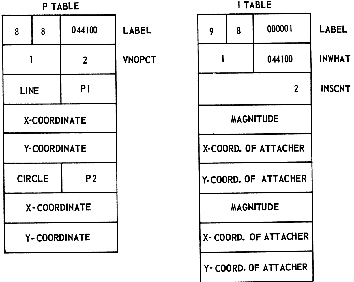
FIGURE 4-2 CONDENSED DATA STRUCTURE
