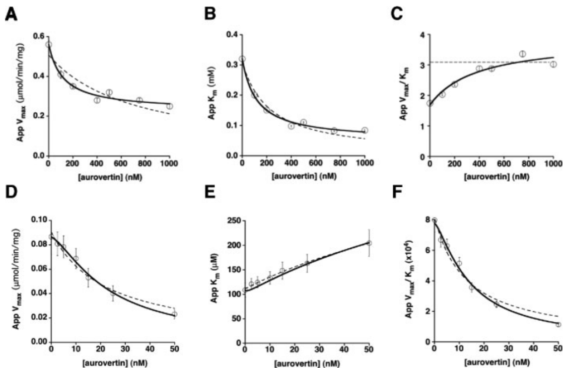
FIGURE 1 Aurovertin inhibition of the F_1F_0 -ATPase in bovine SMPs. ATP hydrolysis: Aurovertin decreases both the apparent V_{\max} (A) and K_m (B), and increases the apparent V_{\max}/K_m (C). The plots of the kinetic parameters in panels A, B, and C were fit using either Eq. (1) for a purely uncompetitive inhibitor (dotted lines) or Eqs. (2)–(4) for a mixed inhibitor with residual activity of the enzyme-substrate-inhibitor (ESI) complex (solid lines), as described in Materials and Methods. Fits shown are with all n values set equal to 1. ATP synthesis: Aurovertin decreases both the apparent V_{\max} (D) and V_{\max}/K_m (F), and increases the apparent K_m (E). The V_{\max} and V_{\max}/K_m plots were fit using Eq. (1) and the plot of K_m was fit using Eq. (3), consistent with mixed inhibition. The fits are shown with n_{(E)} and n_{(ES)} both set equal to 1 (dotted lines), and with n_{(E)} = 2 , n_{(ES)} = 1 (solid lines).
