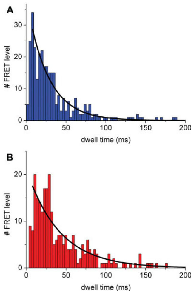
FIGURE 5 Dwell time histograms of single FRET-labeled F_1F_o -ATPase from E. coli in liposomes showing aurovertin inhibition of ATP hydrolysis. FRET levels were assigned manually and dwell times binned to 3 ms. (A) Dwell time histogram in the presence of 1 mM ATP; (B) dwell time histogram in the presence of 20 \mu\text{M} aurovertin and 1 mM ATP. Black lines are monoexponential decay fittings.
