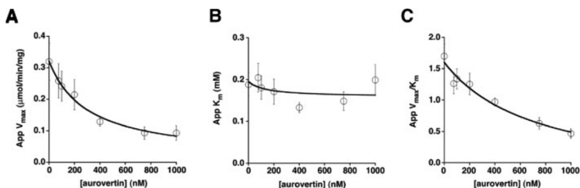
FIGURE 3 Aurovertin inhibition of ATP hydrolysis in E. coli membranes. Aurovertin decreases the apparent V_{\max} (A) and V_{\max}/K_m (C), while the apparent K_m remains relatively constant (B). These data were fit using Eqs. (2)–(4) for a mixed inhibitor with residual activity of ESI, as described in Materials and Methods.
