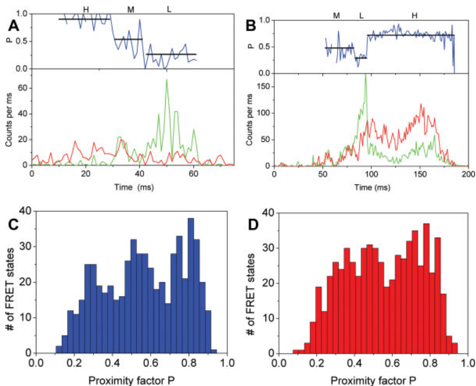
FIGURE 4 Photon bursts and proximity factor distributions of single FRET-labeled F_1F_o -ATPases from E. coli in liposomes in the presence of 1 mM ATP (A) and 1 mM ATP with 20 \mu M aurovertin (B). The F_1F_o -ATPase was labeled with rhodamine 110 at the rotating \gamma subunit and with Cy5-bismaleimide cross-linking the static b_2 subunits. Background-corrected fluorescence time trajectories of FRET donor ( I_D , green) and acceptor ( I_A , red) are shown in the lower panel and the corresponding proximity factor P = I_A/(I_D + I_A) as blue trace in the upper panel. The sequential transitions of three proximity factor levels within the burst indicate stepwise rotation of \gamma . The intermediate FRET level (M) in the absence of aurovertin has a dwell time of 10 ms (A). The intermediate FRET level (L) in the presence of aurovertin has a dwell time of 15 ms (B). (C, D) Distribution of proximity factors of FRET-labeled F_1F_o -ATPases upon ATP hydrolysis. (C) Distribution of FRET levels of rotating F_1F_o -ATPase in the presence of 1 mM ATP showing three or more levels within single photon bursts (556 levels in total). (D) Distribution of FRET levels in the presence of ATP plus 20 \mu M aurovertin (617 levels in total). Thresholds of minimal FRET level dwells of 10 ms, minimal mean photon count rates of 5 counts per ms, maximal peak intensities of 150 counts per ms, and fluctuations of the proximity factor P of less than 0.15 in each FRET level were applied.
