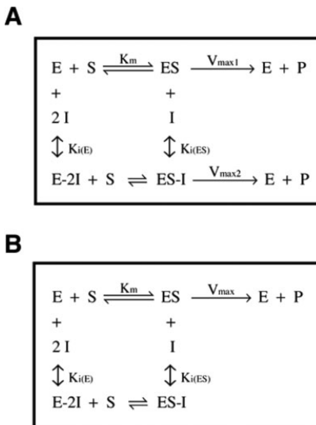
FIGURE 2 Proposed models for inhibition of the bovine F 1 F 0 -ATPase by aurovertin. (A) ATP hydrolysis. (B) ATP synthesis.
