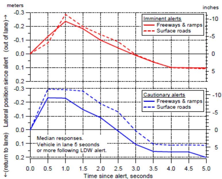
Figure 6. QL3 sample method of illustrating the affects of the integrated crash warning system on extent and duration of lane departures.
