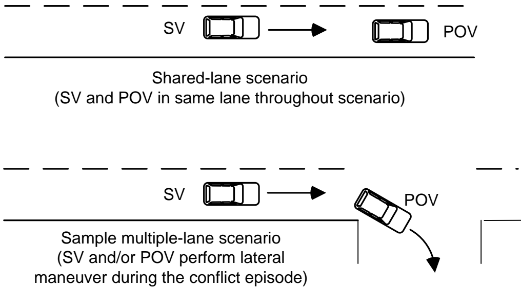
Figure 13. QF2 Concept drawing: Actual deceleration required to maintain a headway buffer
