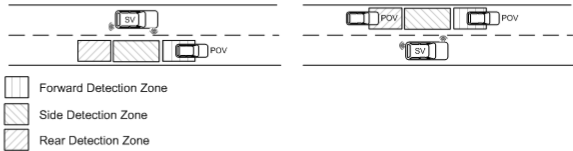
Figure 9. QL6 Concept drawing: Adjacent zone to determine the location of adjacent vehicles relative to the subject vehicle for LCM warnings.
