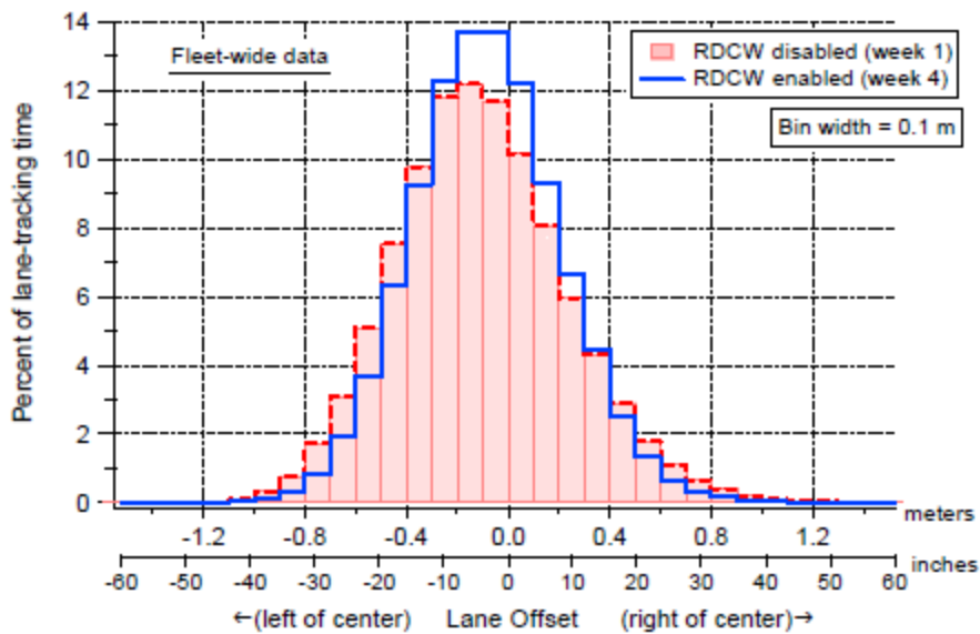
Figure 2. QL1 sample method of illustrating the affects of the integrated crash warning system on lateral offset.
