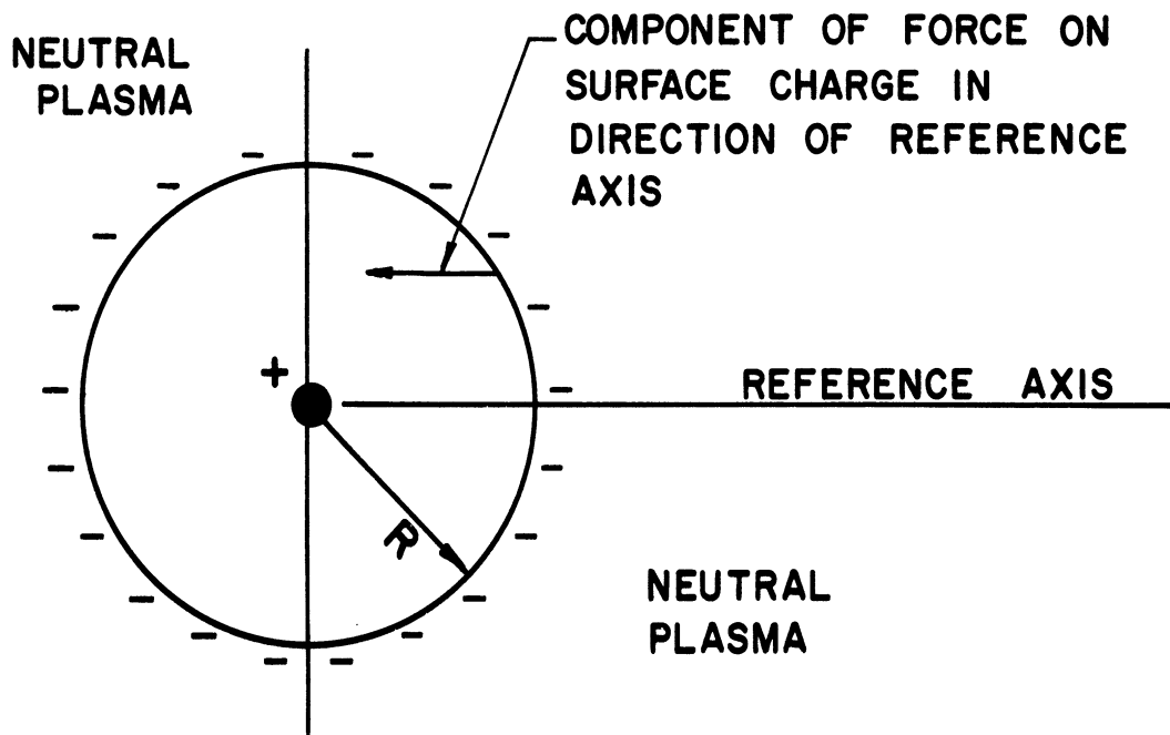
Figure 7. Calculation of internal pressure within the plasma.
