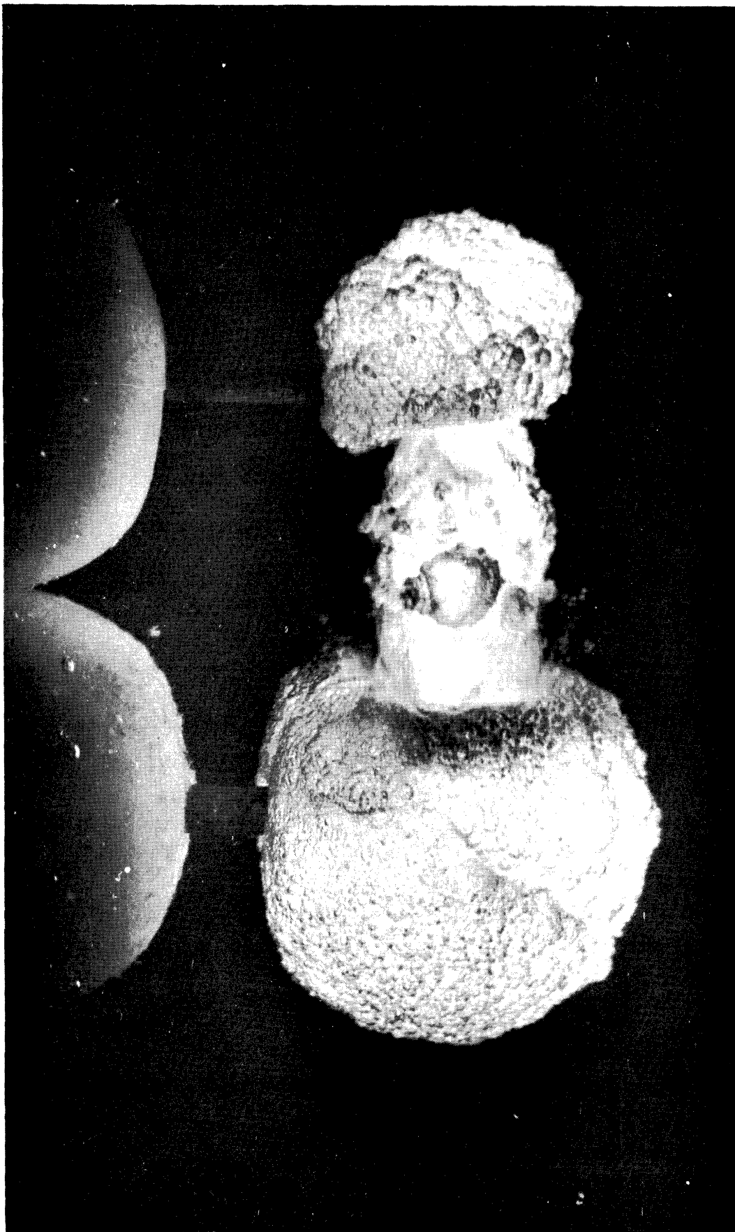
Figure 2. Kerr cell photograph of a 6 kv underwater spark 10 \mu sec after breakdown. Left electrode positive.
