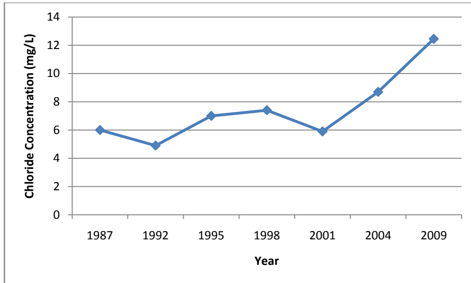
Figure 2: Chloride concentrations in Paradise Lake, Michigan. The levels of chloride ions present in the water column have nearly doubled in the last nine years.
