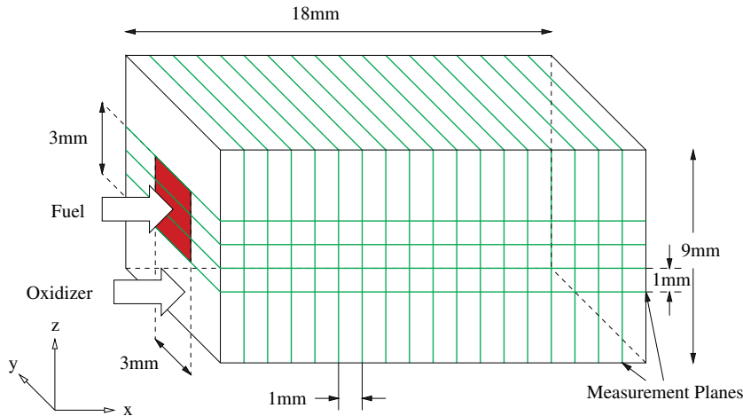
Figure 2. Combustor model domain and problem setup.
