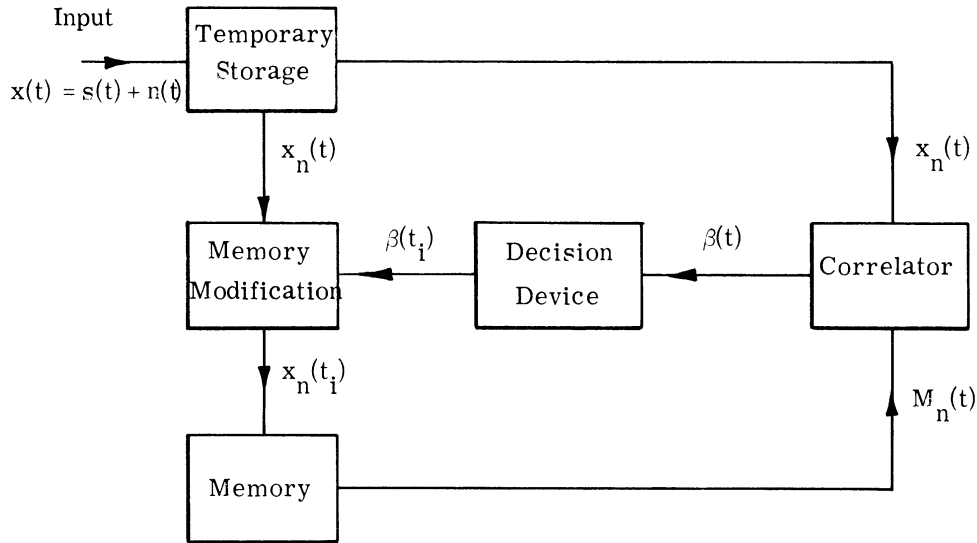
Fig. 1.2. Jakowatz, Shuey and White original adaptive filter.
