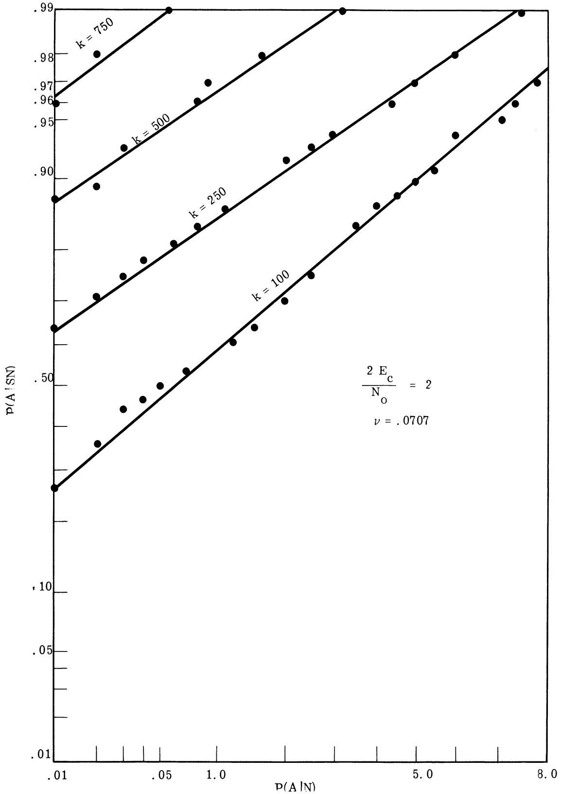
Fig. 7.21. ROC for optimum receiver, CKE, Synchronous-Poisson Time Structure, \frac{2E_c}{N_o} = 2, \nu = .0707.
