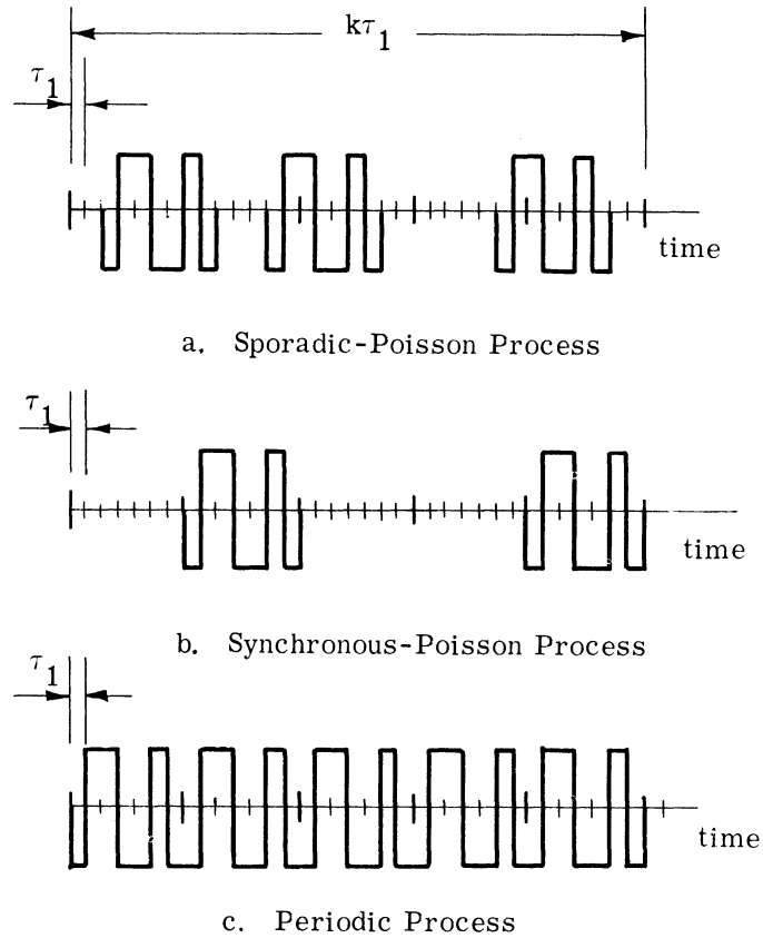
Fig. 4.3. "Typical" signals.
