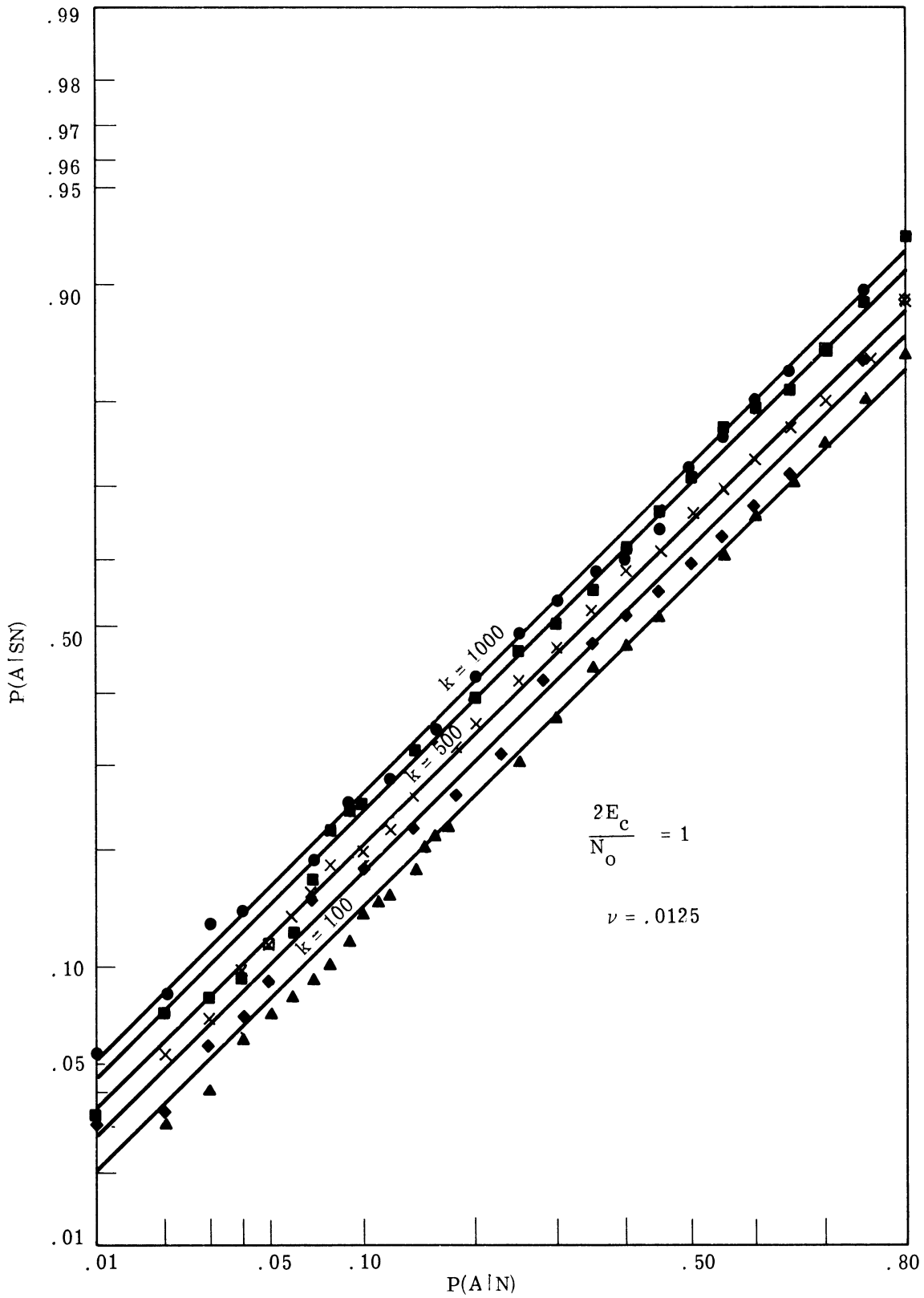
Fig. 7.20. ROC for optimum receiver, CKE, Synchronous-Poisson Time Structure, \frac{2E_c}{N_o} = 1 , \nu = .0125 .
