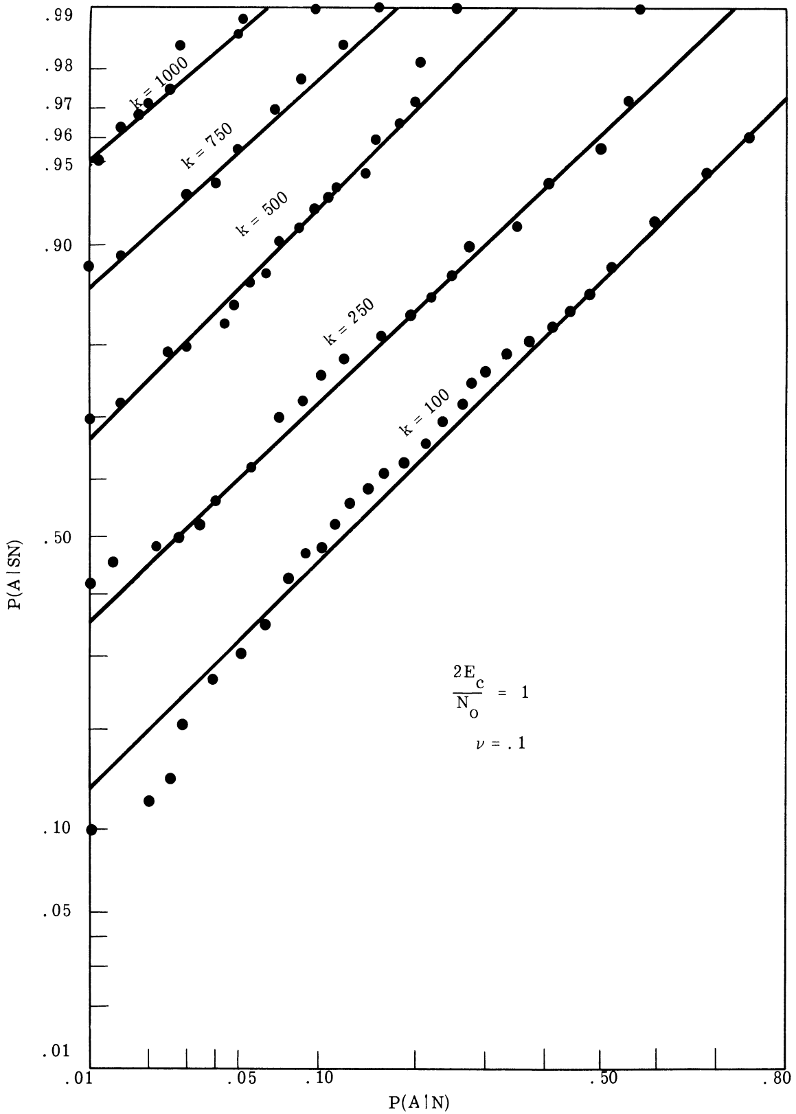
Fig. 7.24. ROC for optimum receiver, CKE, Synchronous-Poisson Time Structure, \frac{2E_c}{N_0} = 1, \nu = .1.
