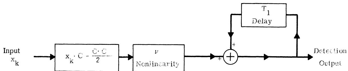
Fig. 5.13 b. Optimum receiver, CKE, Synchronous-Poisson Time Structure
