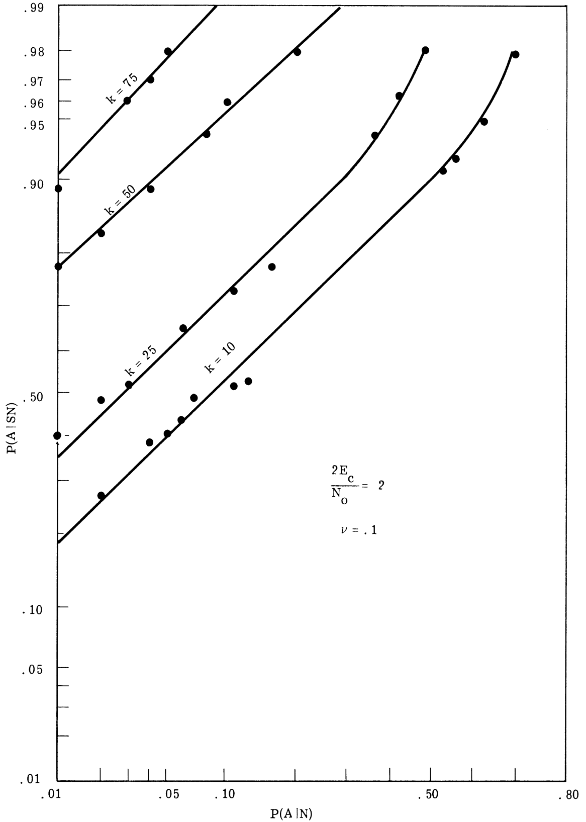
Fig. 7.37. ROC for optimum receiver, CKE, arrival times known exactly,
