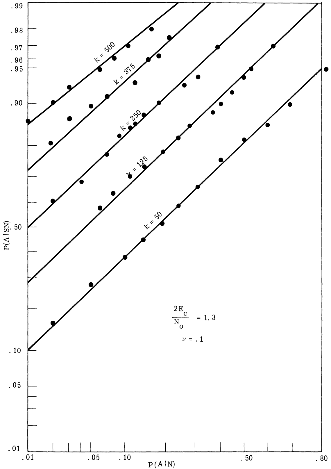
Fig. 7.25. ROC for optimum receiver, CKE, Synchronous-Poisson Time Structure, \frac{2E_c}{N_0} = 1.3, \nu = .1 .
