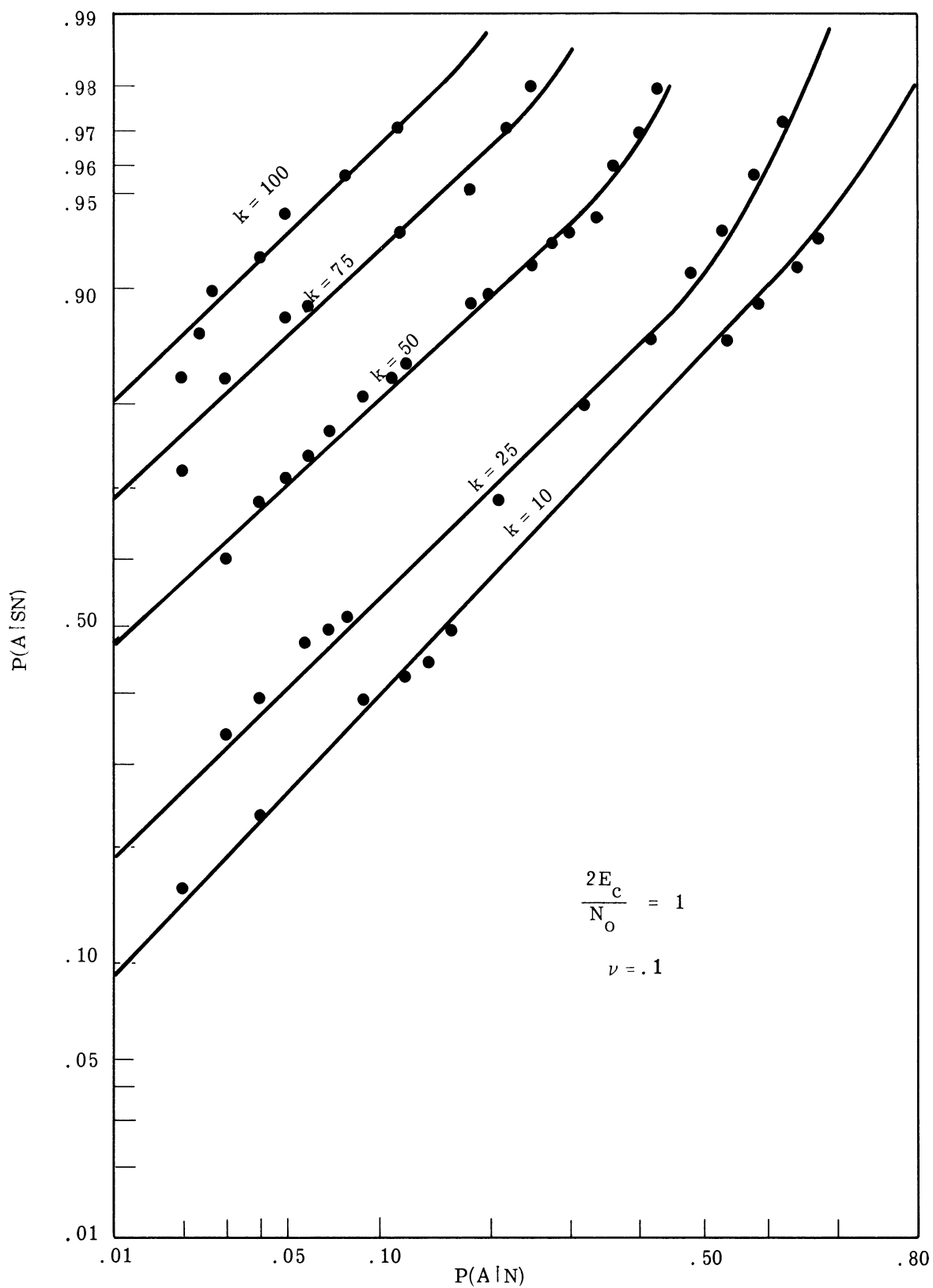
Fig. 7.36 ROC for optimum receiver, CKE, arrival times known exactly,
