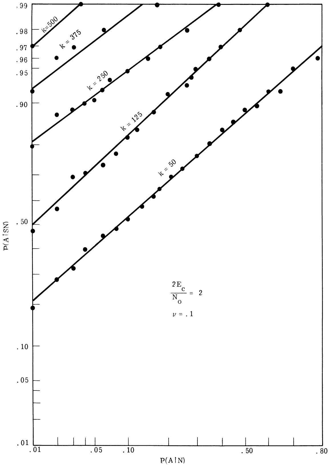
Fig. 7.26. ROC for optimum receiver, CKE, Synchronous-Poisson Time Structure, \frac{2E_c}{N_0} = 2, \nu = .1.
