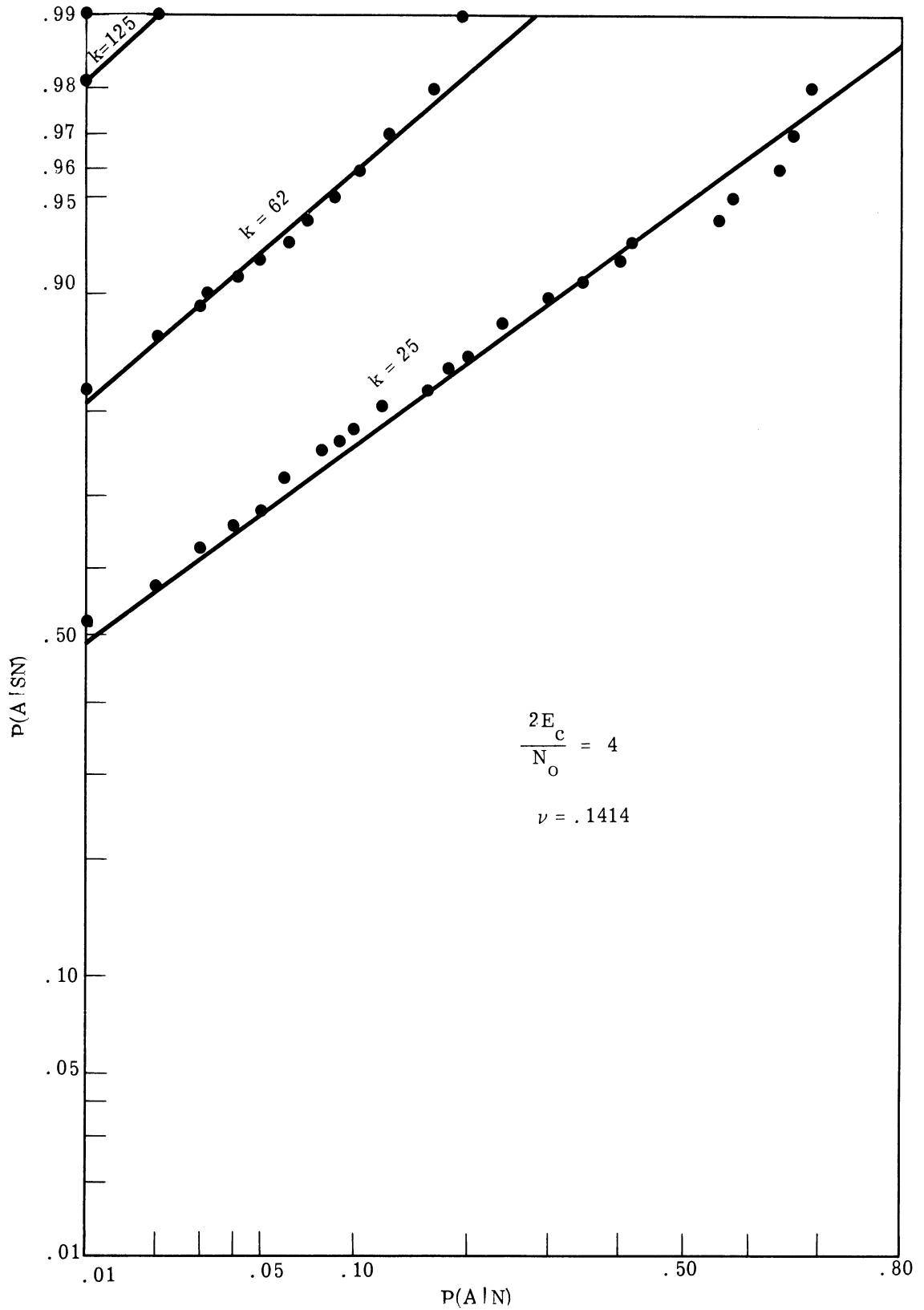
Fig. 7.29. ROC for optimum receiver, CKE, Synchronous-Poisson Time Structure,
