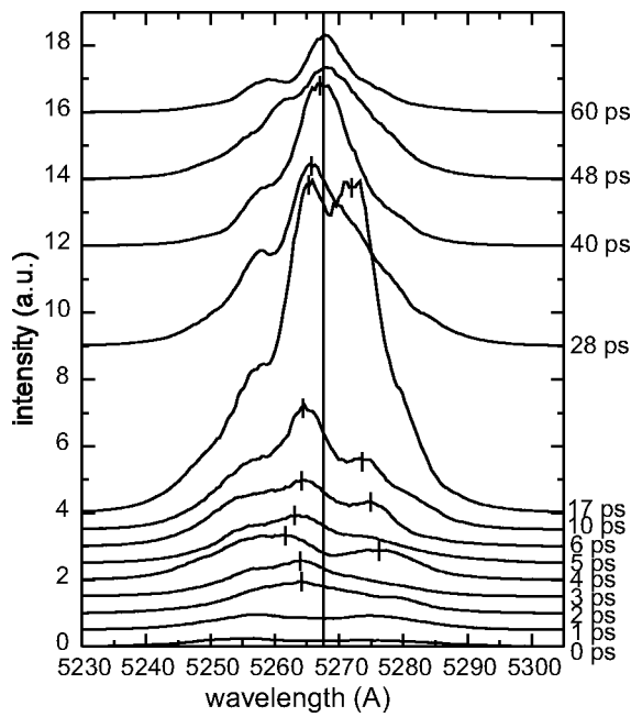
FIG. 13. Spectra of the scattered probe light near the probe wavelength for various probe delays at 25°, 3 TW pump laser power, and 3.7 \times 10^{19} \text{ cm}^{-3} plasma density. The long vertical line indicates the probe wavelength. The short vertical lines indicate the wavelength of the blue- or red-shifted peaks. Note that the intensity scale is linear and that the curves are vertically displaced for ease of viewing. Also note that the bumps on the shoulder originate from the original probe spectrum which is monitored with the 165° channel, (f), which detected the probe light scattered from the nozzle.
