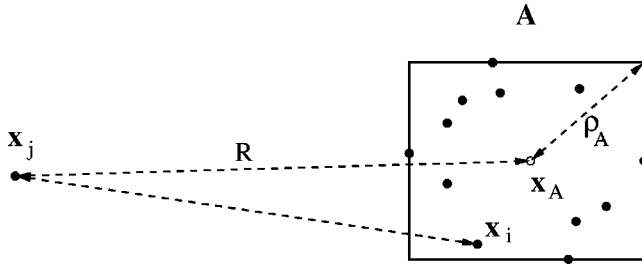
FIG. 1. Particle j and a cluster of particles A .
