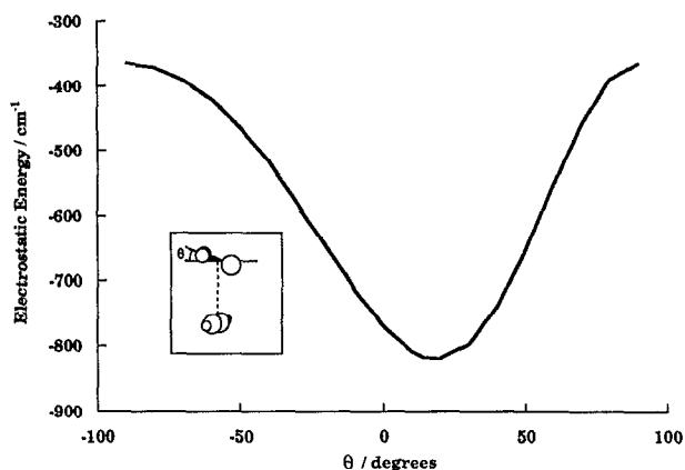
FIG. 3. Electrostatic energy as a function of the tilt angle of SO_2 , for R_{c.m.} fixed at the experimental distance.
