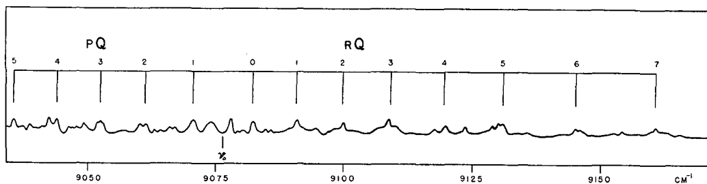
FIG. 3. Microphotometer trace of the perpendicular band of allene at 11,017A, smoothed and corrected for the change in background. Suggested numberings of the Q branches are given. The pQ branch only extends to the fifth line because the band overlaps the 11,100A bands beyond that point.
