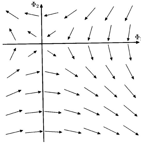
FIG. 2. Flow of \Phi^\pm for large r , schematic.
