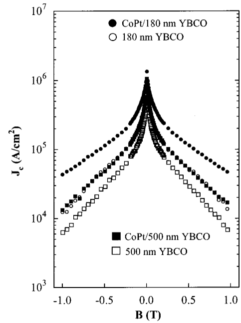
FIG. 2. J_c vs B\|c transport measurements for 500 and 180 \text{ nm} YBCO films at 86 \text{ K} with and without CoPt multilayer applied.
