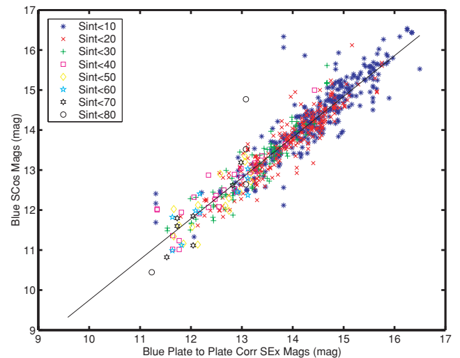
Figure 3. The calibrated B_j magnitudes of the SuperCOS data versus the SEXTRACTOR uncalibrated B_j magnitudes. By fitting and using the values from the line of best fit, a calibration value for bright objects is determined and the calibrated magnitude is calculated for each optically matched galaxy. The corresponding HICAT integrated flux strengths ( \text{Jy km s}^{-1} ) are listed in the inserted panel.
