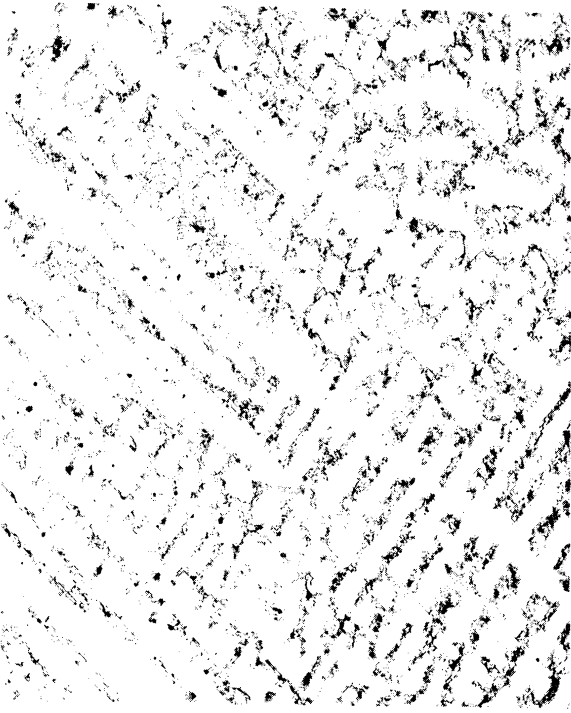
(a) Rupture tested at 1500°F, 30,000 psi (30 hr)
