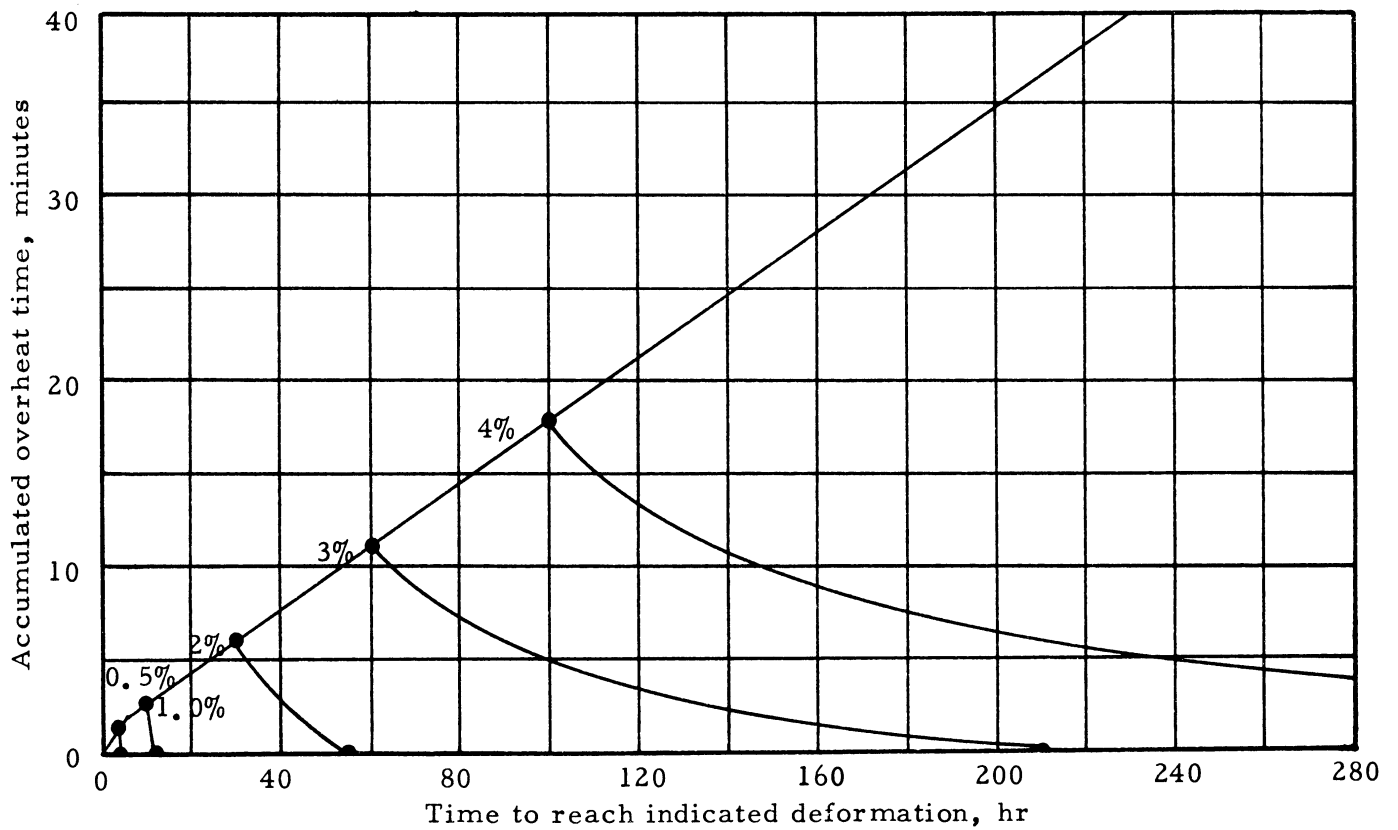
(b) Overheats to 1800°F.
