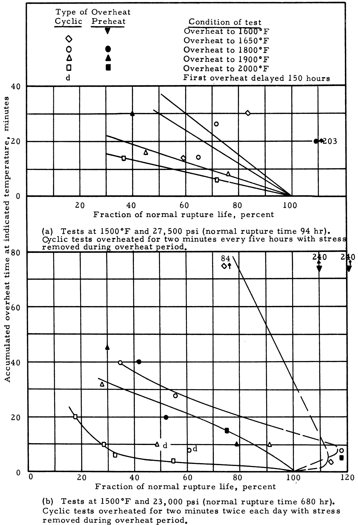
Figure 11.- Effect of amount of overheating to 1600°, 1650°, 1800°, 1900°, and 2000°F on the rupture life at 1500°F under a stress of 23,000 or 27,500 psi.
