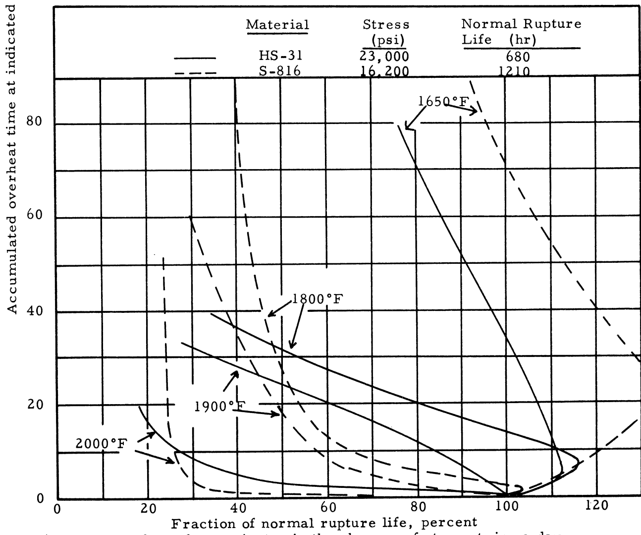
Figure 37. - Comparison for HS-31 and S-816 alloy of the effect of amount of overheating to 1650°, 1800°, 1900° and 2000°F on the rupture life at 1500°F under the indicated stress.
