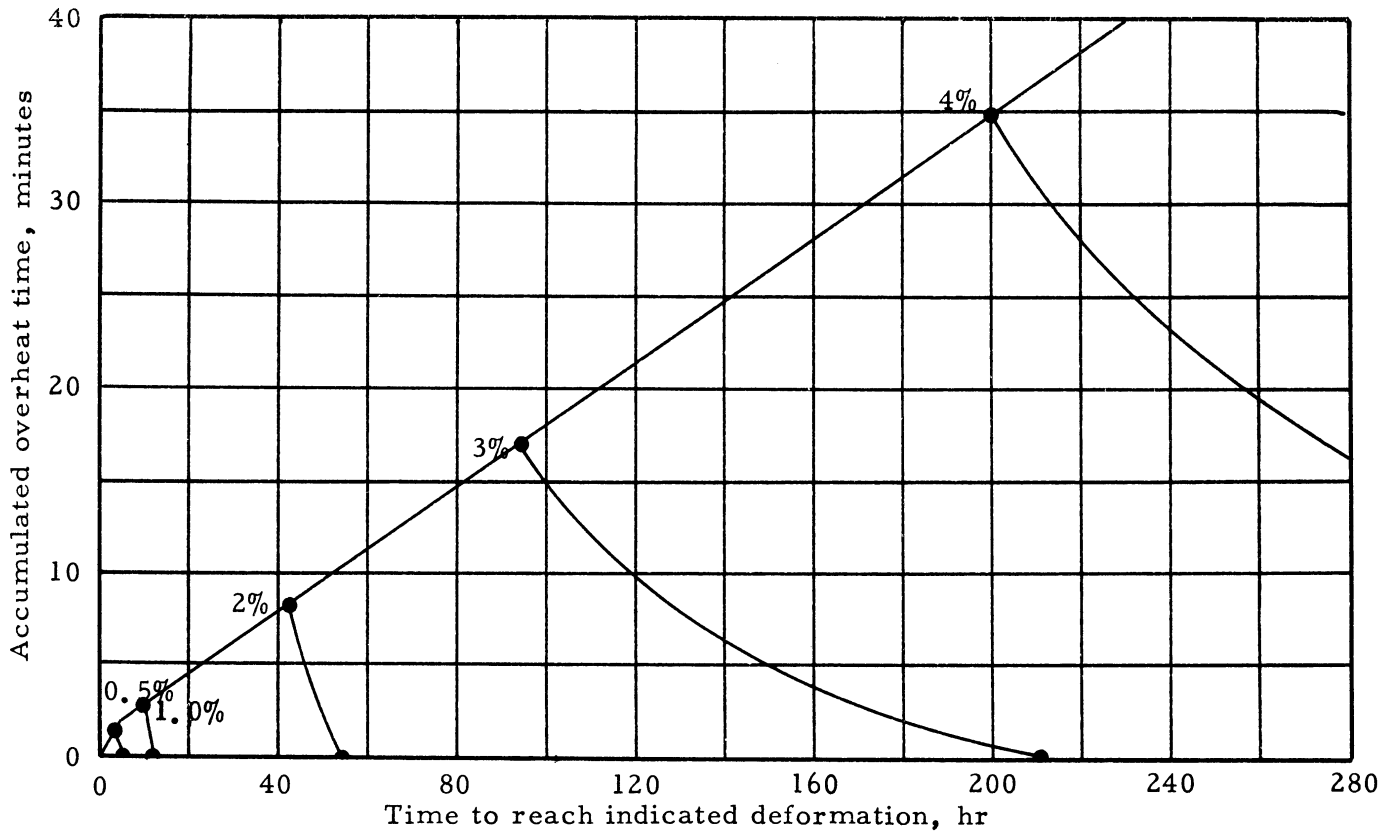
(a) Overheats to 1650°F.
