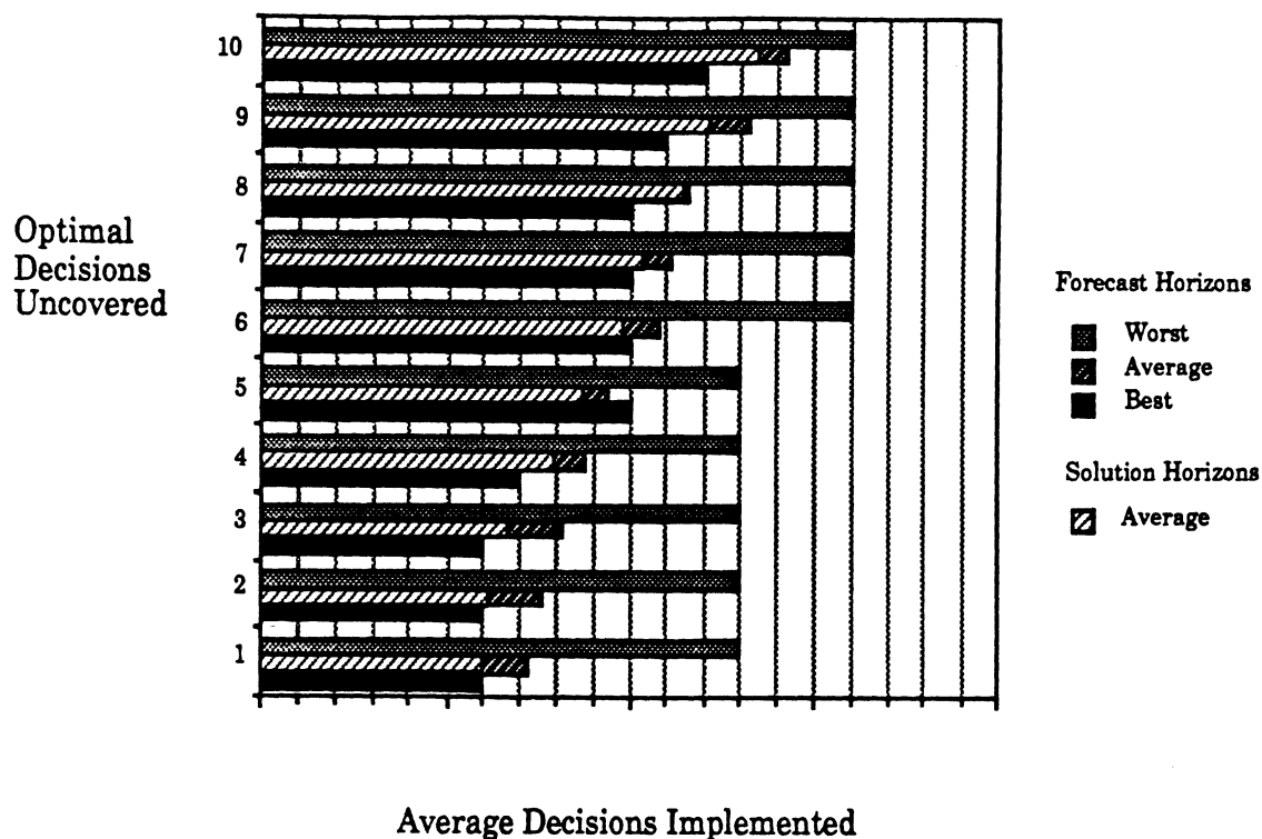
Figure 2: Forecast horizons for the cyclic demand function.
