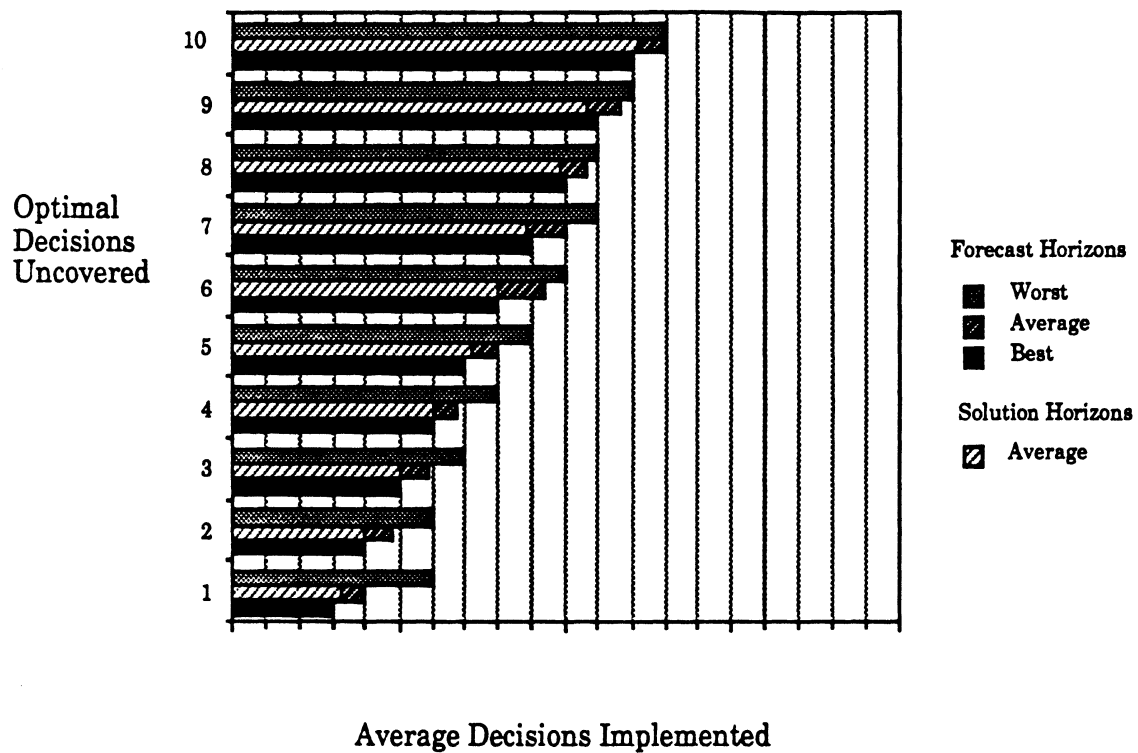
Figure 1: Forecast horizons for the linear demand function, measured by the average number of decisions implemented by efficient strategies. The best, average, and worst case forecast horizons are shown as well as solution horizons for the average case.
