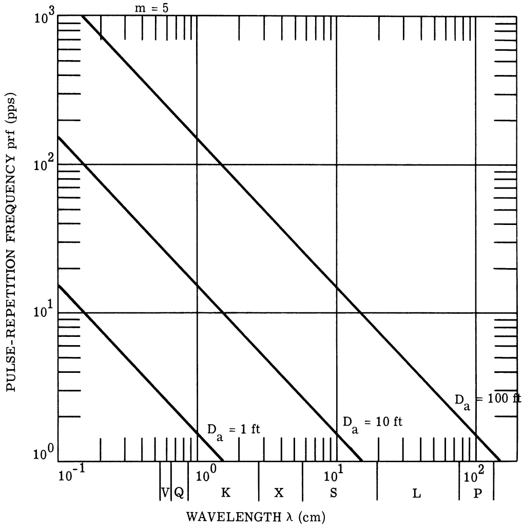
FIGURE 51. NONCOHERENT-RADAR PULSE-RATE REQUIREMENTS
