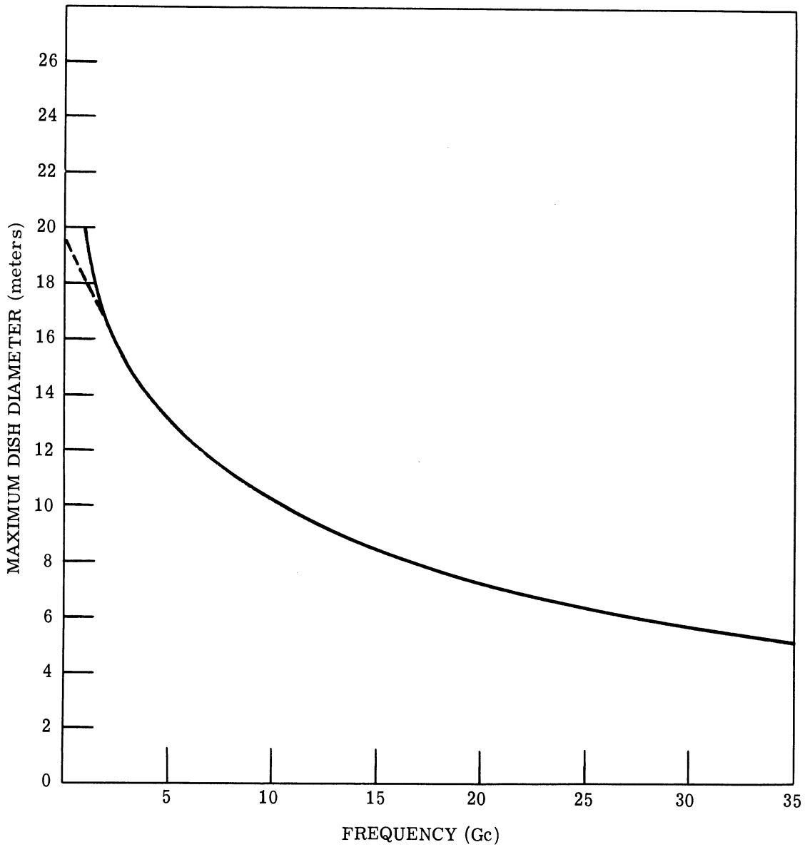
FIGURE 40. ATTAINABLE DISH DIAMETER vs. FREQUENCY. The maximum dish diameter attainable in space with deployable antennas in the 1970 time frame were explored by Hiatt and Larson with these results (Ref. 15).
