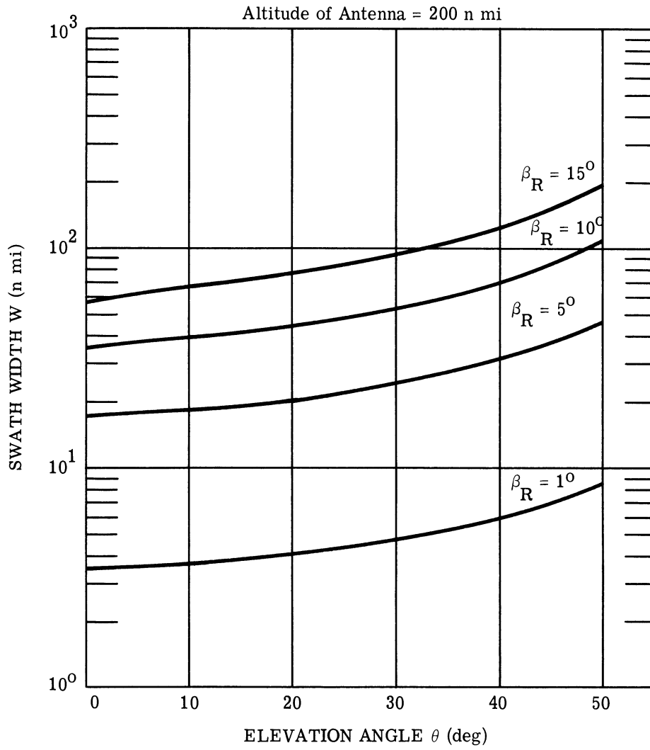
FIGURE 48. ILLUMINATED SWATH WIDTH
