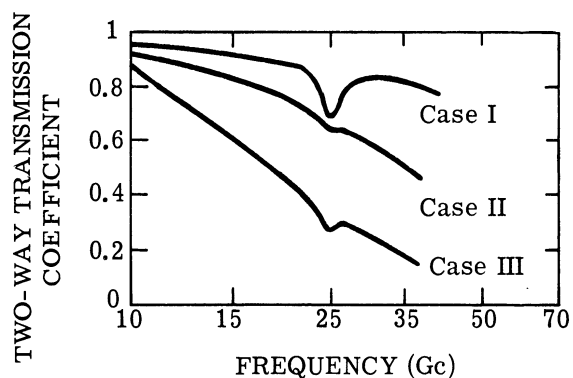
FIGURE 20. TWO-WAY ATMOSPHERIC TRANSMISSION COEFFICIENT vs. OPERATING FREQUENCY FOR A 12-mi ALTITUDE (Ref. 36). Case I: maritime tropical atmosphere containing water vapor but no clouds. Case II: heavy snow falling from a dense mixed water-ice cloud to an altitude of 5 mi. Case III: heavy snow turning to rain falling through a dense water cloud. Heavy weather extends to an altitude of 4 mi.
