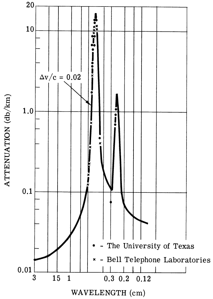
FIGURE 39. ATTENUATION OF OXYGEN vs. WAVELENGTH (Reprint from Ref. 13, p. 135)
