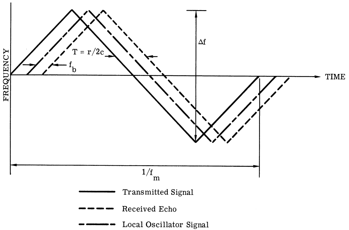
FIGURE 63. FREQUENCY TIME RELATIONSHIP IN FM-CW RADAR
