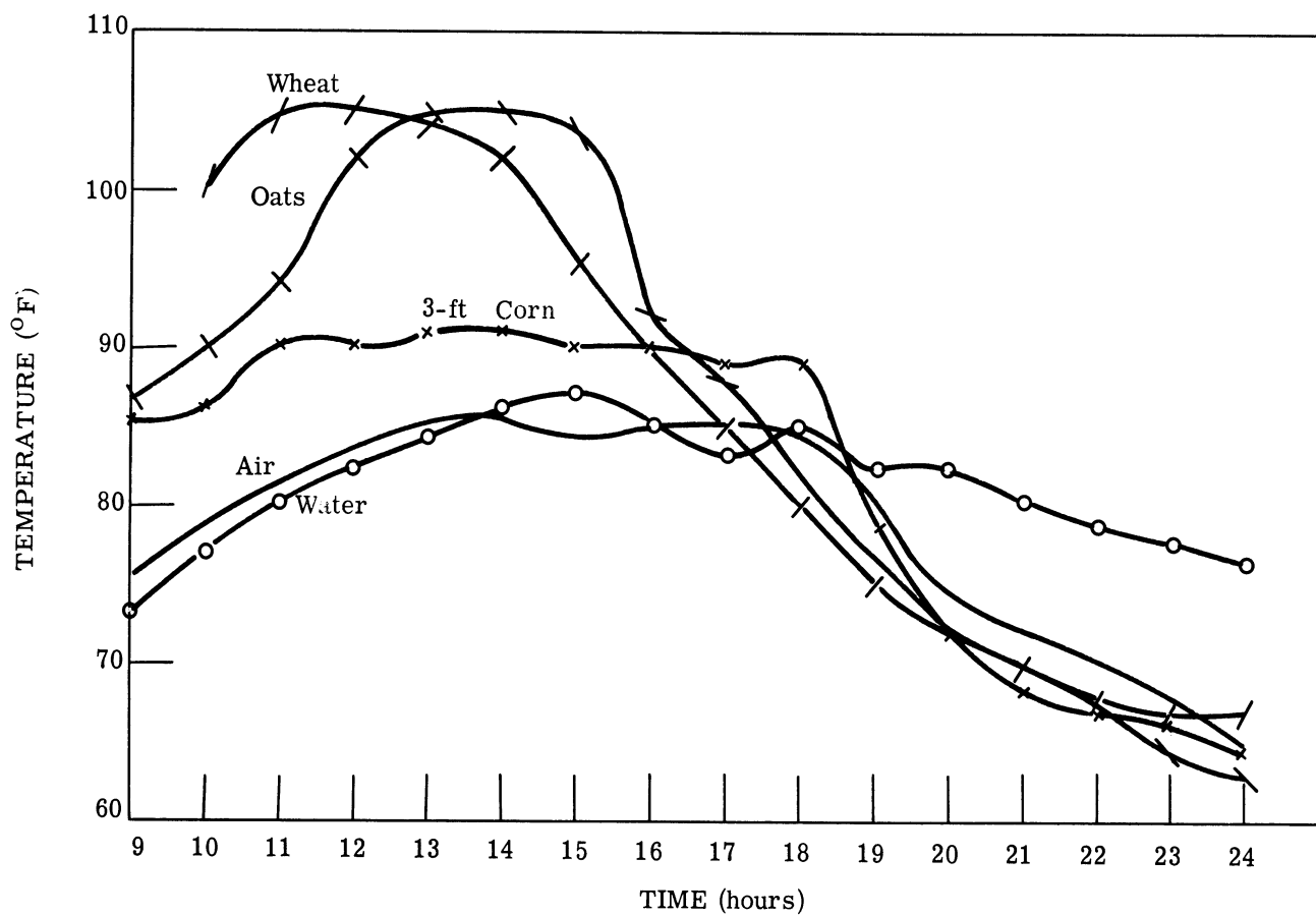
FIGURE 28. TEMPERATURE VARIATIONS OF CROPS
