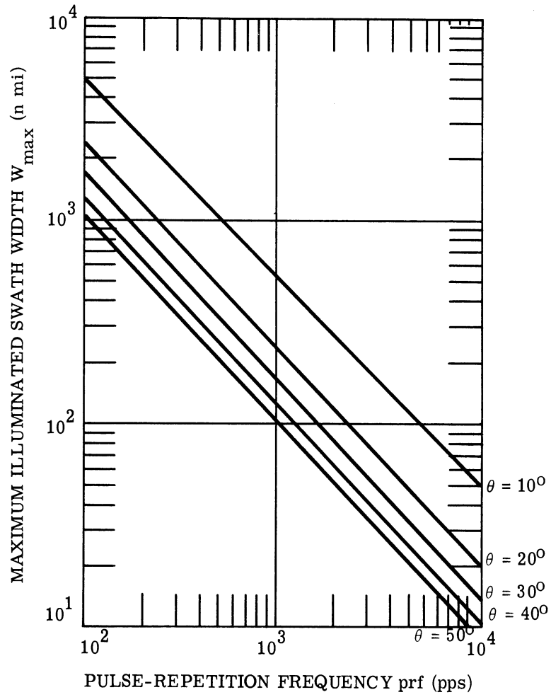
FIGURE 56. MAXIMUM SWATH WIDTH
