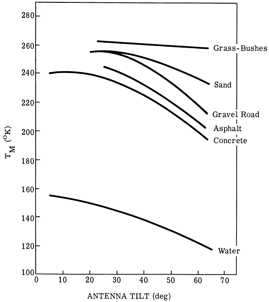
FIGURE 2. MEASURED TARGET TEMPERATURE vs. ANTENNA TILT (Ref. 12)
