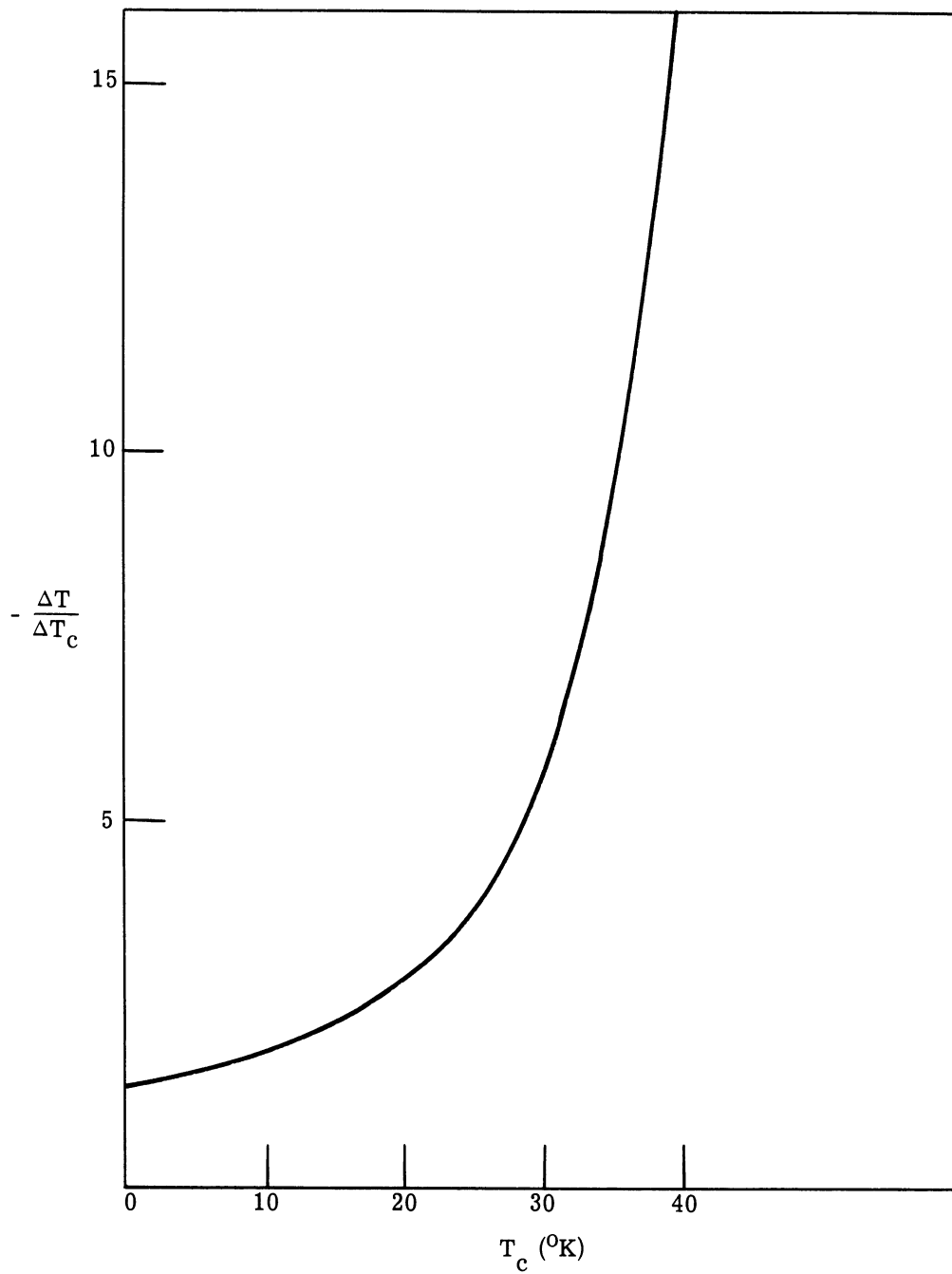
FIGURE 32. SIGNAL-LEVEL STABILITY AS A FUNCTION OF CELL TEMPERATURE
