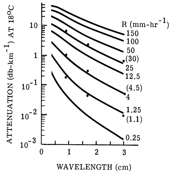
FIGURE 4. ATTENUATION vs. WAVELENGTH FOR RAINFALL AT VARIOUS RATES (Ref. 13, p. 134)
