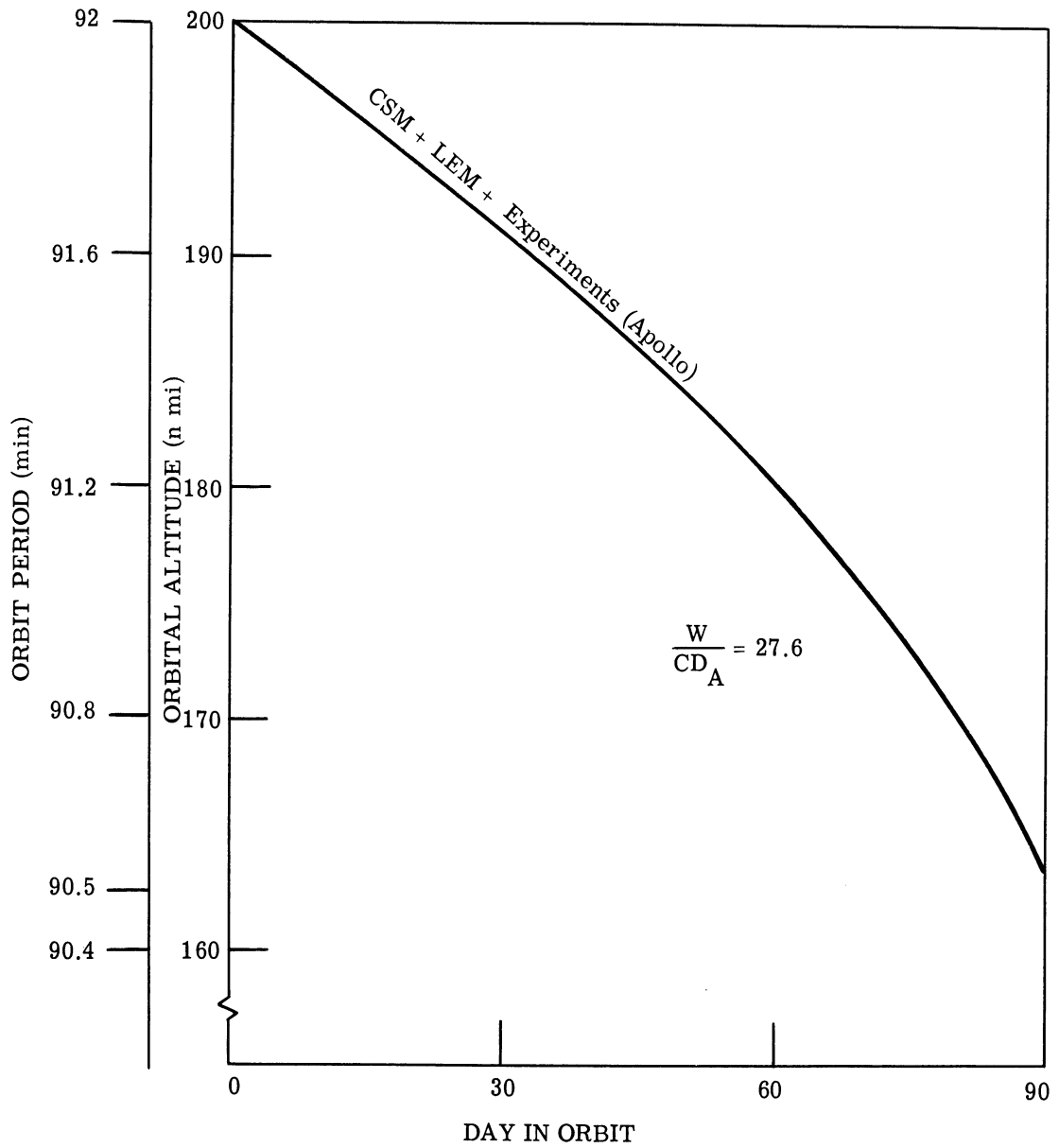
FIGURE 33. APPROXIMATE ORBIT DECAY
