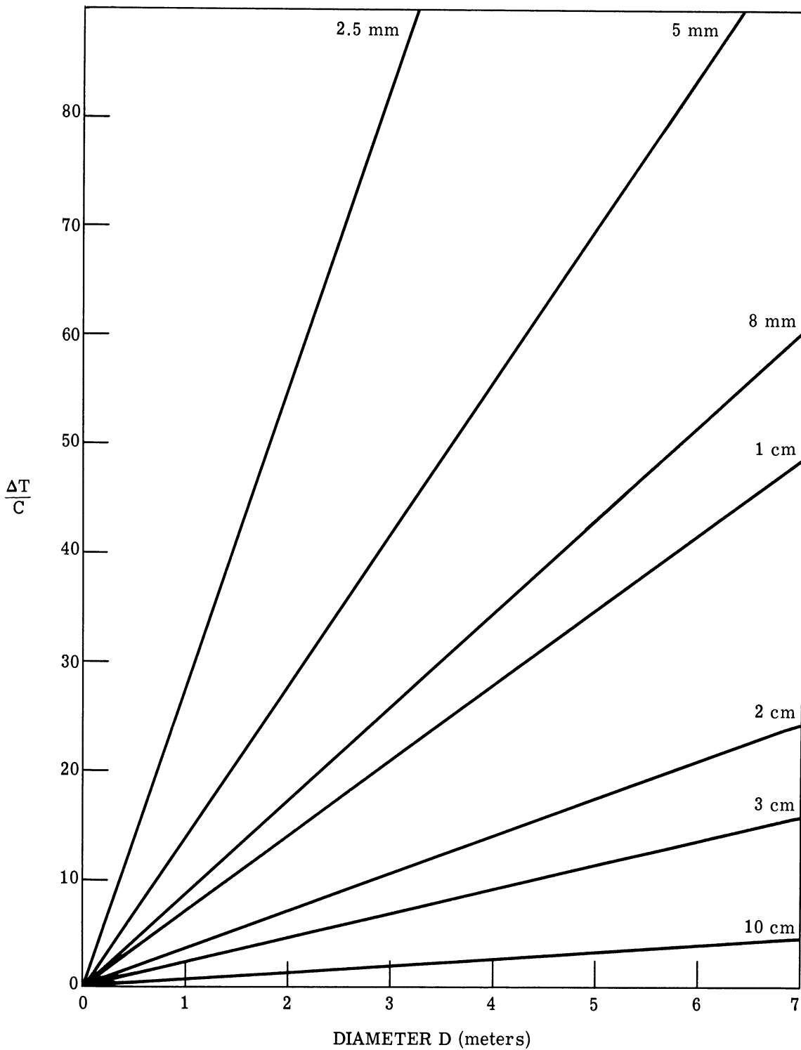
FIGURE 35. \frac{\Delta T}{C} vs. APERTURE DIAMETER. This represents the operation which can be expected for a system at an altitude of 200 n miles, v/h = 0.02 , and a scan angle \alpha = 10^\circ .
