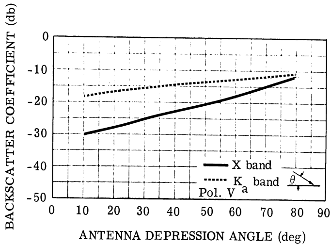
FIGURE 9. ONE-HALF-INCH GREEN WHEAT (Reproduced from Ref. 18)
