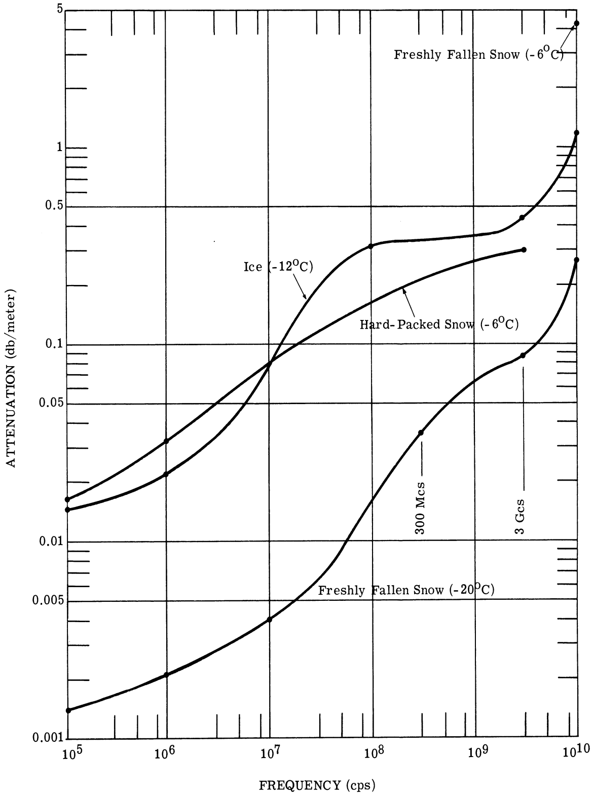
FIGURE 15. ATTENUATION OF ELECTROMAGNETIC WAVES BY ICE AND SNOW vs. FREQUENCY
