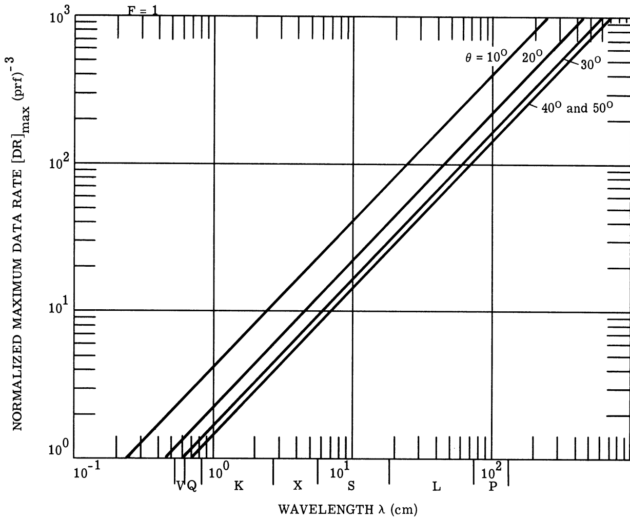
FIGURE 59. MAXIMUM NORMALIZED DATA RATES
