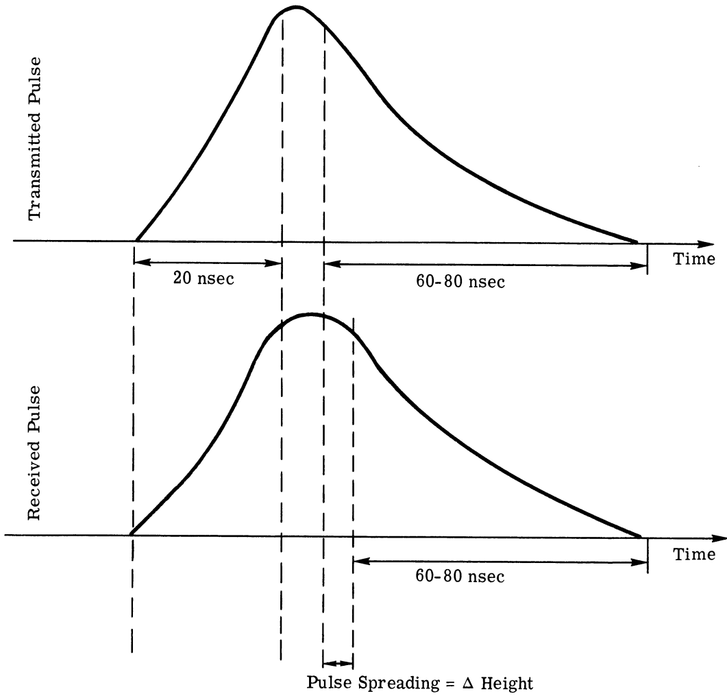
FIGURE 66. TRANSMITTED AND RECEIVED PULSES TO DETERMINE RELATIVE HEIGHT (HEIGHT OF OCEAN WAVES)
