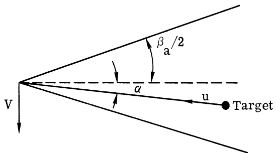
FIGURE 54. TARGET DOPPLER GEOMETRY
