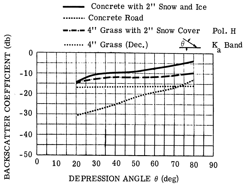
FIGURE 11. EFFECTS OF SNOW COVER UPON \gamma AT K a -BAND, HORIZONTAL POLARIZATION (Reproduced from Ref. 18)
