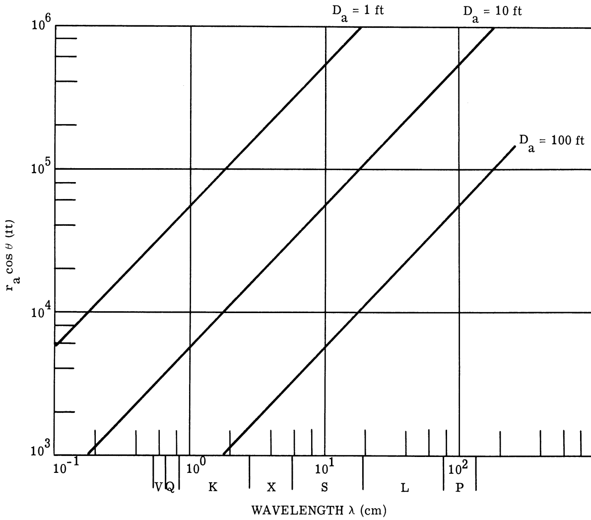
FIGURE 44. AZIMUTH RESOLUTION FOR SATELLITE ORBITING AT 200-n mi ALTITUDE
