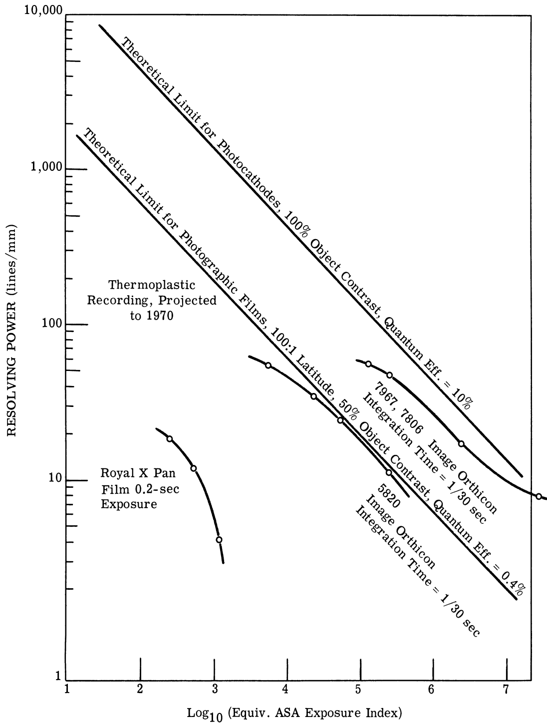
FIGURE 30. THEORETICAL PERFORMANCE FOR PHOTOGRAPHIC FILMS AND PHOTOCATHODES
