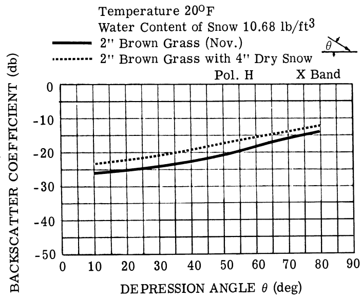
FIGURE 13. EFFECTS OF SNOW UPON \gamma AT X-BAND (Reproduced from Ref. 18)
