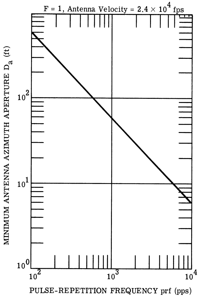
FIGURE 55. MINIMUM ANTENNA APERTURE
