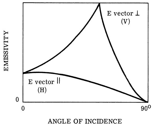
FIGURE 18. EMISSIVITY OF WATER vs. ANGLE OF INCIDENCE AND POLARIZATION (Ref. 29)
