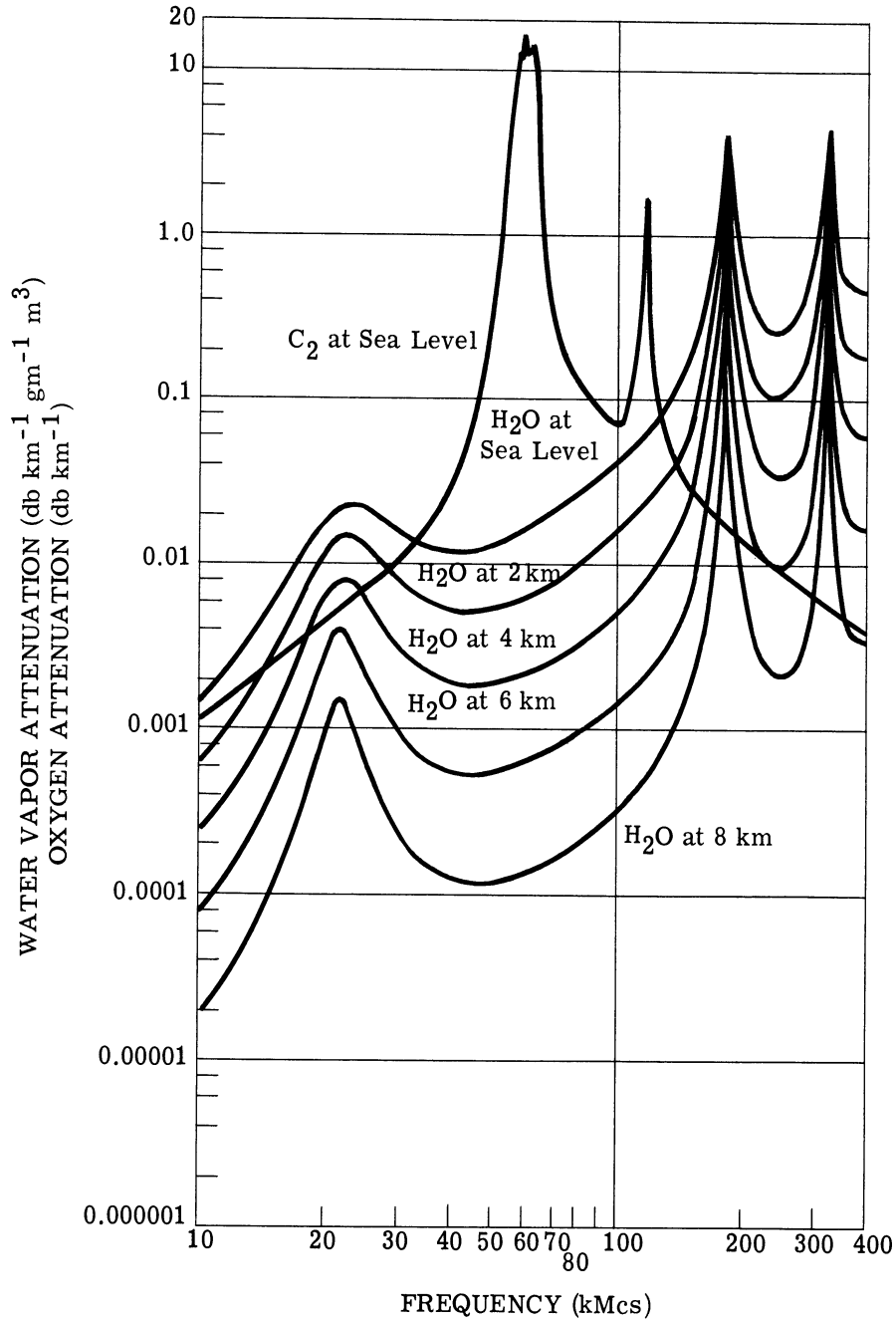
FIGURE 38. OXYGEN AND WATER VAPOR ATTENUATION FOR VARIOUS ELEVATIONS IN THE EARTH'S ATMOSPHERE
