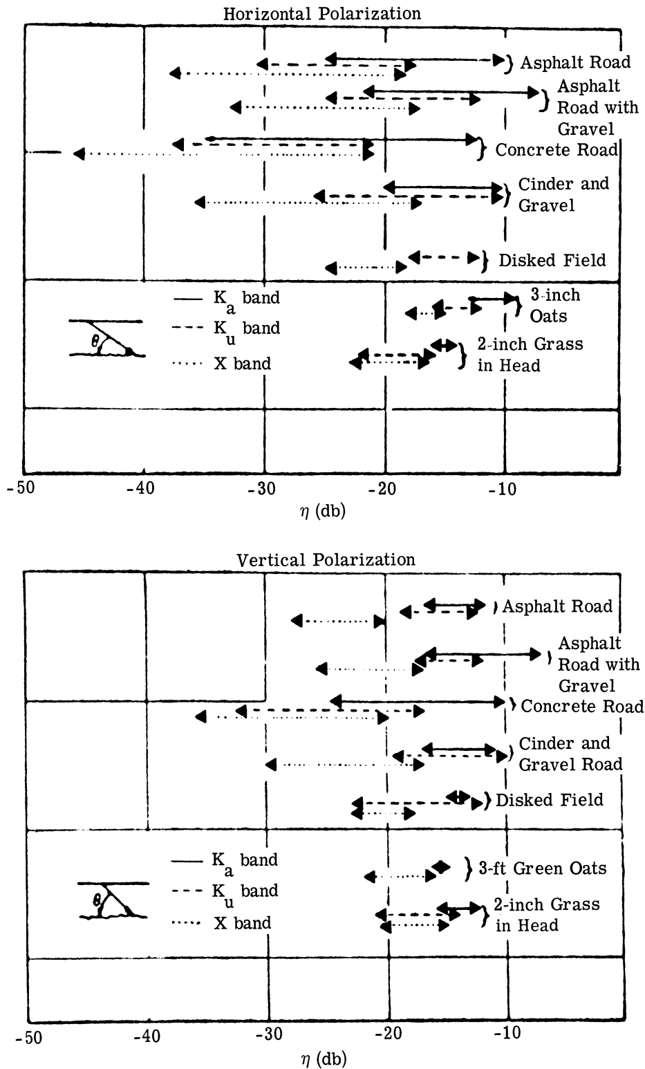
FIGURE 29. DYNAMIC RANGE OF \eta FOR VARIOUS TYPES OF TERRAIN (Reproduced from Ref. 18)
