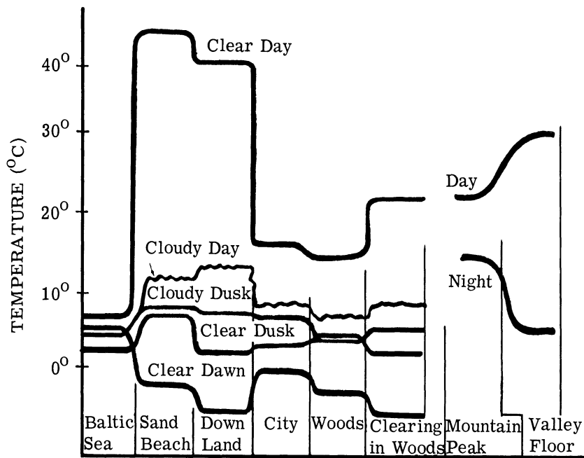
FIGURE 3. TYPICAL GROSS TEMPERATURE DIFFERENCES (Ref. 12)
