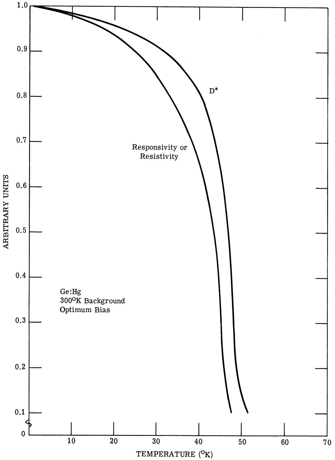
FIGURE 1. DETECTOR PERFORMANCE vs. CELL TEMPERATURE
