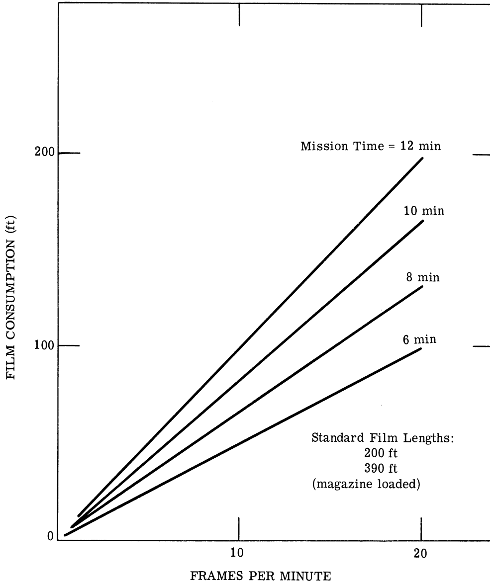
FIGURE 23. FILM CONSUMPTION PER ORBIT vs. FRAMES PER MINUTE AND MISSION TIME. 9- by 9-inch camera.
