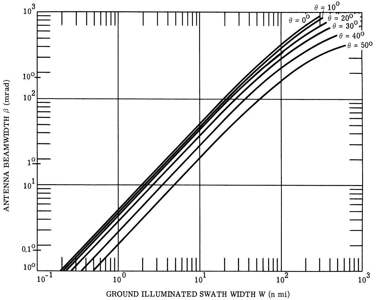
FIGURE 53. GROUND ILLUMINATED SWATH vs. ANTENNA BEAMWIDTH
