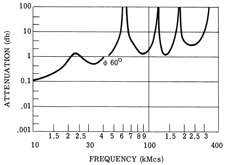
FIGURE 37. TOTAL ATMOSPHERIC ABSORPTION (Extracted from Ref. 12)
