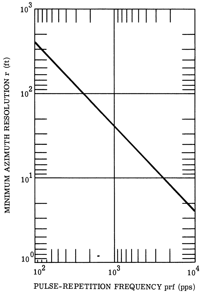
FIGURE 57. AZIMUTH RESOLUTION BASED ON SYSTEM CONSTRAINTS
