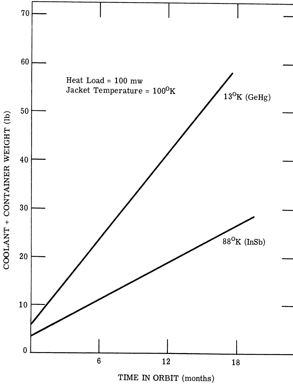
FIGURE 21. COOLANT + CONTAINER WEIGHT vs. TIME IN ORBIT. Reproduced from Ref. 38.
