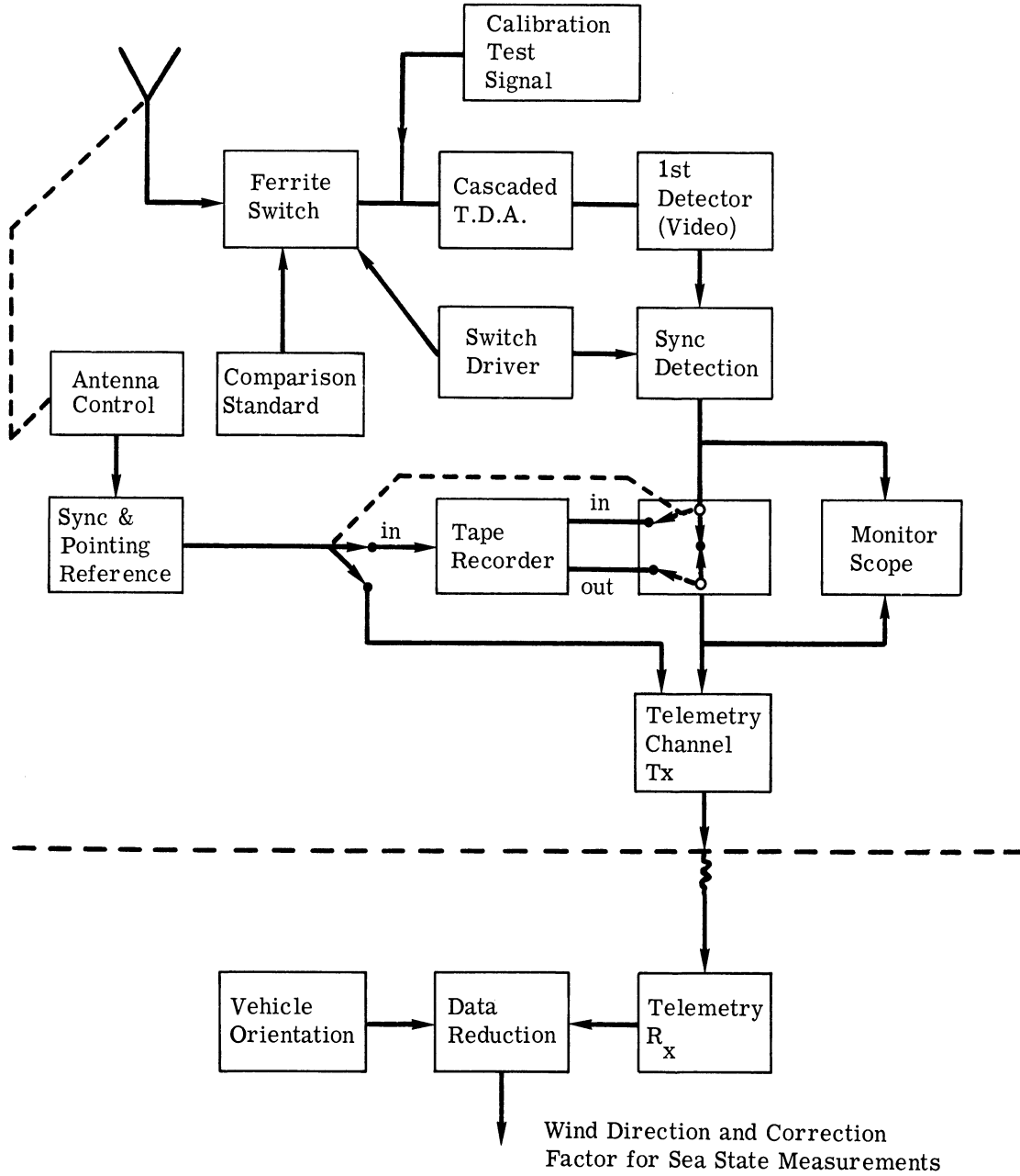
FIGURE 6. CONICAL-SCANNING RADIOMETER (X-BAND) BLOCK DIAGRAM
