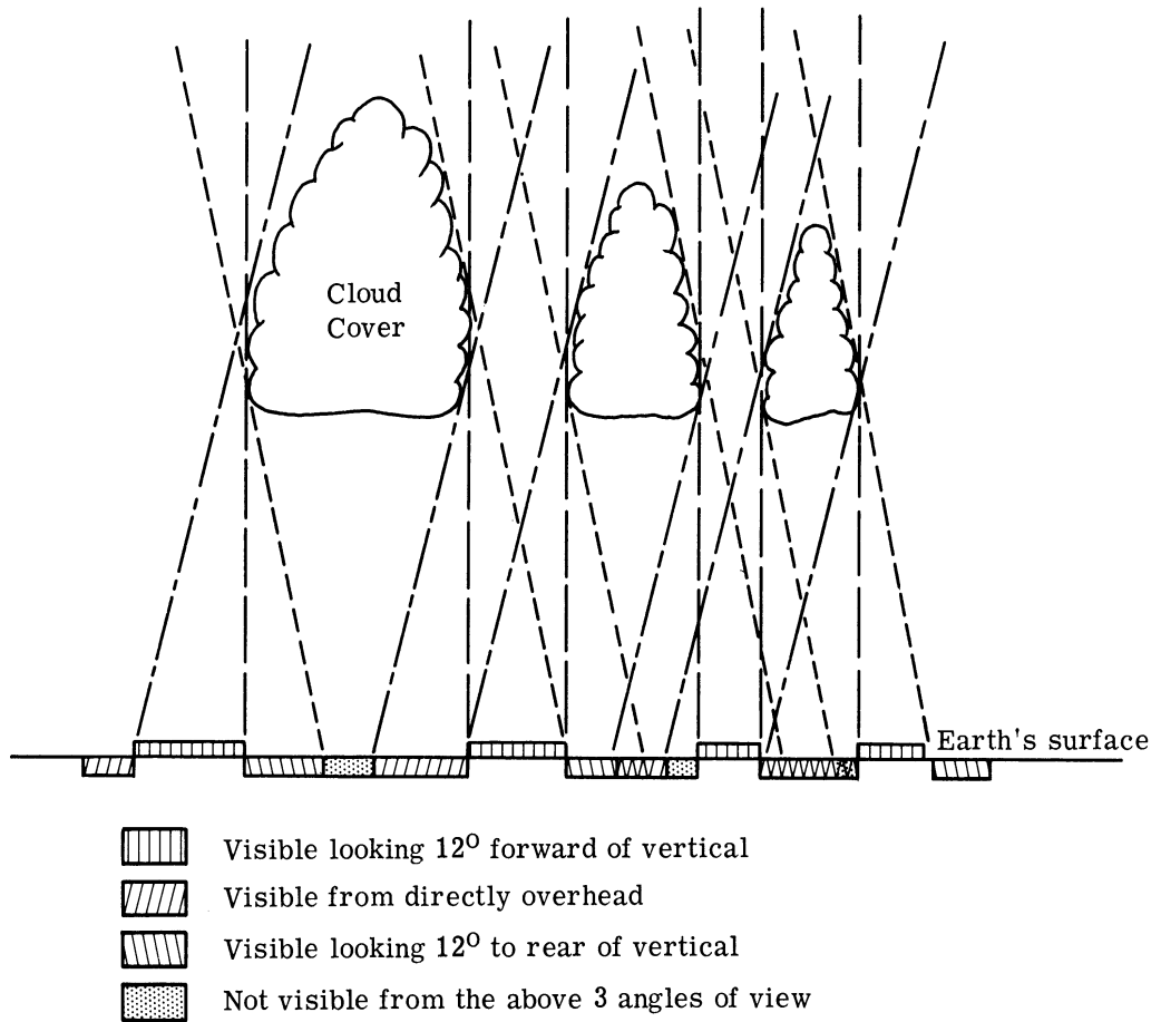
FIGURE 24. EFFECT OF CLOUD COVER ON TERRAIN VISIBILITY
