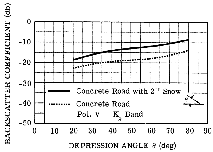
FIGURE 12. EFFECTS OF SNOW COVER UPON \gamma AT K_a -BAND, VERTICAL POLARIZATION (Reproduced from Ref. 18)
