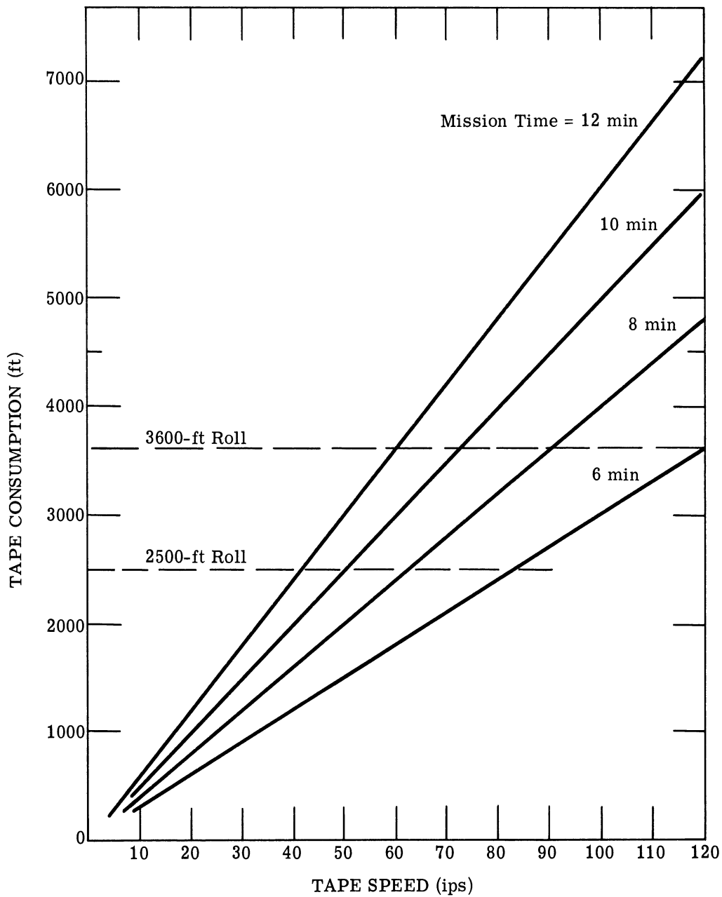
FIGURE 22. TAPE CONSUMPTION PER ORBIT vs. TAPE SPEED AND MISSION TIME
