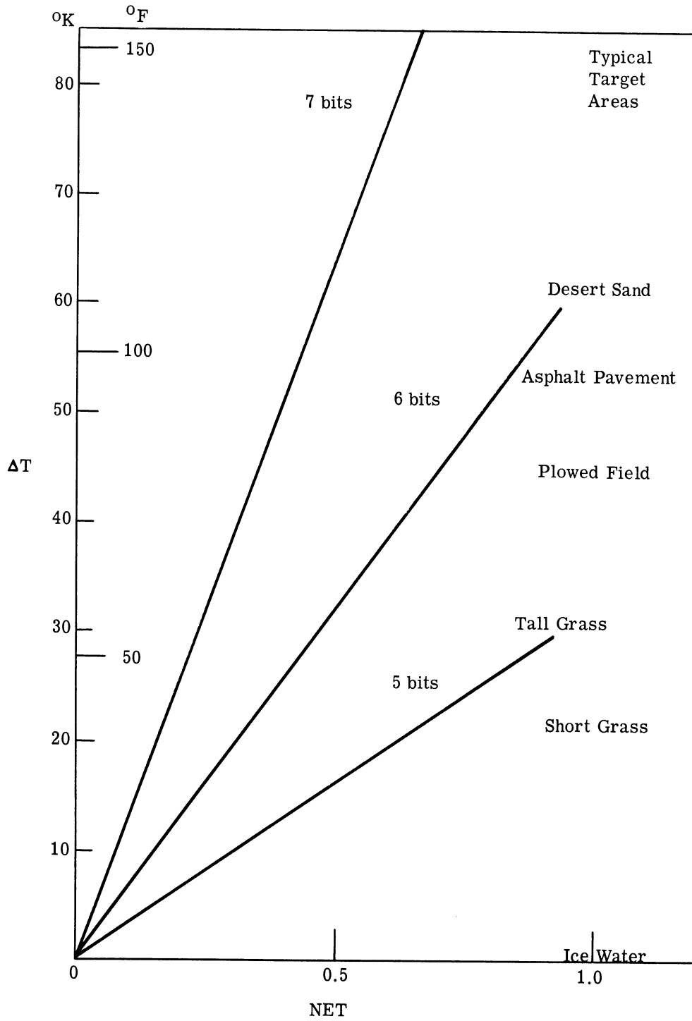
FIGURE 26. RELATIONSHIP BETWEEN NET, BITS/ELEMENT, AND TEMPERATURE
