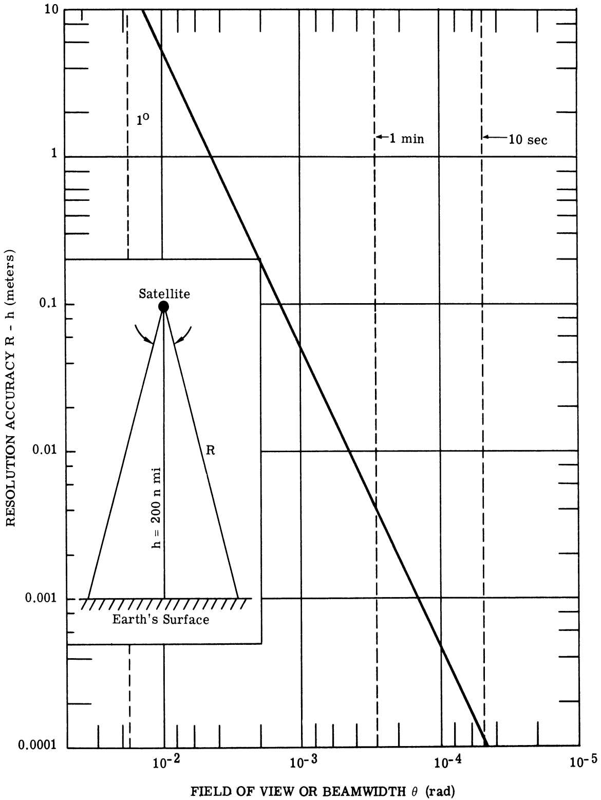
FIGURE 64. GEOMETRICAL RESOLUTION ACCURACY vs. FIELD OF VIEW FROM A 200-n mi SATELLITE
