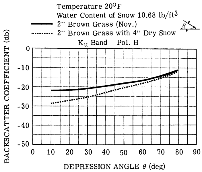
FIGURE 14. EFFECTS OF SNOW UPON \gamma AT K u -BAND (Reproduced from Ref. 18)
