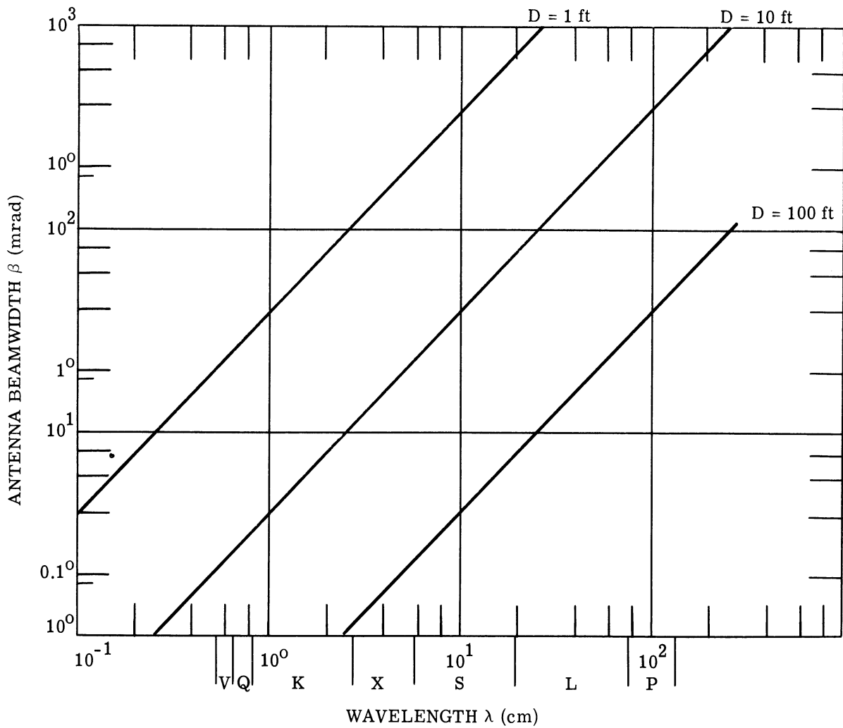
FIGURE 46. ANTENNA BEAMWIDTH
