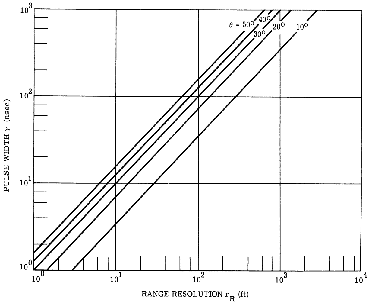
FIGURE 45. PULSE WIDTH DEPENDENCE FOR RANGE RESOLUTION
