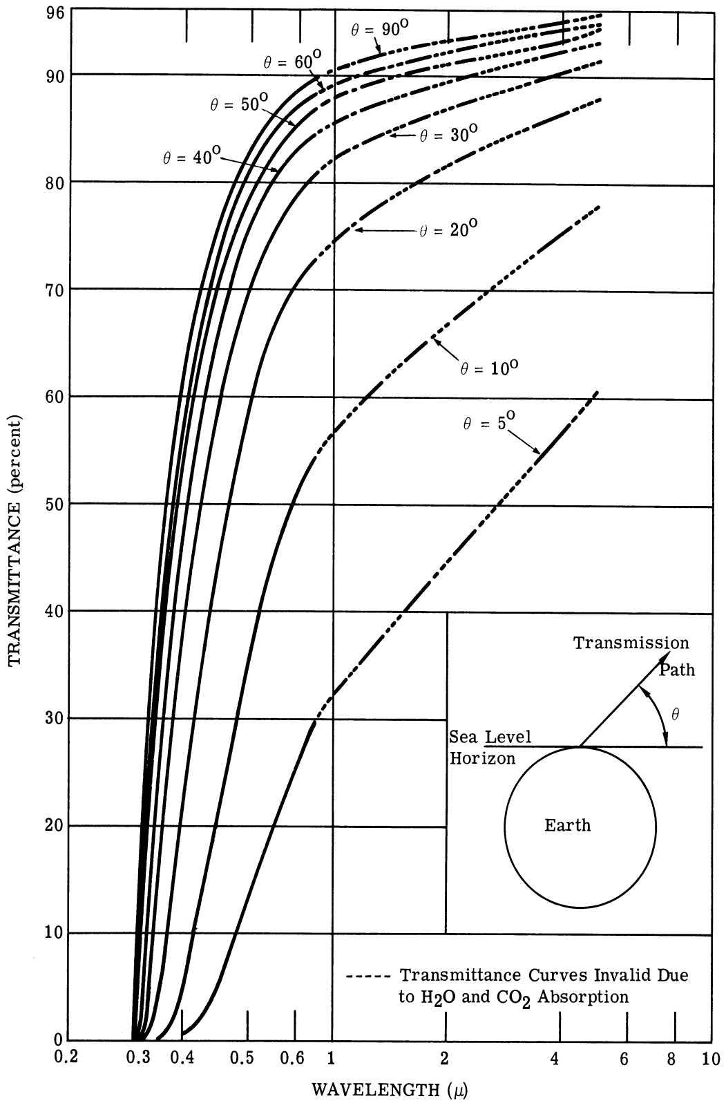
FIGURE 61. TRANSMITTANCE OF THE TOTAL ARDC STANDARD ATMOSPHERE FOR RAYLEIGH AND MIE SCATTERING, AND OZONE ABSORPTION vs. WAVELENGTH AND ELEVATION ANGLE
