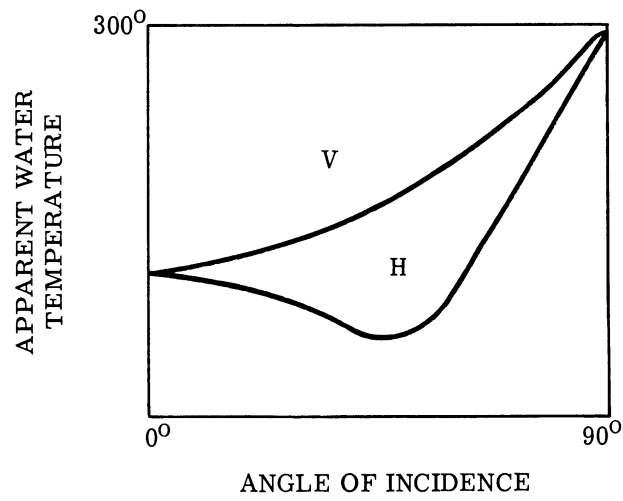
FIGURE 19. APPARENT WATER TEMPERATURE vs. ANGLE OF INCIDENCE AND POLARIZATION (Ref. 29)
