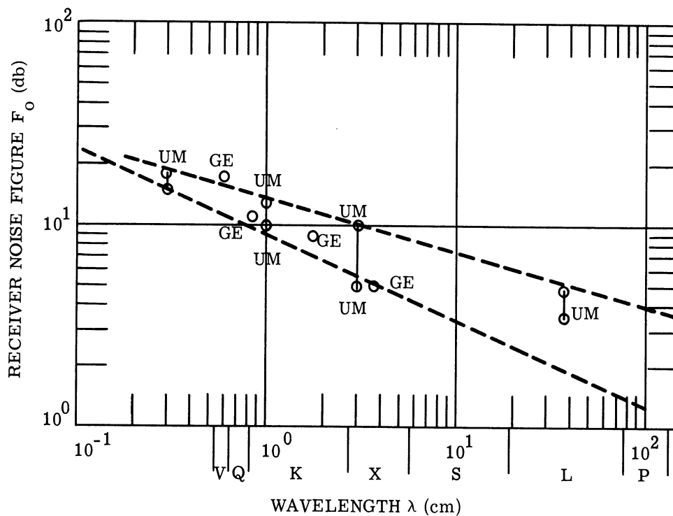
FIGURE 49. ATTAINABLE SYSTEM NOISE FIGURES
