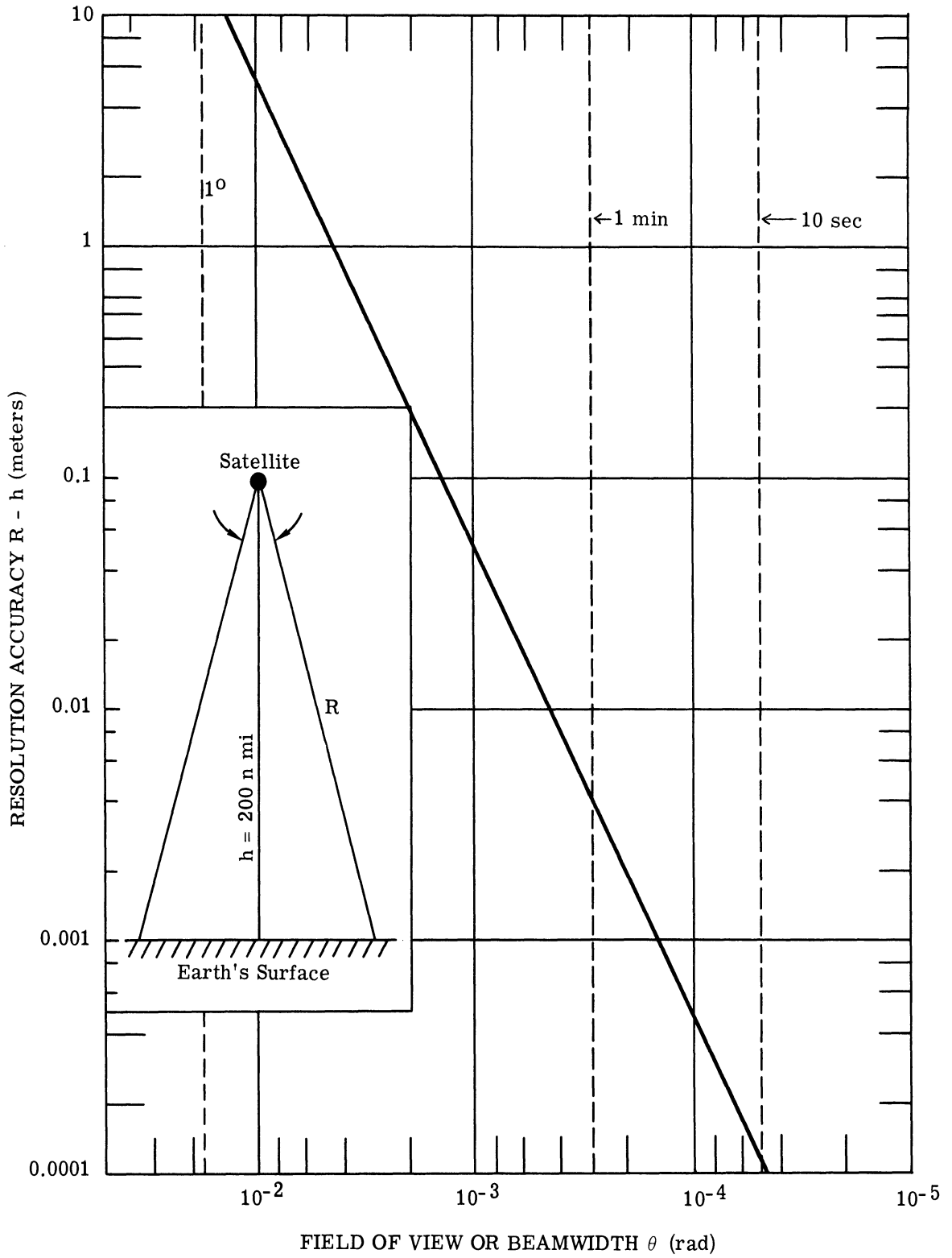
FIGURE 16. GEOMETRICAL RESOLUTION ACCURACY vs. FIELD OF VIEW FROM A 200-n mi SATELLITE
