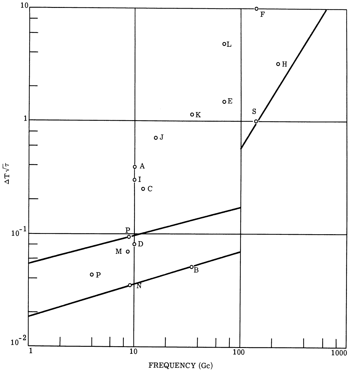
FIGURE 36. RECEIVER FIGURE OF MERIT vs. FREQUENCY (for state-of-the-art devices)
