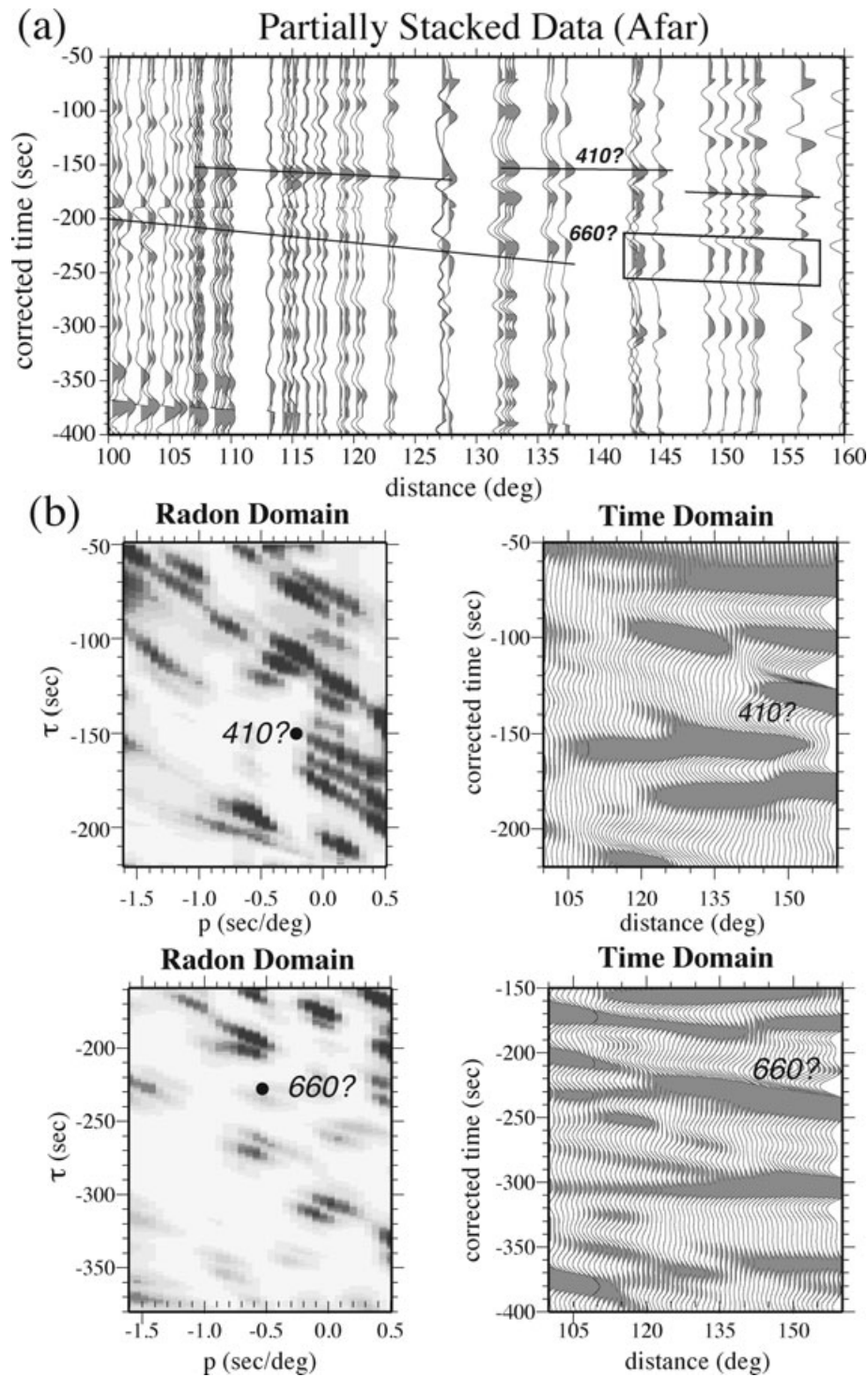
Figure 5. Time series and the corresponding Radon transform of the Afar hotpot. (a) The reflections (top panel) resulting from the 410 and 660 are strongly segmented and complex. The lines highlight the detectable phases within the data window. Waveforms contained in the box (142–156°) show the diminished S660S and, possibly, multiple arrivals. (b) Radon transform of the time series (left column, middle and bottom). The solid black circles mark the reference MTZ reflector positions (at 400 and 670 km, respectively) of PREM synthetic seismograms. Both S410S and S660S are missing from the Radon solution. The reconstructed time series (right column, middle and bottom) show substantial variations signal arrival times.
