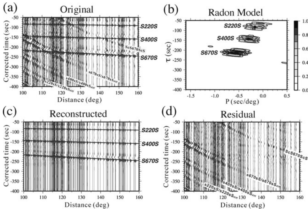
Figure 2. (a) PREM synthetic seismograms computed based on sample source–receiver pairs. These traces have been partially stacked (using a running average window of 20°) to enhance the signal-to-noise ratio. (b) Radon model obtained from the HRT method. The energy peaks result from underside reflections at 220-, 400- and 670-km depths. The contour lines mark the normalized amplitudes of 0.2, 0.4, 0.6 and 0.8; the maximum amplitude of the entire solution is set to 1. (c) Reconstructed time series based on the inverted Radon model. The main phases of interest are accurately predicted by the Radon solution. (d) Residual time series after subtracting the time series shown by (c) from (a). Both correlated (multiples) and random noise has been effectively eliminated.
