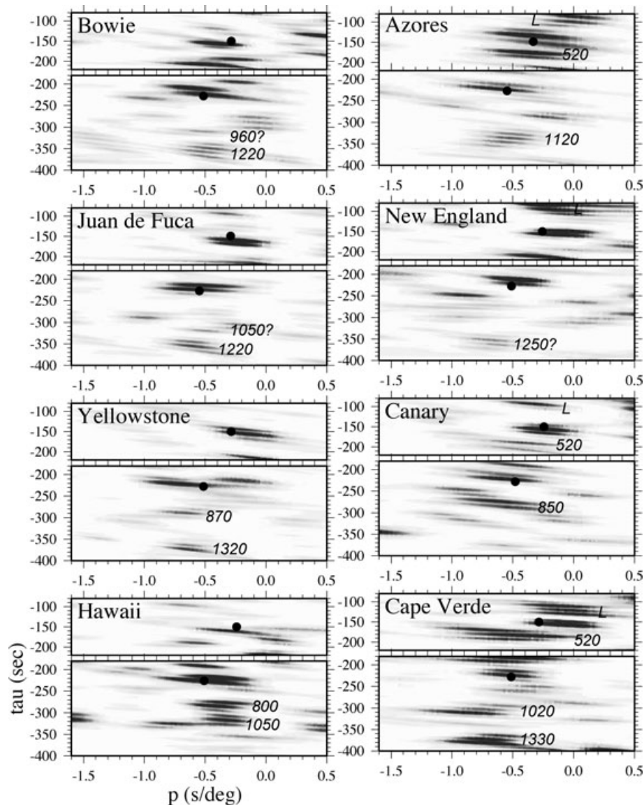
Figure 6. The radon image of eight hotspots in the Northern Hemisphere. The solid black circles mark the positions of measured MTZ peaks from PREM synthetic seismograms. The difference between observed and predicted Radon peaks reflect structural and dip differences (see main text). Most of these Radon images show robust energy peaks preceding the MTZ phases. Some of these signals are potentially caused by lower mantle reflectors at the depths that are indicated on the plot.
