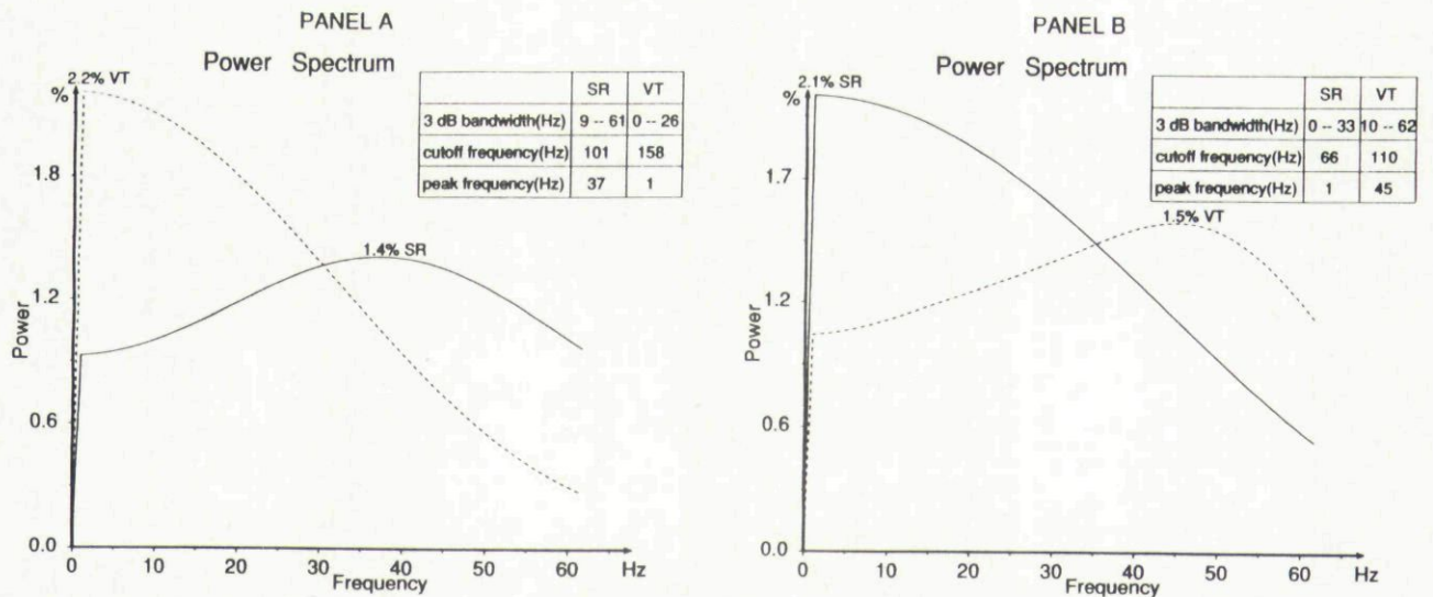
Figure 5. Typical power spectrum plots of ventricular depolarization during sinus rhythm and ventricular tachycardia from one patient (patient 4) without antiarrhythmic drug therapy (Panel A) and with antiarrhythmic drug therapy (Panel B). The peak frequency content of the depolarization waveform from each of the two rhythms has been plotted as a percent of the power. Identification of ventricular tachycardia has been based on the hypothesis that slower conduction (i.e. widened waveforms) during ventricular tachycardia result in a shift of peak frequency to a lower value than that observed during sinus rhythm. However, whereas sinus rhythm has a higher peak frequency than ventricular tachycardia in Panel A, the converse is observed in Panel B. No consistent pattern is present in the differences in bandwidths having 3 dB points as limits, or in the cutoff frequency, to distinguish sinus rhythm from ventricular tachycardia.
