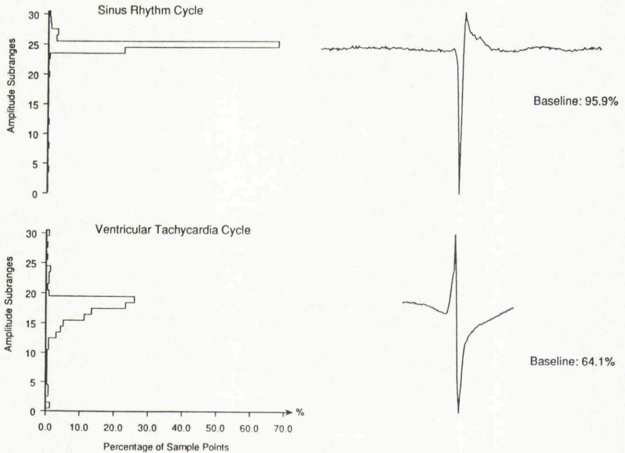
Figure 4. Examples of success (Panel A) and failure (Panel B) in identifying ventricular tachycardia by amplitude distribution analysis in individual patients. An amplitude histogram of a cardiac cycle with its associated ventricular electrogram during sinus rhythm is shown in the upper half, and an amplitude histogram of a cardiac cycle during ventricular tachycardia with its associated ventricular electrogram during subsequently induced ventricular tachycardia is shown in the lower half of each panel. The peak-to-peak amplitude range of the cardiac cycle has been divided into 30 subranges and temporal normalization was performed by dividing by the number of sample points in each subrange by the total number of sample points within the cardiac cycle. The percentage of sample points falling within each subrange has then been plotted on a histogram. Determination of the baseline percentage of sample points on, or near, the isoelectric baseline has been made from the 5 subranges centered on the most populated subrange. During sinus rhythm, 95.9% of all amplitude points fall within the baseline region while only 64.1% fall within the baseline region during ventricular tachycardia. In Panel A (patient 8), the baseline percentage of sample points during ventricular tachycardia was significantly less than the baseline percentage during sinus rhythm, thus successfully identifying ventricular tachycardia. In Panel B (patient 10 during antiarrhythmic drug therapy), the opposite occurred, preventing successful detection of ventricular tachycardia by amplitude distribution analysis.
