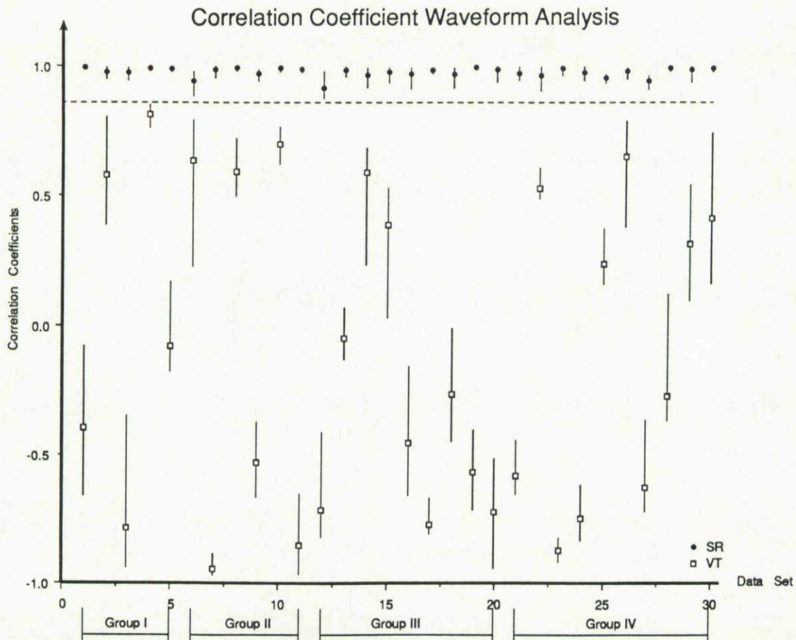
Figure 2. Results of correlation waveform analysis of the 30 paired data sets of sinus rhythm (SR) and ventricular tachycardia (VT). Solid circles are average values and vertical bars represent the range of correlation coefficients for each patient during sinus rhythm. Open squares are average values and the vertical bars represent the range of correlation coefficients during ventricular tachycardia. Each paired set is aligned vertically. The dotted line represents a decision boundary (between 0.855 and 0.874) which separates sinus rhythm from ventricular tachycardia with 100% accuracy. Groups I-IV are defined in the text.
