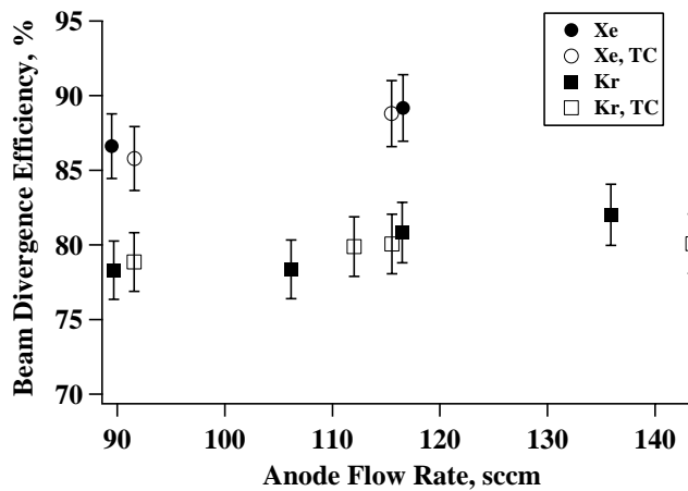
Figure 12. Beam Divergence Efficiency versus Anode Flow Rate
