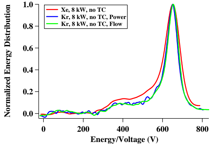
Figure 7. Voltage Energy Distribution Comparison for Xenon and Krypton at 8 kW without the Trim Coil
