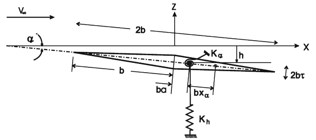
Fig. 5 Two-degree-of-freedom typical airfoil geometry.
