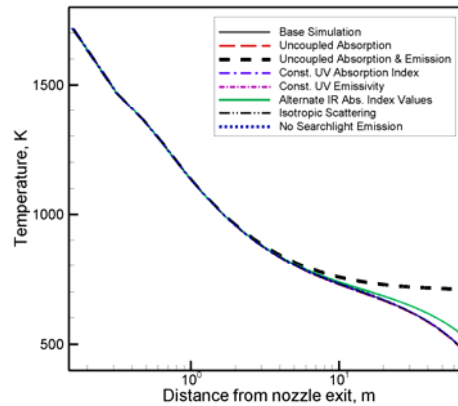
Fig. 12 Temperature of 0.4 \mu\text{m} particles along the extraction line.
