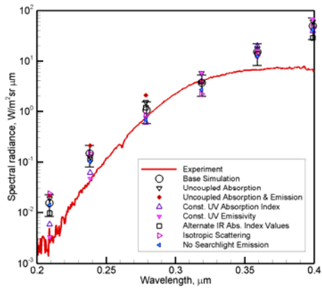
Fig. 15 Dependence of UV spectral radiance on radiation model parameters.
