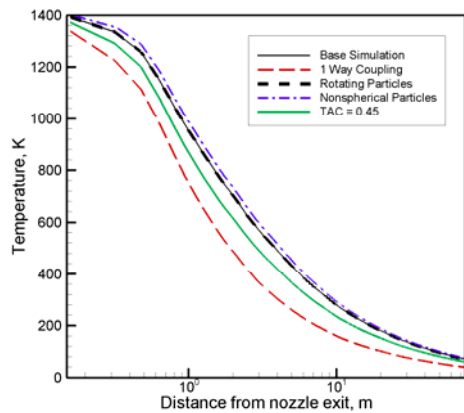
Fig. 7 Gas translational temperature along the extraction line.
