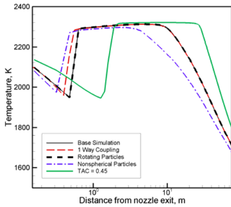
Fig. 9 Temperature variation along the extraction line for 4 \mu\text{m} particles.
