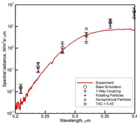
Fig. 11 UV spectral radiance at the onboard sensor.
