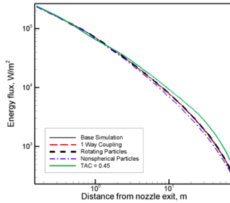
Fig. 10 Net radiative energy flux along the extraction line.
