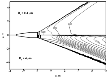
Fig. 3 Close-up view of particle temperature contours. Values are given in K.
