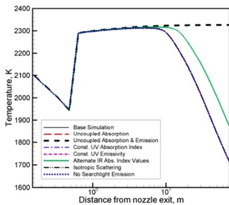
Fig. 13 Temperature of 4 \mu\text{m} particles along the extraction line.
