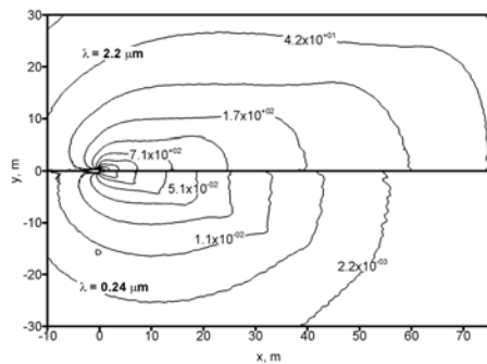
Fig. 5 Contours of the direction-averaged spectral energy flux at wavelengths of 2.2 \mu\text{m} and 0.24 \mu\text{m} . Values are in \text{W}/\text{m}^2\mu\text{m} .
