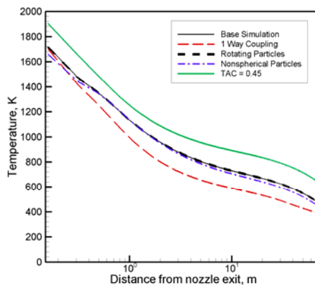
Fig. 8 Temperature variation along the extraction line for 0.4 \mu\text{m} particles.
