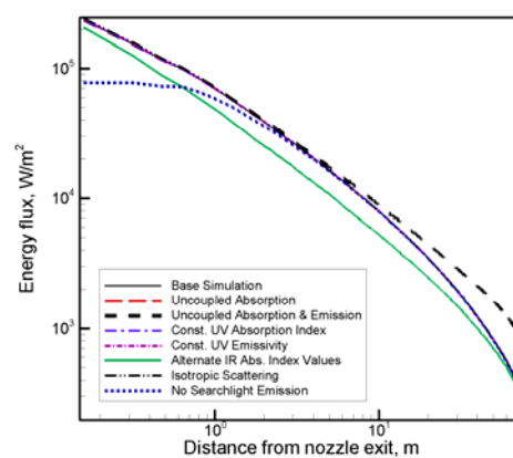
Fig. 14 Variation along the extraction line in the net direction-averaged radiative energy flux.
