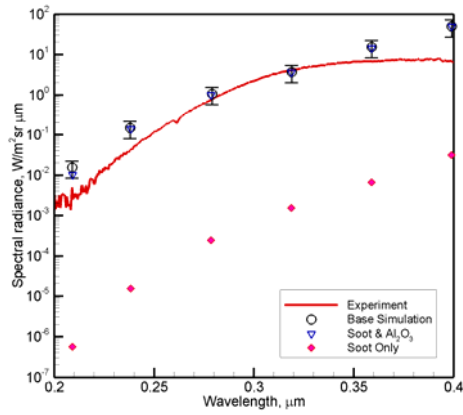
Fig. 17 Effect of soot on UV radiance at the onboard sensor.
