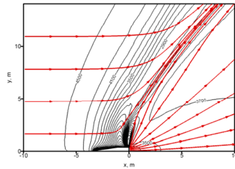
Fig. 2 Gas streamlines and contours of bulk velocity magnitude. Contour line values are given in m/s.
