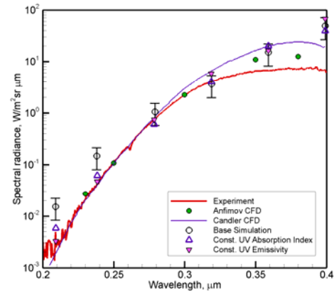
Fig. 6 UV spectral radiance measured at the onboard sensor.
