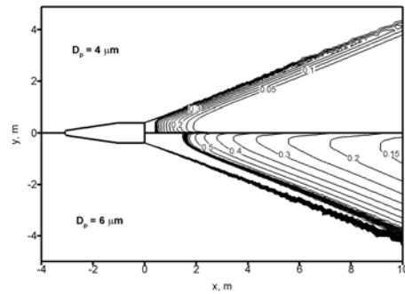
Fig. 4 Contours of liquid mass fraction for 4 and 6 \mu\text{m} diameter particles.
