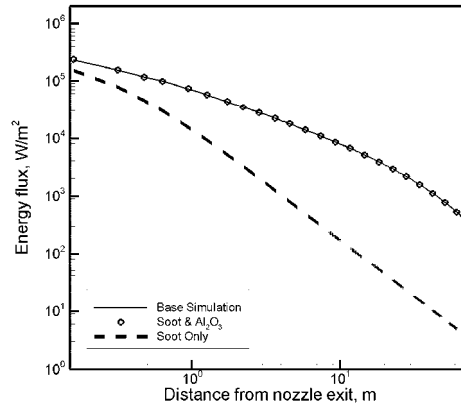
Fig. 16 Effect of soot on the net radiative energy flux along the extraction line.
