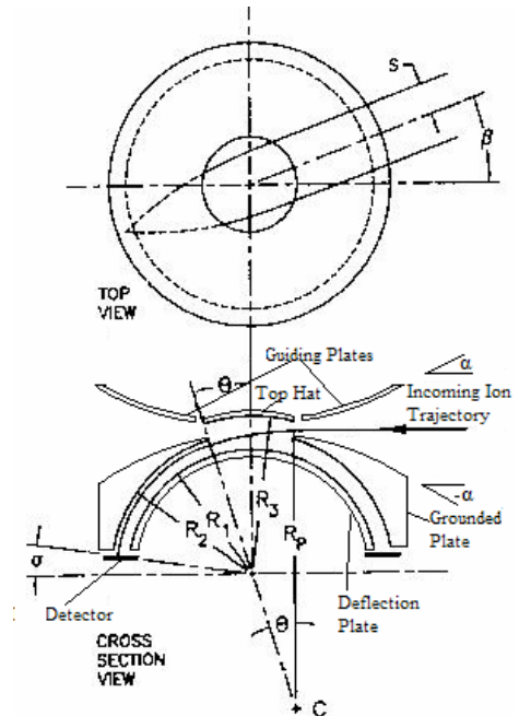
Figure 2. Principal design parameters of a top hat analyzer. 12
