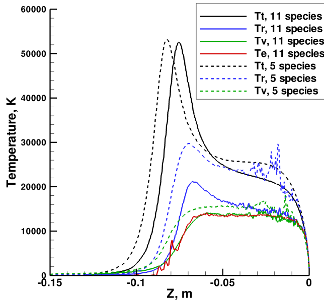
Figure 3.6: Temperatures along the stagnation streamline for both the 11 species and 5 species cases, FIRE II at 76 km.
