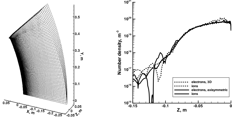
(a) Computational grid used for the 3D simulation. (b) Charged species number densities along the stagnation streamline of both the 3D and axisymmetric fore body solutions.
