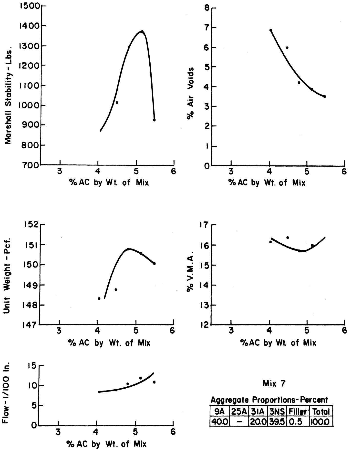
Figure 13 Marshall Data for Mix 7 with Natural Coarse Aggregate
