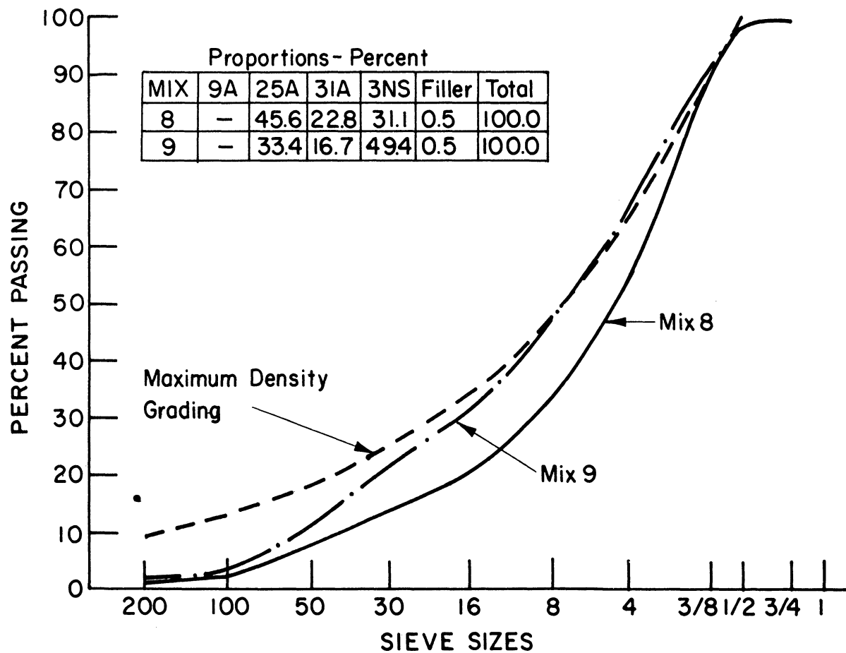
Figure 6 Aggregate Grading for Mix 8 and 9
