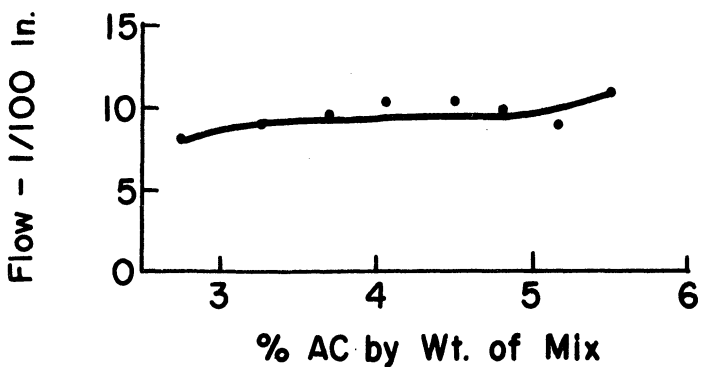
Figure 7 Marshall Data for Mix 1 with Natural Coarse Aggregate
