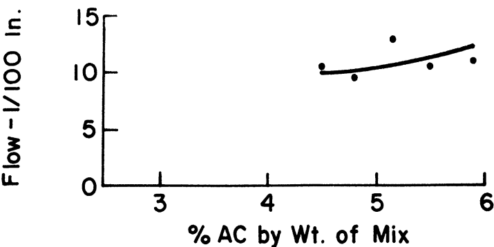
Figure 10 Marshall Data for Mix 4 with Natural Coarse Aggregate
