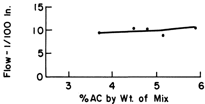
Figure 15 Marshall Data for Mix 9 with Natural Coarse Aggregate
