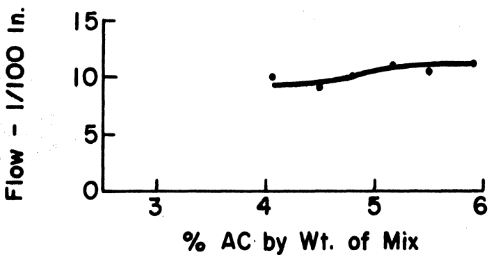
Figure 12 Marshall Data for Mix 6 with Natural Coarse Aggregate
