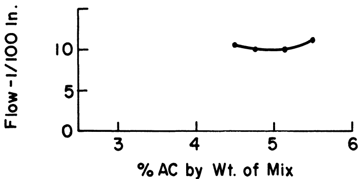
Figure 17 Marshall Data for Mix 4 with Crushed Dolomite Coarse Aggregate
