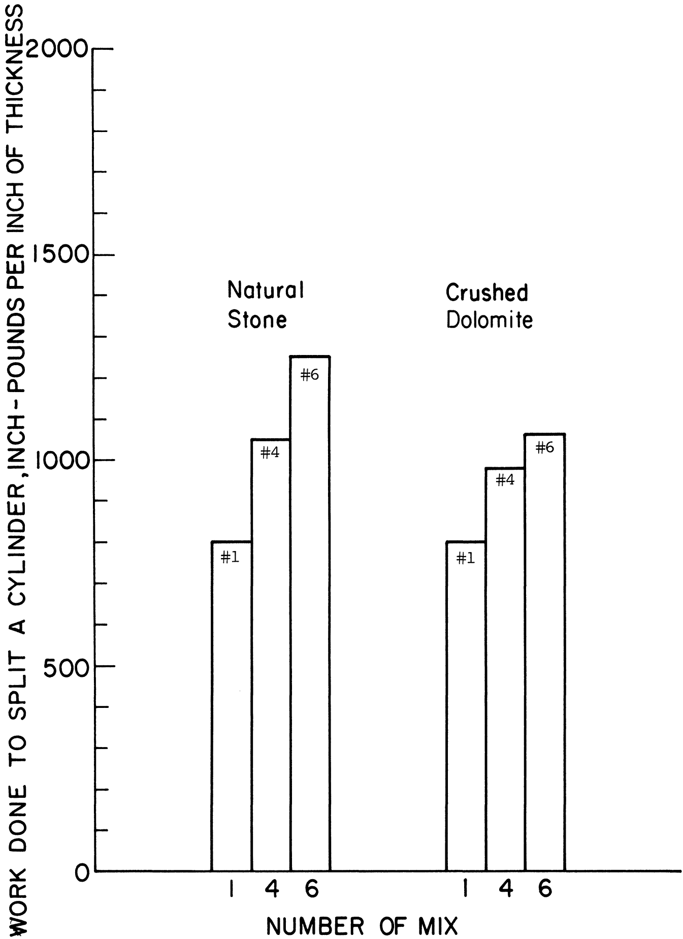
Figure 20 Comparisons of Work Necessary to Split Cylinders Made Out of Various Mixes
