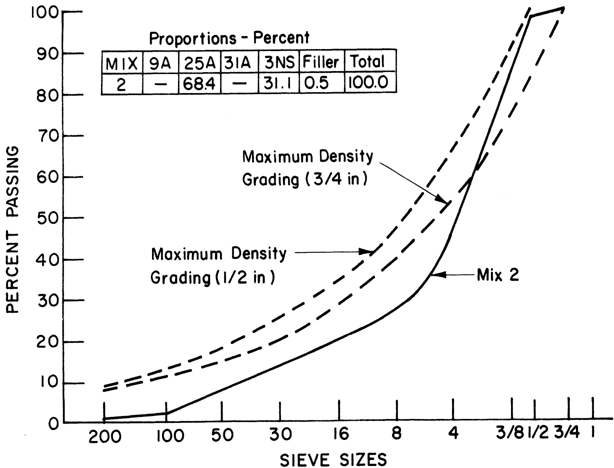
Figure 2 Aggregate Grading for Mix 2
