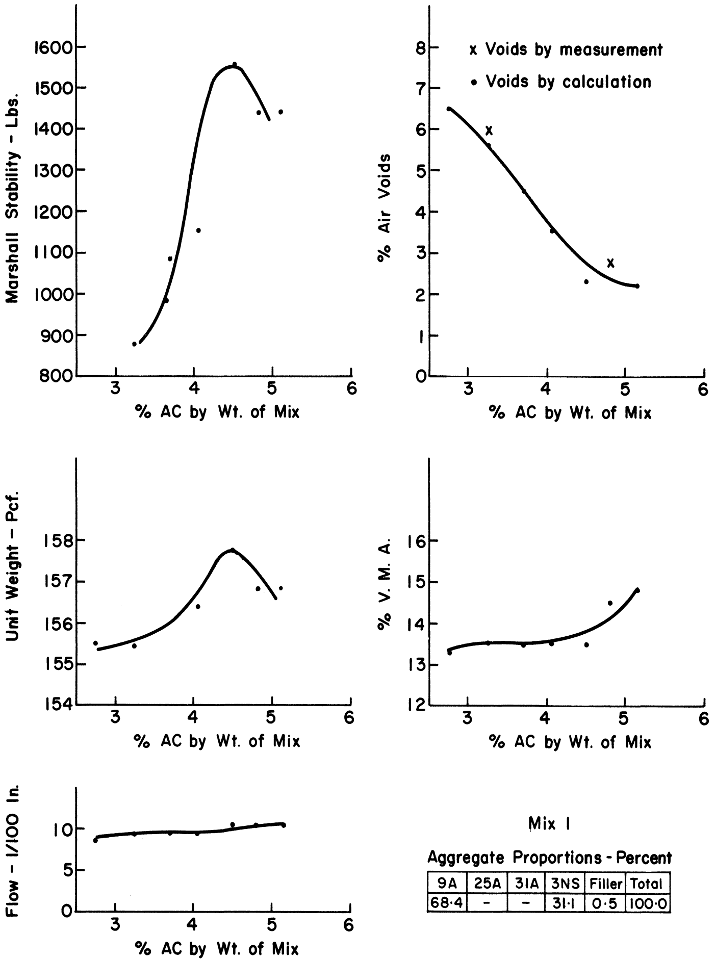
Figure 16 Marshall Data for Mix 1 with Crushed Dolomite Coarse Aggregate
