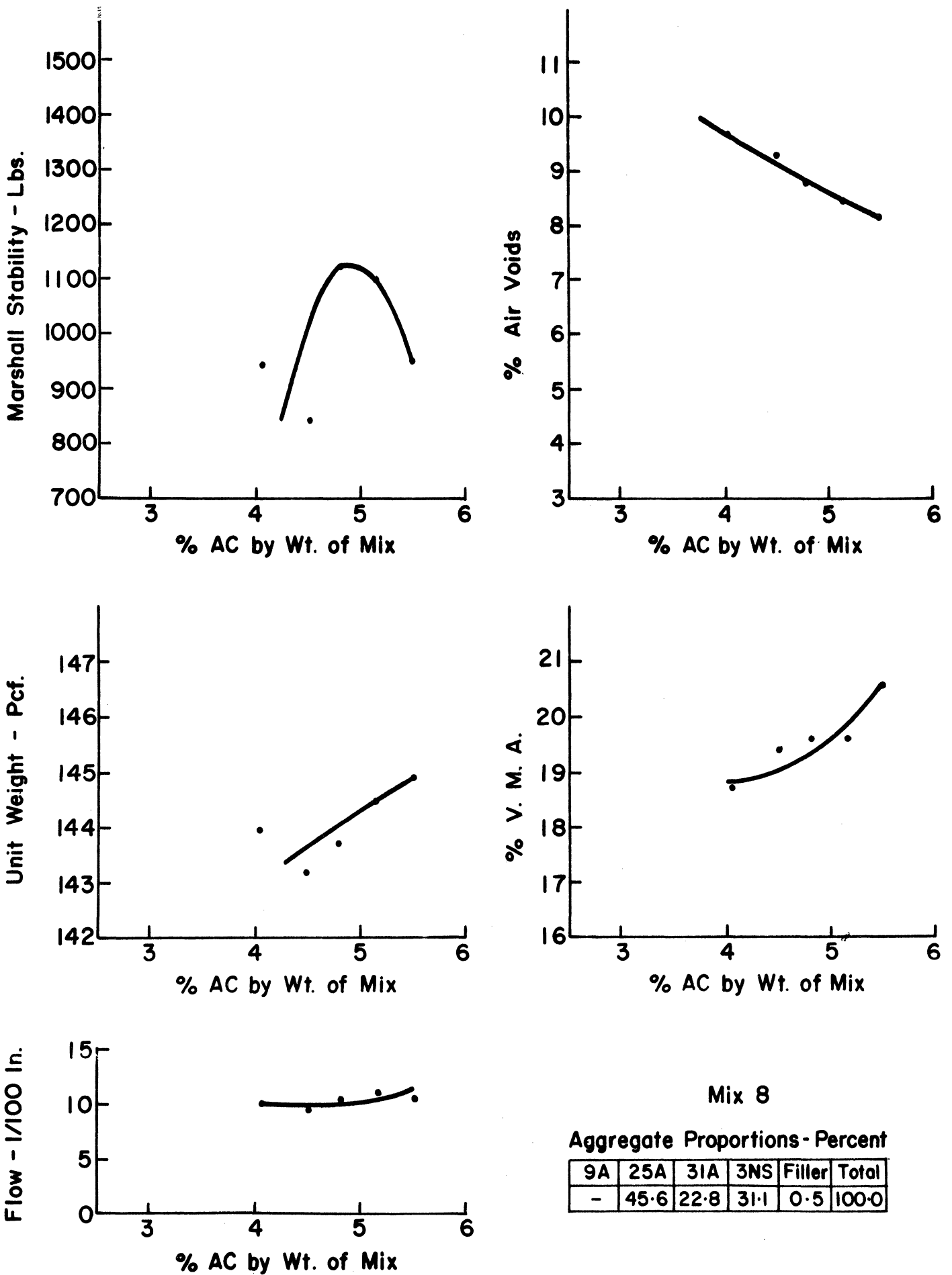
Figure 14 Marshall Data for Mix 8 with Natural Coarse Aggregate
