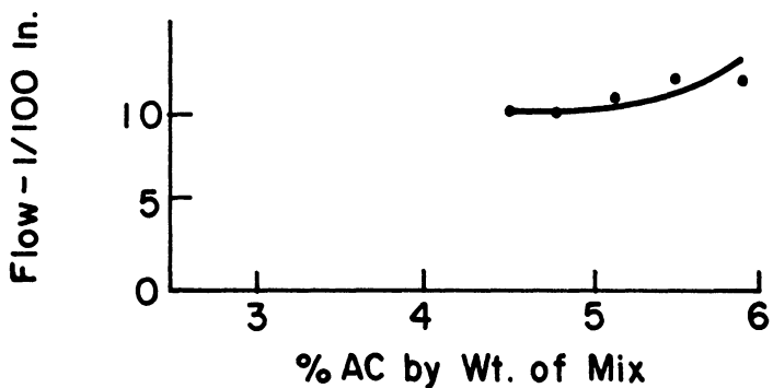
Figure 18 Marshall Data for Mix 6 with Crushed Dolomite Coarse Aggregate
