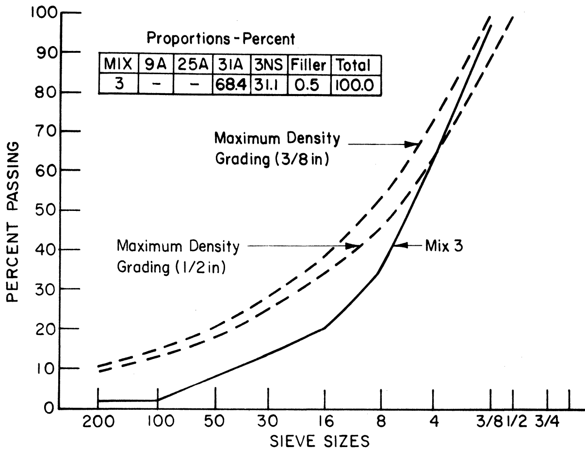
Figure 3 Aggregate Grading for Mix 3
