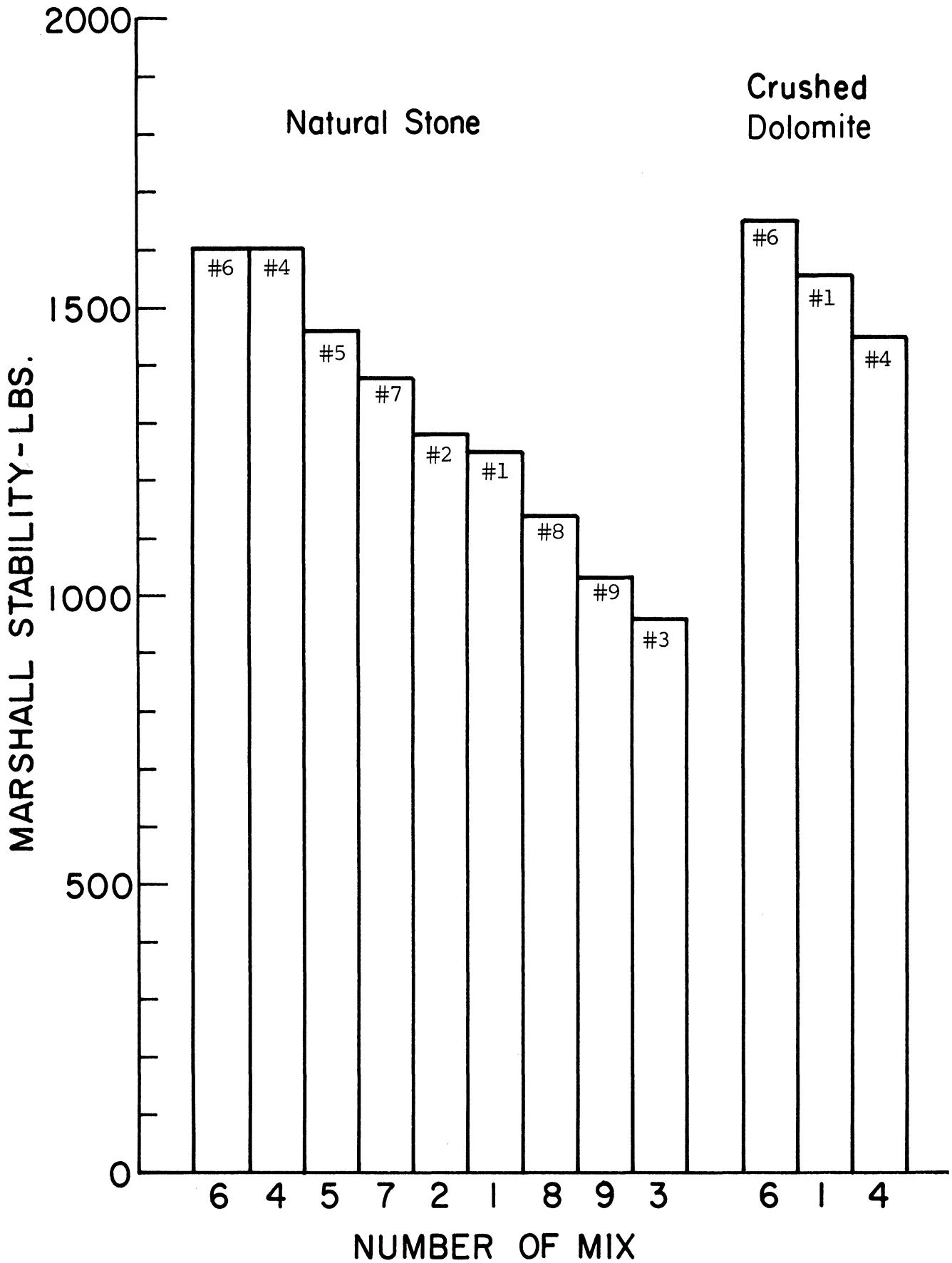
Figure 19 Peak Marshall Stability Attained for Each Mix at Asphalt Content Above 4.5%
