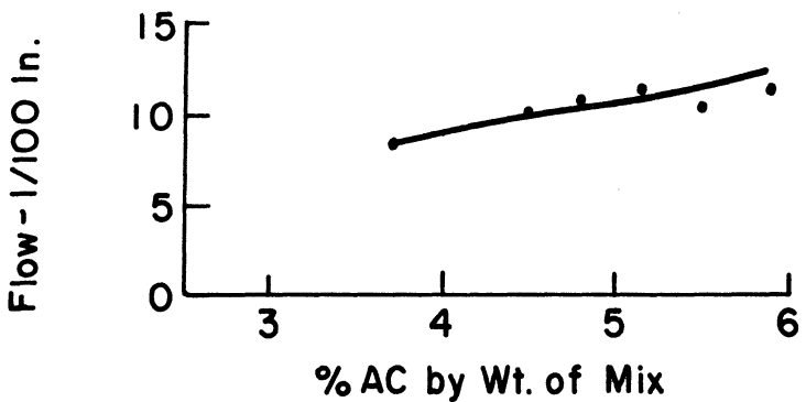
Figure 11 Marshall Data for Mix 5 with Natural Coarse Aggregate
