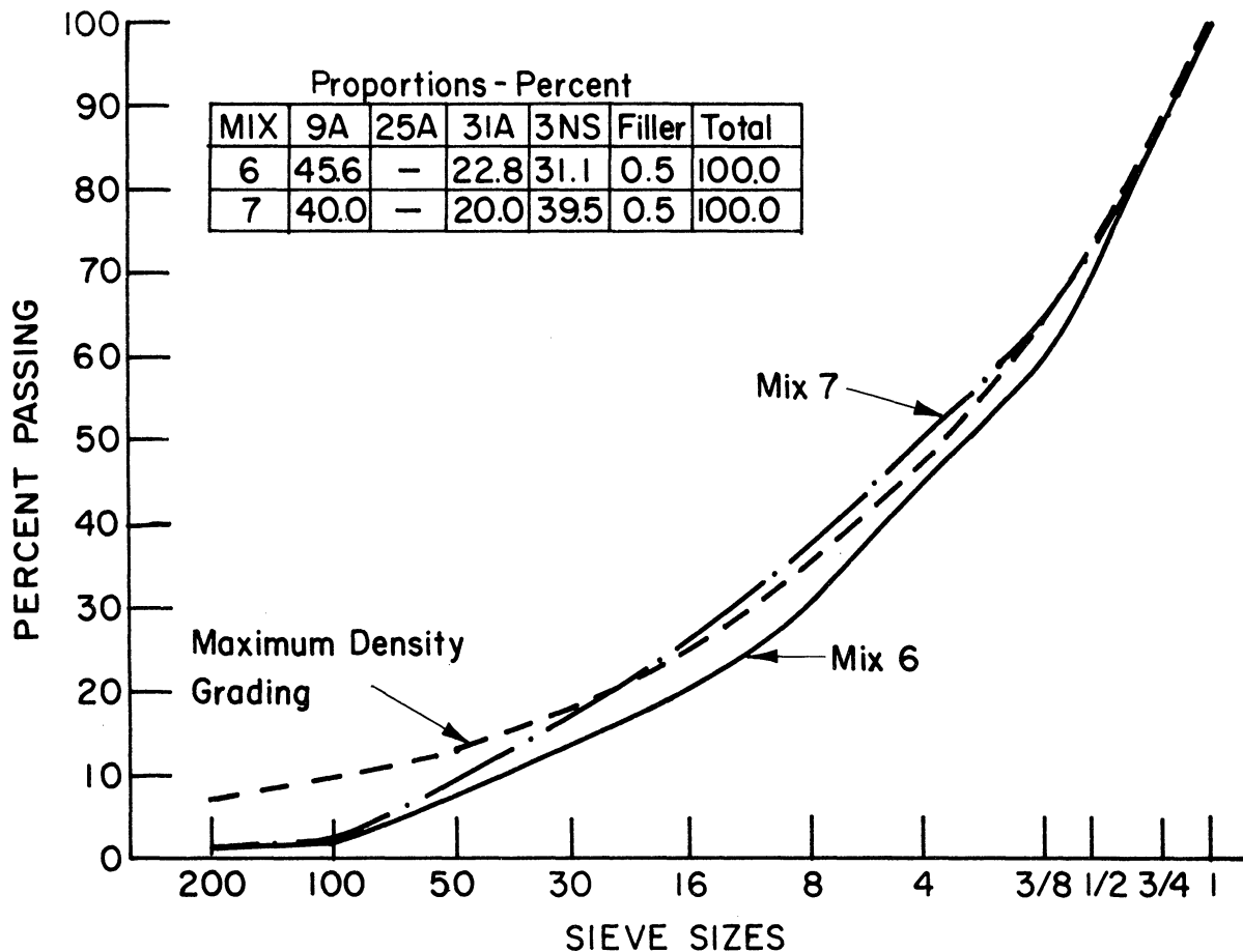
Figure 5 Aggregate Grading for Mix 6 and 7
