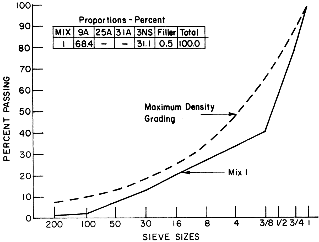
Figure 1 Aggregate Grading for Mix 1
