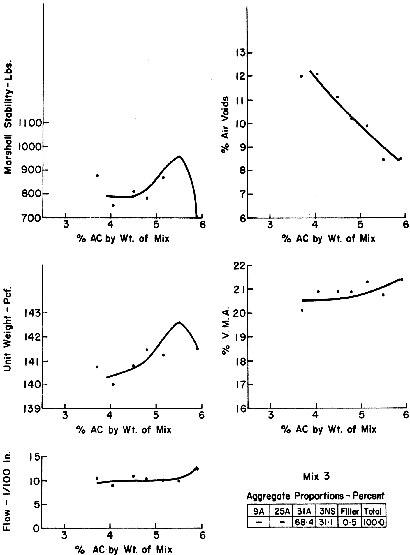
Figure 9 Marshall Data for Mix 3 with Natural Coarse Aggregate
