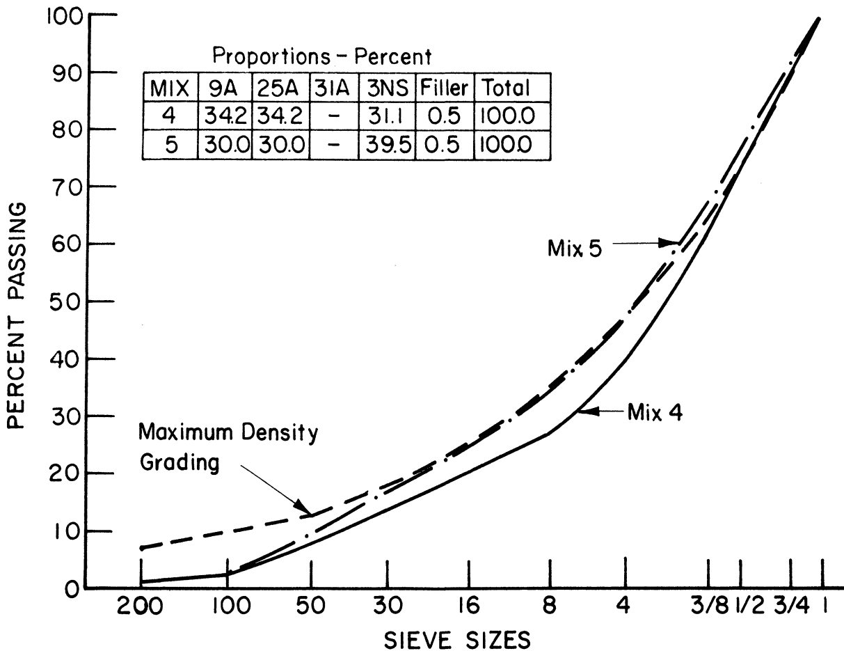
Figure 4 Aggregate Grading for Mix 4 and 5
