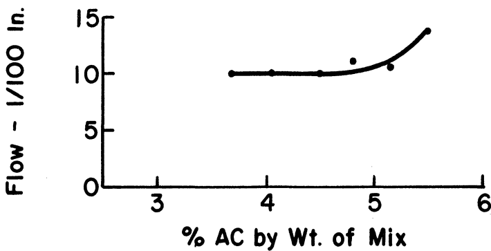
Figure 8 Marshall Data for Mix 2 with Natural Coarse Aggregate
